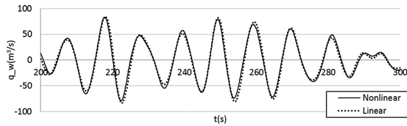
FIG. 19. Flowrates driven by the IWS for linear and nonlinear PTOs: H_s = 2 m and T_p = 10 s.
