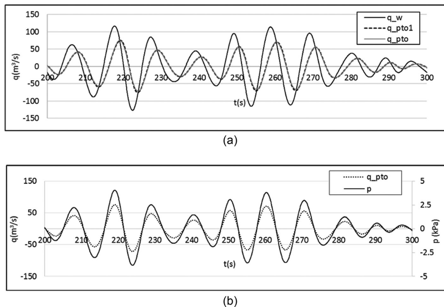
FIG. 11. A comparison of the flowrates through the PTO (“ q_{pto} ” by Eq. (8) and “ q_{pto1} ” by Eq. (9)) and the flowrate driven by the IWS (Eq. (7)). V_r = 5.0 , H_s = 2.0 m, and T_p = 10 s, K_1 = 52.48 N s/m 5 , P_{av} = 65.25 kW (floating). (a) Comparison of flowrates and (b) flowrate and chamber pressure.
