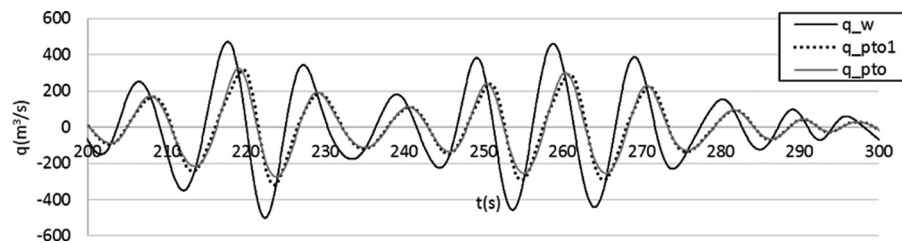
FIG. 13. A comparison of the flowrates through the PTO (“q_pto” by Eq. (8) and “q_pto1” by Eq. (9)) and the flowrate driven by the IWS (Eq. (7)). V_r = 5.0 , H_s = 8.0 m, and T_p = 10 s, K_1 = 52.48 N s/m 5 , P_{av} = 1049.1 kW (floating).
