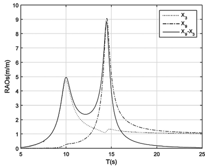
FIG. 2. Heave RAOs of the structure ( X_3 ) and the water body ( X_9 ) and their relative motion RAO ( X_9-X_3 ), with additional damping coefficients: B_{33} = 200 \text{ kN s/m} and B_{99} = 100 \text{ kN s/m} .
