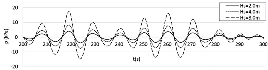
FIG. 16. T_p = 10 s, V_r = 5.0 , and K_1 = 52.48 N s/m 5 .
