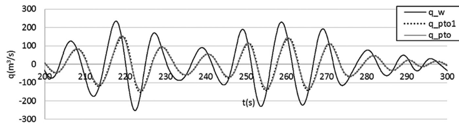
FIG. 12. A comparison of the flowrates through the PTO (“q_pto” by Eq. (8) and “q_pto1” by Eq. (9)) and the flowrate driven by the IWS (Eq. (7)). V_r = 5.0 , H_s = 4.0 m and T_p = 10 s, K_1 = 52.48 N s/m 5 , P_{av} = 261.26 kW (floating).
