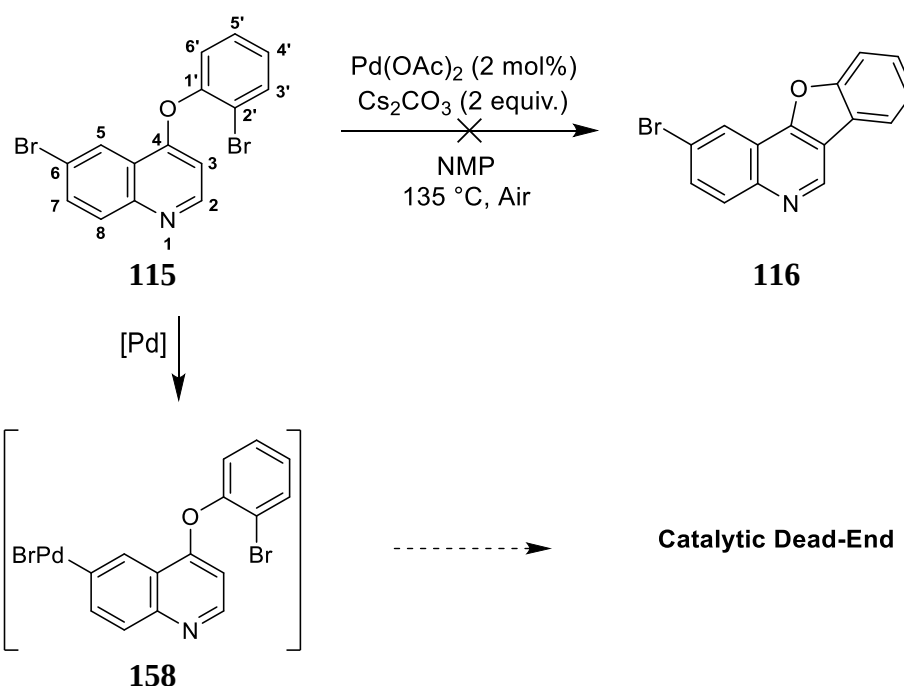
Scheme 78 Irreversible oxidative addition of the catalyst into the C-6 C-Br bond of 115 causes the catalytic cycle to reach a dead-end in the absence of an intermolecular coupling partner.
