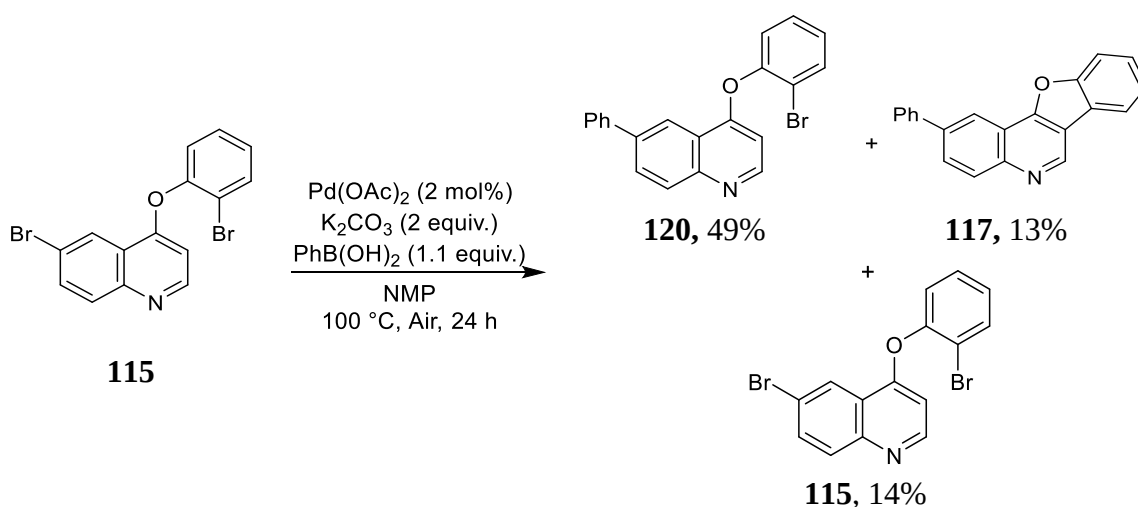
Scheme 59 Tandem reaction carried out at 100^\circ\text{C} . Yields are isolated yields.
