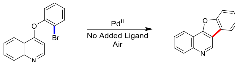
Figure 24 Palladium-catalysed C-H activation at the C-3 position of quinolines.
