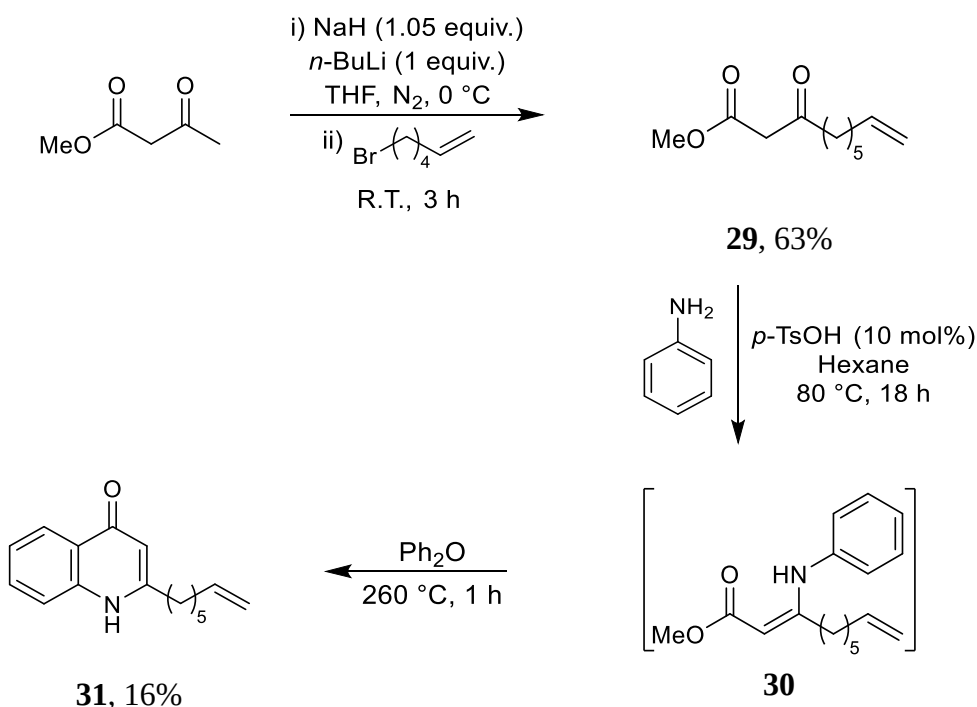
Scheme 10 Synthesis of HHQ analogue 31 with a terminal alkene.
