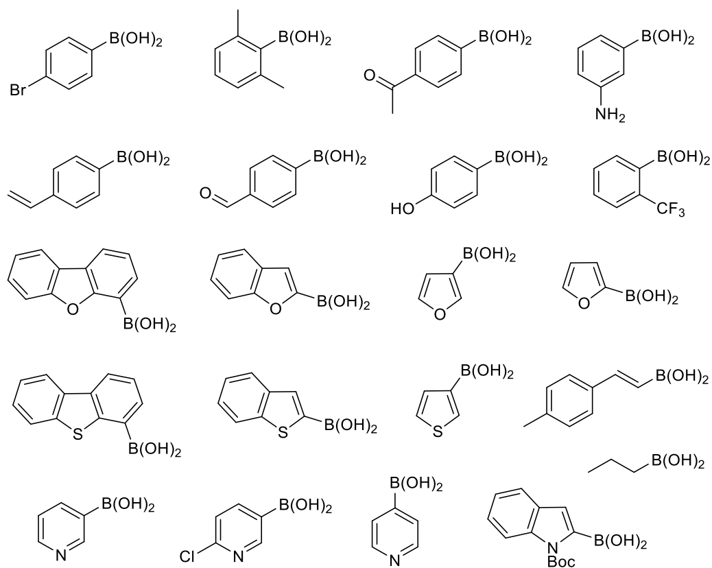
Figure 28 Boronic acids that were not compatible with the tandem reaction.
