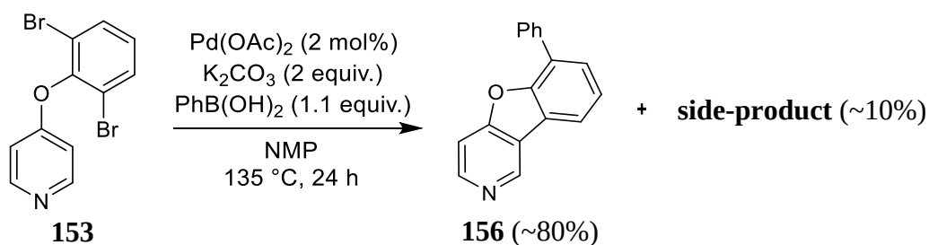
Scheme 76 Tandem reaction of substrate 153 .
