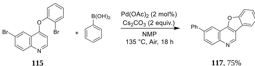
Scheme 57 Tandem Suzuki-Miyaura and direct arylation of 115 .
