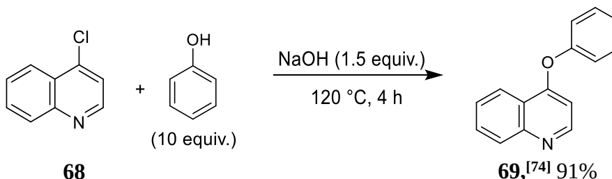
Scheme 45 Synthesis of 4-phenoxyquinoline 69 .
