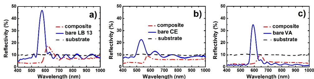
Fig. 3. The optical reflectivity spectra of colloidal crystal photonic multilayers (a) 13-layer LB multilayer of 250 nm silica particles, (b) controlled evaporation (see Ref. 10) multilayer of 235 nm silica particles and (c) vertical assembly grown multilayer of 265 nm polystyrene particles in comparison with the spectra of freestanding composite films of the original films in PVA.
