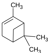
Figure 4.1 Structure of \alpha -pinene.
