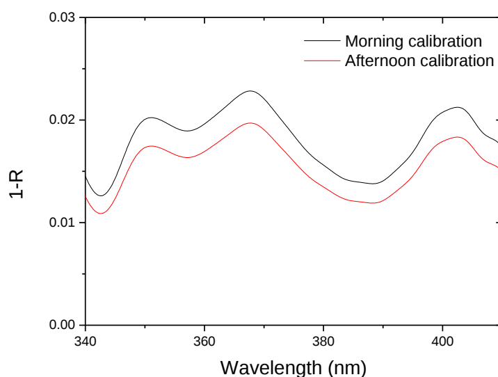
Figure 2.16 Mirror reflectivity spectra based on calibrations prior to (black) and after (red) an experiment in which SOA was formed. The shape of the reflectivity spectrum is the same for the morning and afternoon, with a 15% difference in the magnitude in the (1 - R) values.
