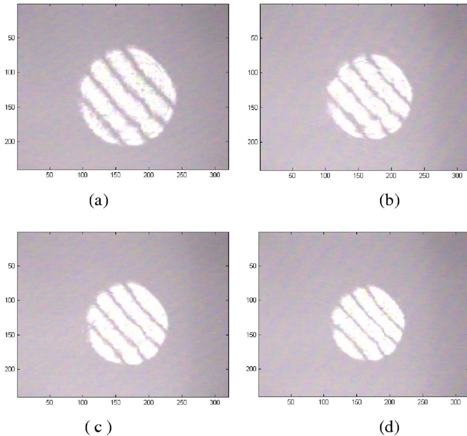
Fig. 8 Optical images I_i(x,y) produced by the SiC-chip-based pressure system for (a) 0 atm, (b) 13.6 atm (200 psi), (c) 27.2 atm (400 psi), and (d) 40.8 atm (600 psi) high differential pressure conditions in the pressure capsule. Dimensions on both axes are in CCD pixels.
