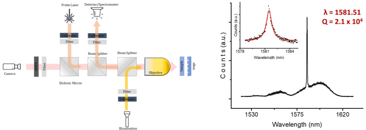
Figure 1. a) Schematic of Resonant Scattering experimental set up b) Resonant spectra of a PhC L3 cavity
