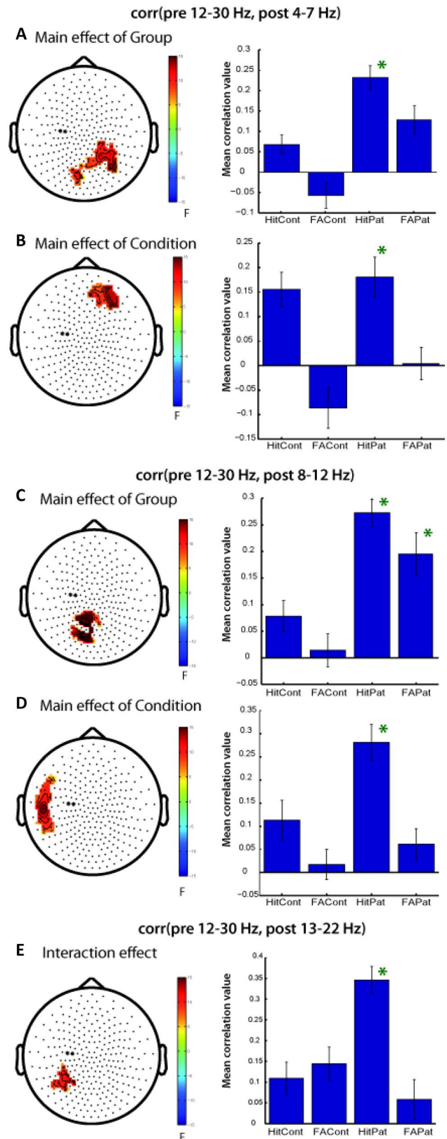
Fig. 6 Correlation between pre-stimulus beta and post response power. Beta (12–30 Hz) power in the pre-stimulus interval (–0.5 s to stimulus onset) of two centro-parietal sensors (marked with black asterisks on the topographies) was correlated with post response power (0–0.5 s after response) in all other sensors on a trial by trial basis. Left: topographies of results of 1-within-1-between permutation ANOVA on correlation values, n = 26 , only significant clusters are depicted). Right: mean correlation values over significant channels. Green asterisks indicate also a significant one-sample t-test over the channels in the significant cluster. HitCont hits controls, HitPat hits patients, FACont false alarms Controls, FAPat false alarms patients; a, b Correlation of pre-stimulus beta power with post-response theta power (4–7 Hz). c, d Correlation of pre-stimulus beta power with post-response alpha power (8–12 Hz). e Correlation of pre-stimulus beta power with post-response beta power (13–22 Hz)
