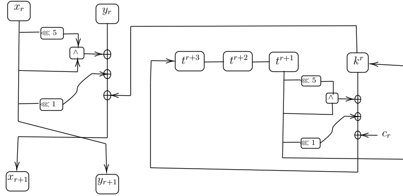
Figure 4.2: Simeck cipher
