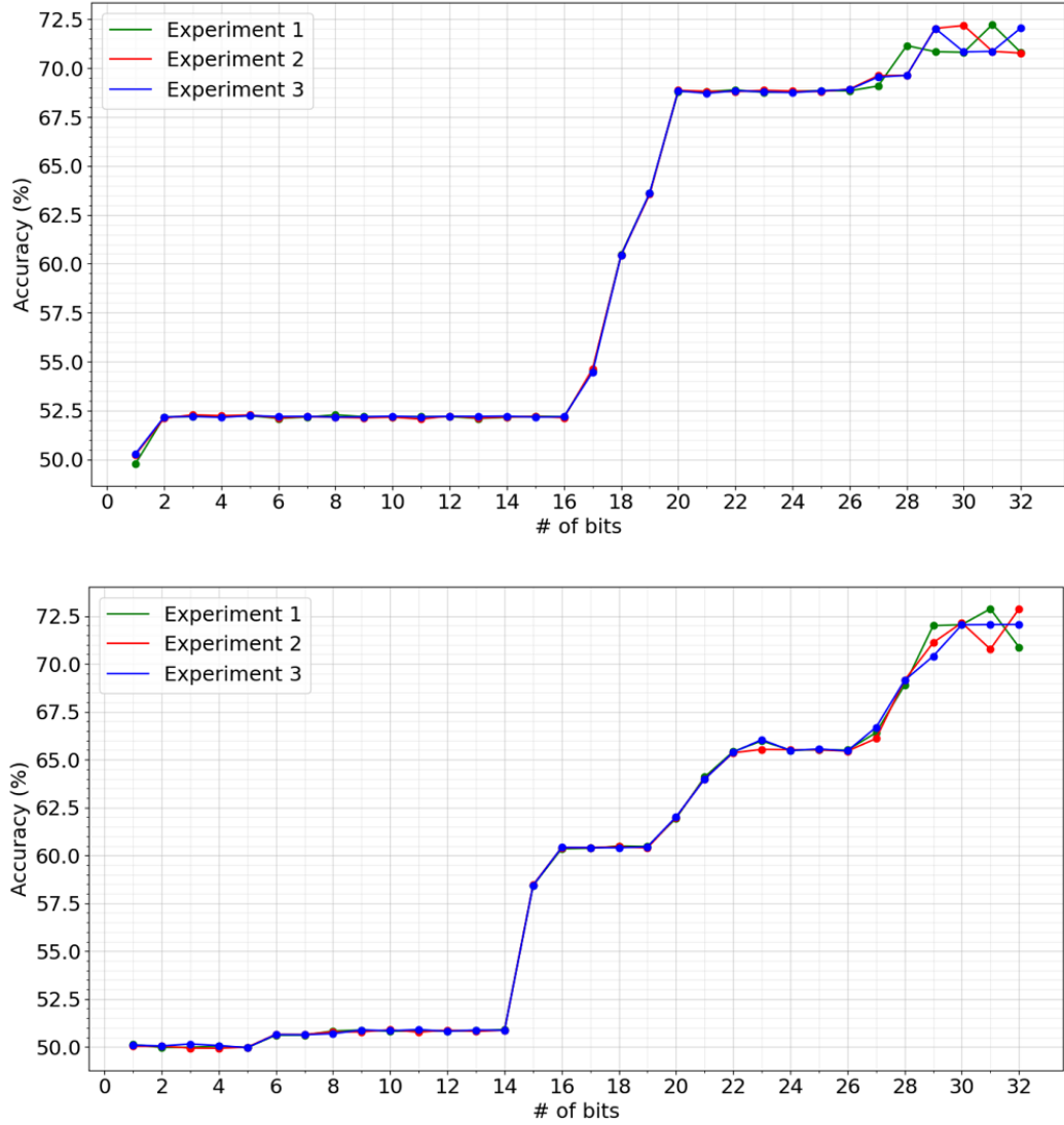
Figure 3.2: Accuracy of ML-based distinguishers according to number of bits in MSB→LSB direction for 6 rounds of SPECK32/64
