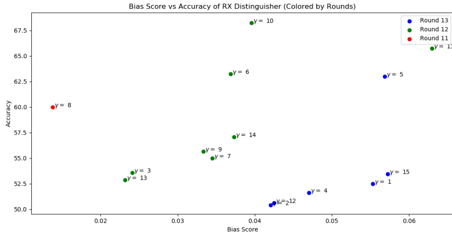
Figure 4.3: Scatter plot of Bias Score vs Accuracy of RX Distinguisher (Colored by Rounds)
