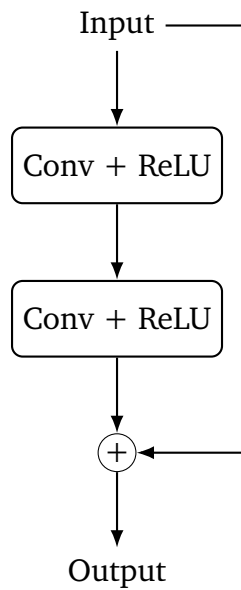
Figure 2.3: Overview of ResNet Layer
