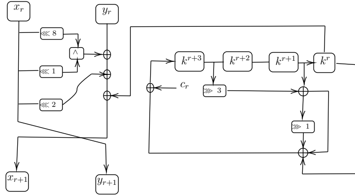
Figure 4.1: Simon cipher for m = 4
