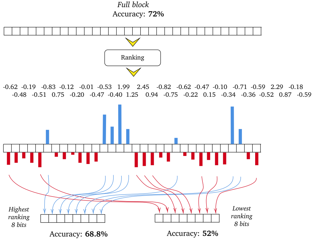
Figure 3.4: The Training Process of PD-ML distinguishers. Rank values are as per Table 3.1. Plotted bars are approximation of the values (due to graphical constraints).
