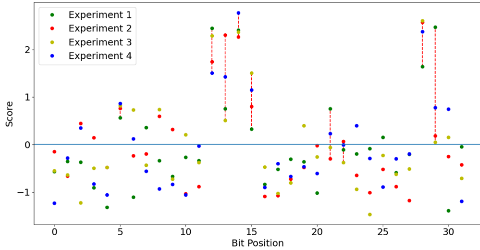
Figure 3.3: Normalized Scores for 4 different combination sets. The bits with vertical lines are the ones that are chosen as the most effective bits for training a PD-ML-based distinguisher for six rounds of SPECK32/64.
