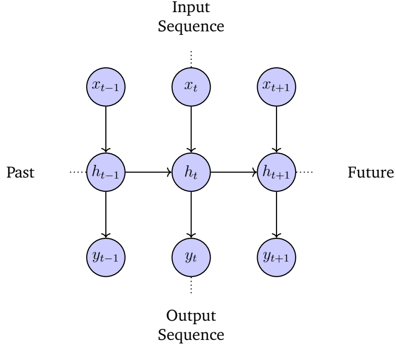
Figure 2.4: Overview of RNN Layer
