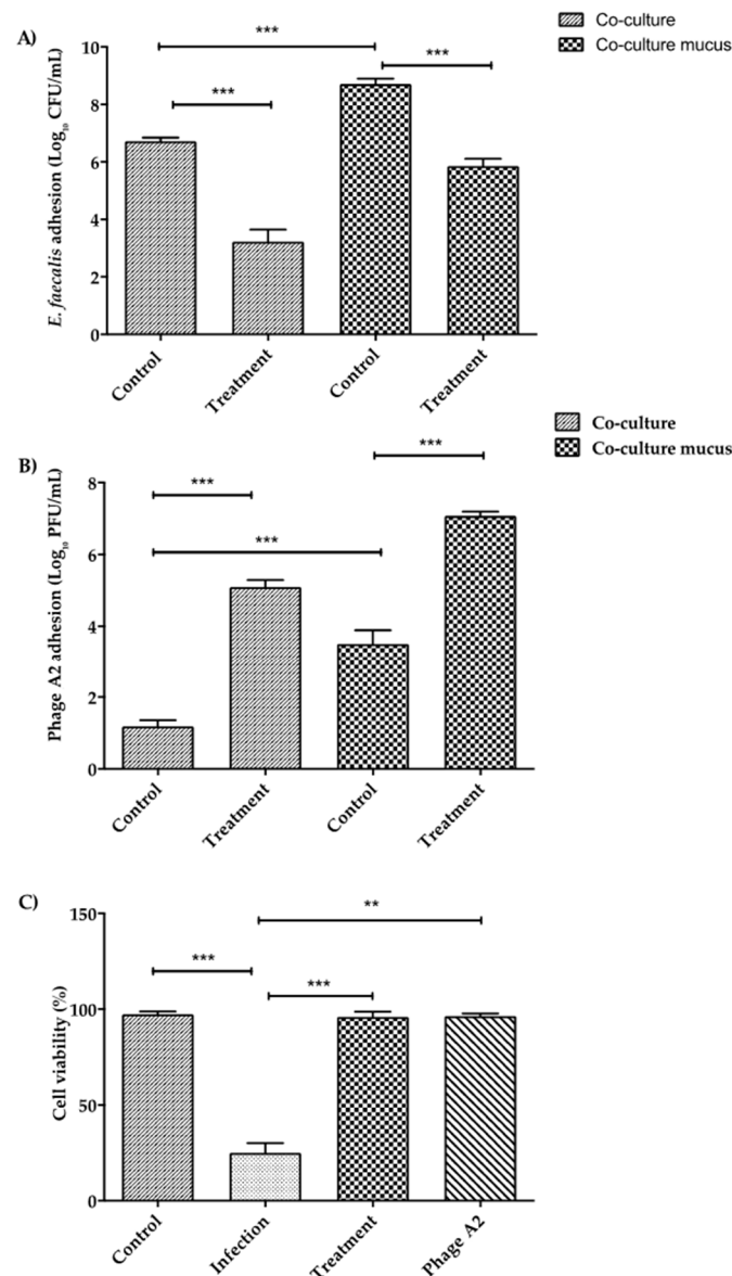
Figure 5. (A) Enterococcus phage A2 and adhered E. faecalis interaction in a co-culture mimicking the intestinal epithelium with and without mucus. E. faecalis was left to adhere to the co-cultures for 3 h. At this point, fresh media was added and the treatment ( E. faecalis + phage A2) groups were inoculated with phage A2. (B) Enterococcus phage A2 adherence to a co-culture with and without the presence of mucus. Control groups were co-cultures only inoculated with phage. The treatment groups were infected with E. faecalis for 3 h and then treated with phage. All the samples were collected at 24 h post-inoculation. (C) Cell survival of co-culture producing mucus following 24 h. of exposure to E. faecalis and Enterococcus phage A2. Cell survival following each exposure is shown in comparison to a control co-culture without bacteria and phage. All values are average concentrations ( n = 9 ) \pm standard error. ** p < 0.01 ; *** p < 0.001 .
