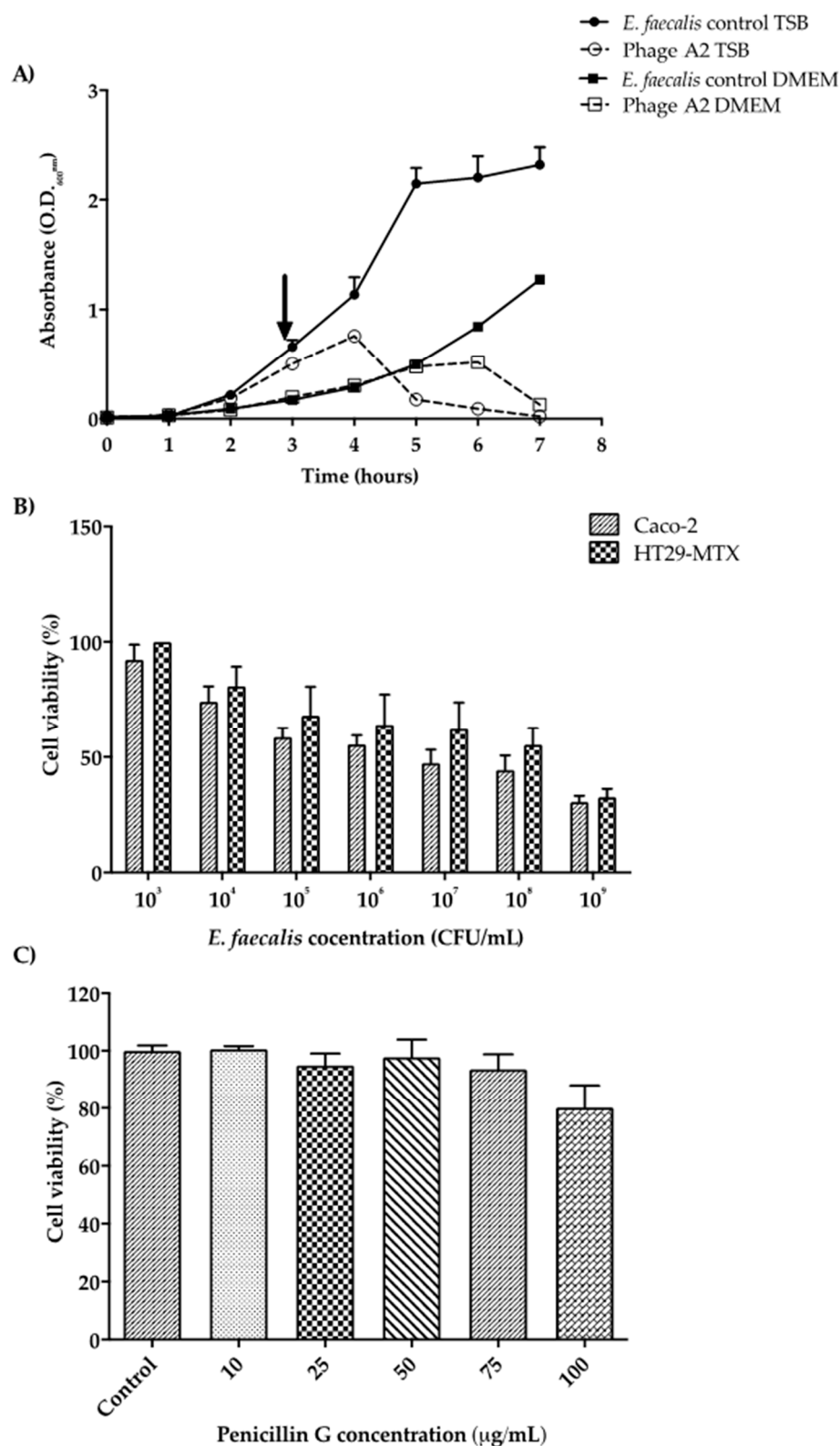
Figure 4. (A) Enterococcus phage A2 infectivity and E. faecalis growth in TSB broth and DMEM cell culture media. Results show average values ( n = 3 ) \pm standard error (arrow indicates timepoint which phage A2 was introduced to culture). (B) Caco-2 and HT29-MTX cell viability following infection of E. faecalis at varying concentrations. The cells were exposed to E. faecalis for 24 h before measuring survival rates. Columns show average cell viability in percentage ( n = 6 ) \pm standard error. (C) Caco-2 and HT29-MTX co-culture viability at varying penicillin G concentrations. Columns show average cell viability in percentage ( n = 3 ) \pm standard error.
