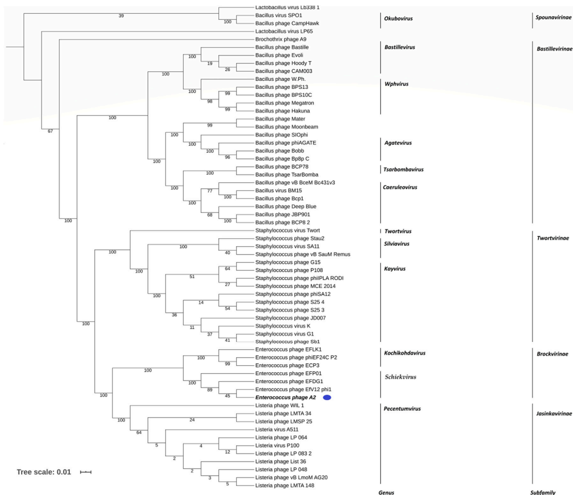
Figure 3. Amino acid based VICTOR-generated phylogenomic Genome-BLAST Distance Phylogeny (GBDP) tree of Enterococcus phages A2 (highlighted with a blue dot), EfV12-phi, and EFP01 with 58 members of the Herelleviridae family Inferred using the formula D4 and yielding average support of 69%. The numbers below branches are GBDP pseudo-bootstrap support values from 100 replications.
