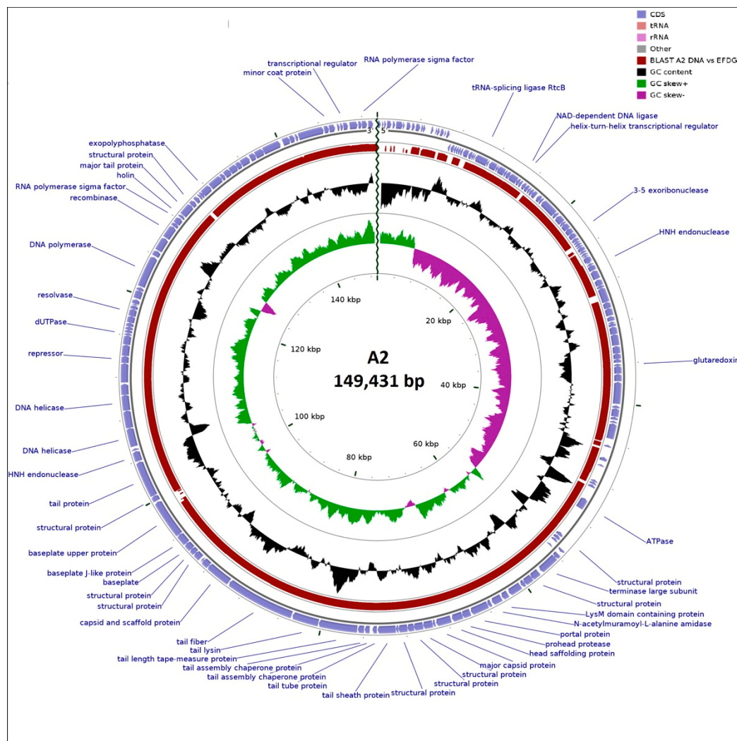
Figure 2. Summary of the genomic organization of Enterococcus phage A2. The outer ring shows putative ORFs, represented by purple arrowheads labelled with a predicted function where possible. The following inner ring shows a TBLASTX comparison (in red, where homologous) to Enterococcus phage EFDG1. GC content is depicted in black, while positive and negative GC skew is denoted by green and purple, respectively.
