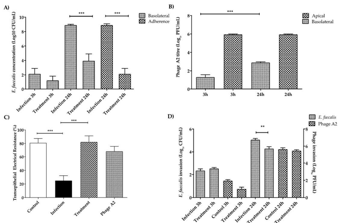
Figure 6. (A) E. faecalis adherence and translocation through intestinal epithelium and the effect of phage A2 predation. E. faecalis was left to adhere to the co-cultures for 3 h. At that point, treatment groups were inoculated with phage A2. (B) Enterococcus phage A2 translocation through intestinal epithelium when grown in trans-wells. Phage A2 was left to adhere to the co-cultures for 3 h. Then, fresh media was added to the wells without E. faecalis . (C) Co-culture trans-epithelial electrical resistance during exposure to E. faecalis and Enterococcus phage A2. E. faecalis was left to adhere to the co-cultures for 3 h. Treatment groups were inoculated with phage A2. The control and the phage groups were left uninfected with E. faecalis . (D) E. faecalis and phage A2 invasion of the intestinal epithelium. E. faecalis was left to adhere to the co-cultures for 3 h. At that point, the treatment groups were inoculated with phage A2. After 3 h or 24 h the samples were treated for 2 h with penicillin G to remove all the extracellular E. faecalis . Phage controls were not infected with E. faecalis , these groups were used to check phage invasion without the host. Columns show average concentration ( n = 9 ) \pm standard error. ** p < 0.01 ; *** p < 0.001 .
