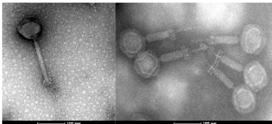
Figure 1. Electron micrograph of Enterococcus phage A2. Phage particles were negatively stained with 0.5% ( w/v ) uranyl acetate. Scale bar represents 100 nm.
