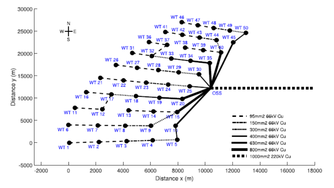
Figure 6. Example array cable network with varied sizes [38]
