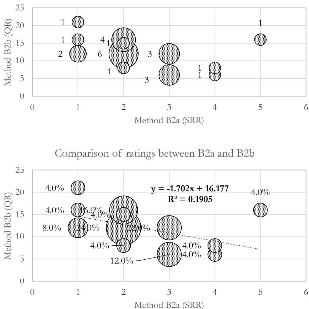
Figure 11.88 Results of the comparison between Method B2a and B2b for Data block 2.
