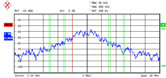
Fig. 2. Typical 802.15.4 distorted spectrum
