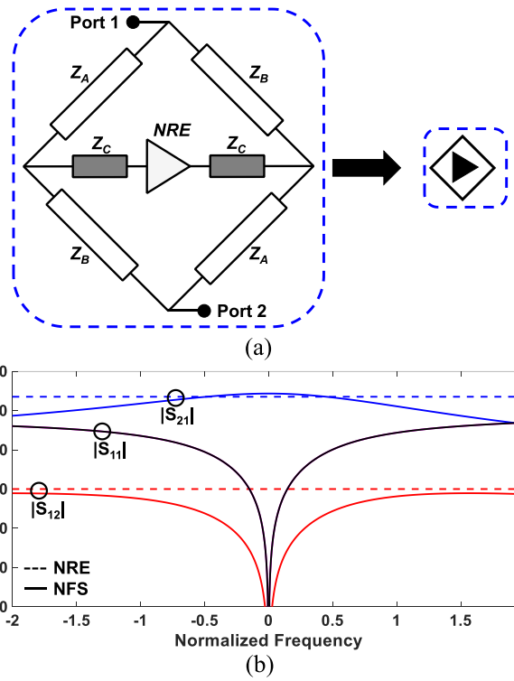
Fig. 2. NFS with enhanced power transmission response in the forward direction ( |S_{21}| ) and complete RF signal cancellation in the reverse one ( |S_{12}| ). (a) Block diagram and symbol, white and grey rectangles represent 90^\circ -long transmission lines at f_{cen} , white triangle: NRE with or without gain. (b) Ideal power transmission ( |S_{21}| ), isolation ( |S_{12}| ), and reflection ( |S_{11}| , |S_{22}| ) responses of the NFS (solid lines) and its corresponding NRE (dashed lines). The element values for this example are: Z_A = 11.9 \Omega , Z_B = 71.1 \Omega , Z_C = 12.1 \Omega , NRE S-parameters: S_{11} = 0 , S_{12} = 0.17 , S_{21} = 1.5 , and S_{22} = 0 .
