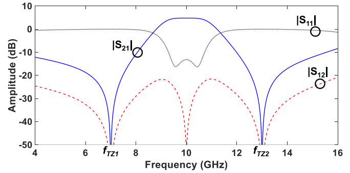
Fig. 7. S-parameters for the NBPF in Fig. 6(a) with separated reflection poles in the passband. The impedances for the inverters and multi-resonant cell are as follows: Z_{INV} = 50 \Omega , Z_{INV1} = 40 \Omega , Z_{TZ1} = 30 \Omega , and Z_{TZ2} = 63 \Omega .
