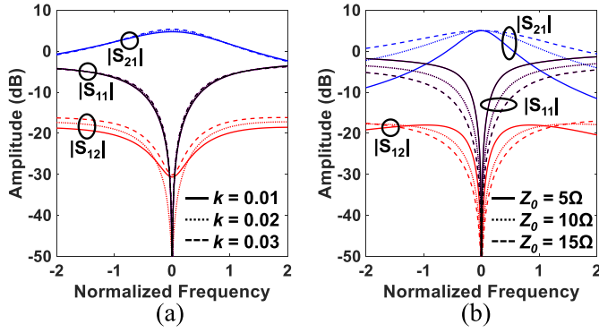
Fig. 3. RF power transmission ( |S_{21}| ), isolation ( |S_{12}| ), and reflection ( |S_{11}| ) response of the NFS as a function of (a) k when Z_0 = 12.1\ \Omega and (b) Z_0 when k = 0.028 . The NRE S-parameters are: S_{11} = 0 , S_{12} = 0.17 , S_{21} = 1.5 , and S_{22} = 0 .
