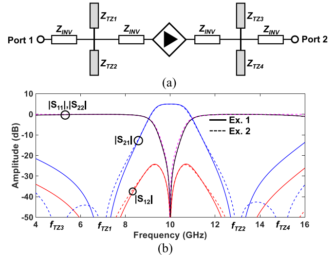
Fig. 8. (a) Block diagram for a three-resonator/four-TZ NBPF based on one NFS and two multi-resonant stages. (b) Comparison of the circuit-simulated power transmission ( |S_{21}| ), isolation ( |S_{12}| ), and reflection responses ( |S_{11}| , |S_{22}| ) for identical (Ex. 1) and non-identical multi-resonant stages (Ex. 2).
