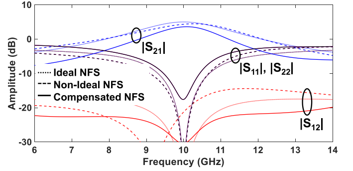
Fig. 10. Comparison of the S-parameter responses of an NFS with an ideal NRE (dotted trace), an NFS with a non-ideal NRE (dashed trace), and an NFS with a non-ideal NRE with the phase of Z_A , Z_B , and Z_C altered to compensate for the phase of the NRE (solid trace). The S-parameters for the non-ideal NRE are as follows: S_{11} = 0 , S_{12} = 0.15 - j0.08 , S_{21} = 1.1 + j1.1 , and S_{22} = 0 .
