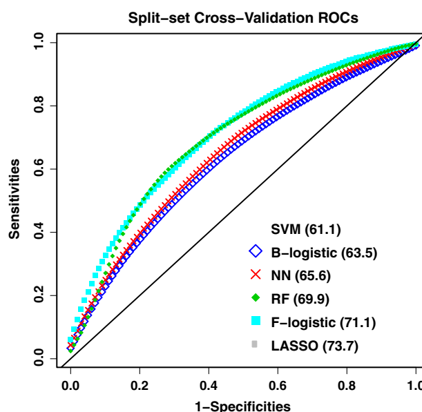
Fig. 3 Receiver operating characteristic curves for the classifiers for outcome-guided feature selection (SVM: support vector machines; F/B-logistic: forward- and backward stepwise logistic regression; NN: neural networks; RF: random forest). AUCs are specified in increasing order (inset). Random forests, forward-stepwise logistic regression, and the LASSO yielded effective discrimination rates.
