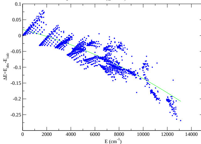
Figure 7: Residuals of matching between fully labelled MARVEL energy levels and our DVR3D calculations based on rigorous quantum numbers as well as energy. Matches were made within +0.1 \text{ cm}^{-1} and -0.05 \text{ cm}^{-1} of a quadratic fit (green).
