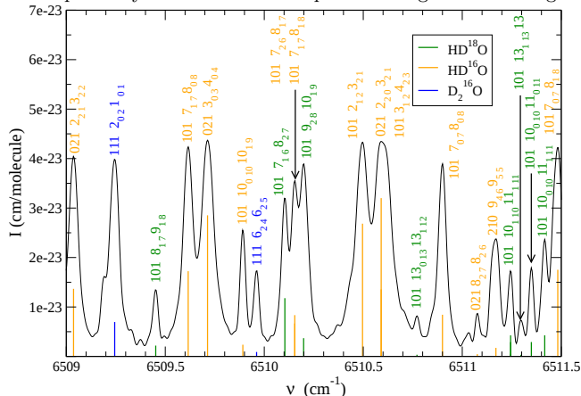
Figure 4: An assigned and labelled sample of the spectrum between 6509–6511.5 \text{cm}^{-1} . The continuous line represents the observed spectrum whilst sticks of different colour represent each isotopologue. The intensity scale refers to the calculated lines given as the height of the sticks. Labels are given in the format v_1''v_2''v_3''J_{K_a''K_c''}^{J_{K_a''K_c''}} where ' and '' represent lower and upper states respectively. Note the blended pairs of assignments arising from doublets.
