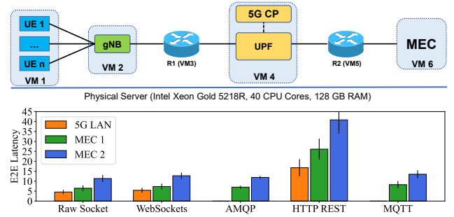
Fig. 3. Setup of 5G testbed and evaluation result.
