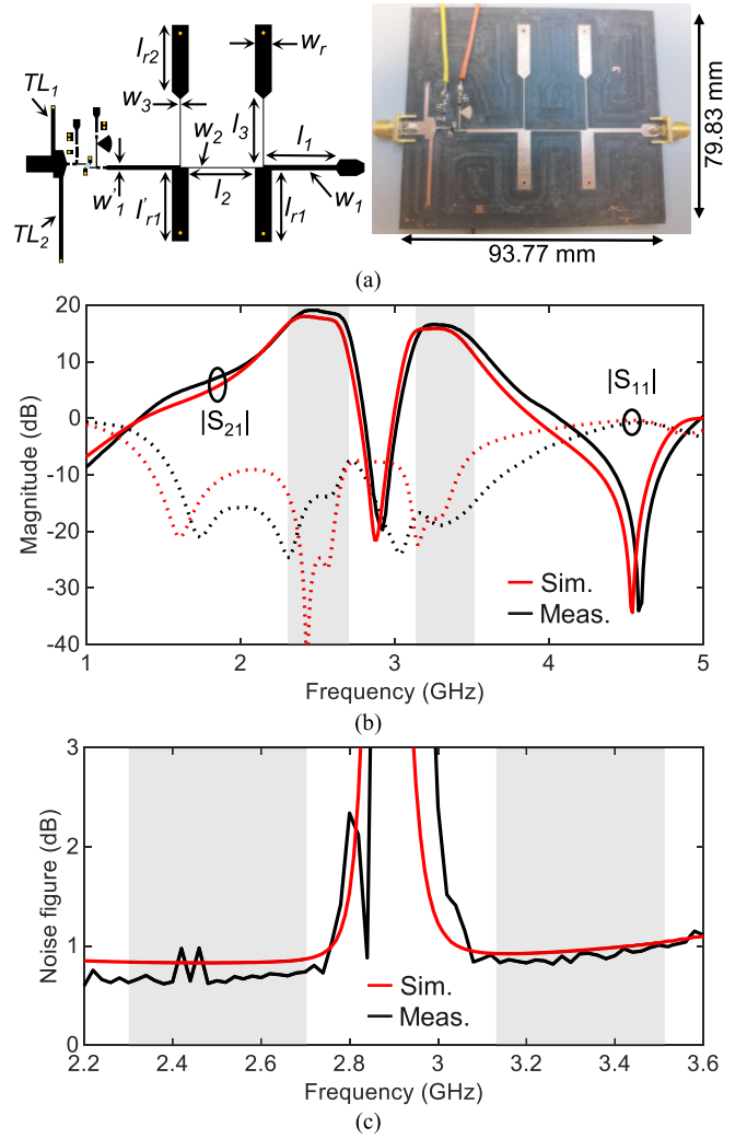
Fig. 8. (a) Layout (left) and manufactured (right) prototype of MBF-LNA I. Dimensions of the filter MN are as follows: TL_1 : l = 12.4 mm, w = 1.2 mm, TL_2 : l = 23.5 mm, w = 1.2 mm, OMN: l_1 = 17.8 mm, l_2 = l_3 = 18.3 mm, l_{r1} = 19.83 mm, l'_{r1} = 19.73 mm, l_{r2} = 18.53 mm, w_1 = 1.5 mm, w'_1 = 1.3 mm, w_2 = w_3 = 0.3 mm, w_r = 4.66 mm. (b) Measured and simulated S-parameter response for MBF-LNA I. (c) Measured and simulated NF of MBF-LNA I.
