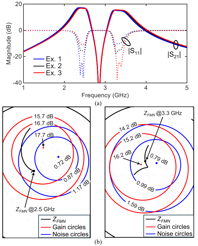
Fig. 6. (a) Simulated S-parameter response of the MBF-LNA in Fig. 4(b) with its IMN designed to match the optimal gain impedance at: 2.4 GHz (Example 1), 2.85 GHz (Example 2), and 3.3 GHz (Example 3). (b) Smith chart showing the constant gain (red) and constant noise (blue) circles of the transistor for the two passband frequencies centered at 2.5 GHz (left) and 3.3 GHz (right).
