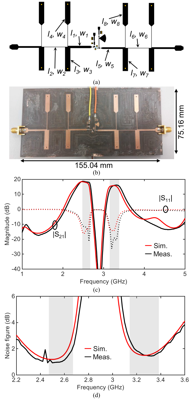
Fig. 10. (a) Layout of MBF-LNA II. Dimensions of the filter MNs are as follows: l_1 = l_5 = 17.8 mm, l_2 = l_6 = 18.3 mm, l_3 = l_7 = 19.33 mm, l_4 = l_8 = 18.53 mm, w_1 = w_5 = 1.5 mm, w_2 = w_3 = 0.3 mm, w_3 = w_4 = w_6 = w_8 = 4.66 mm. (b) Manufactured prototype of MBF-LNA II. (c) Measured and simulated S-parameter response of the MBF-LNA II. (d) Measured and simulated NF of the MBF-LNA II.
