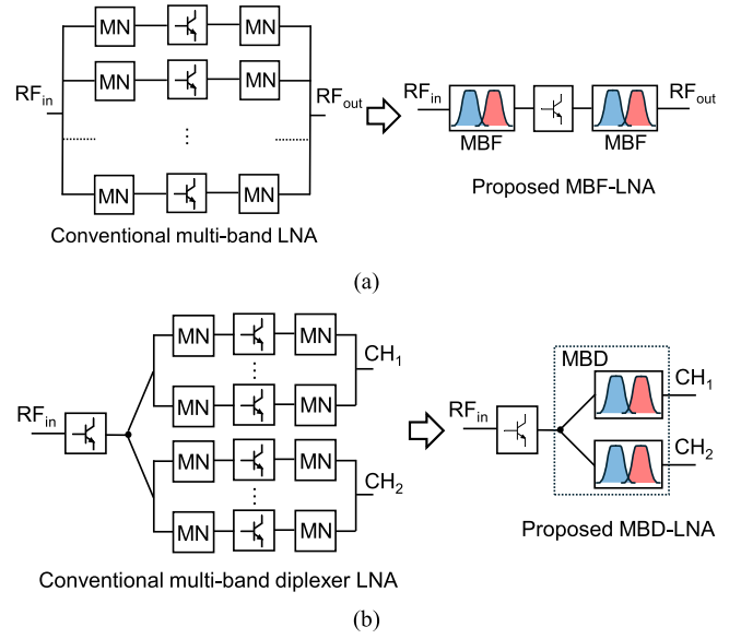
Fig. 1. Conceptual block diagram of the proposed multi-band filter LNA (MBF-LNA) and multi-band diplexer LNA (MBD-LNA) concepts. (a) Conventional and proposed MBF-LNA using complex-terminated split-type multi-resonant matching networks that are directly attached to a low noise transistor. (b) Conventional and proposed MBD-LNA using complex-terminated split-type multi-resonant diplexer matching networks that are directly attached to a low noise transistor.
