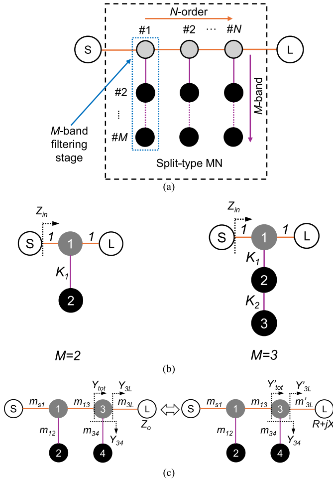
Fig. 2. (a) Coupling routing diagram (CRD) of the M -band N^{th} -order split-type filter matching network. Grey circles: in-line resonators, black circles: in-parallel resonators, white circles: source and load, orange and purple lines: frequency-independent couplings. (b) CRD of the M -band filtering stage for M = 2 and 3 . (c) Dual-band second-order example for conventional 50\ \Omega and arbitrary complex termination of the CRD in (a) where N = 2 and M = 2 .
