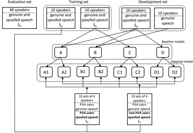
Figure 1: The usage of ASVspooft data to develop baseline models and to further adapt them to PVA users. The spoofing attack sets S_0 = \{A01, \dots, A06\} and S_3 = \{A07, \dots, A19\} .
