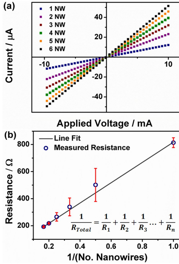
Fig 3: (a) Typical Ohmic responses observed for two point current voltage measurements obtained for nanowire arrays with increasing number of nanowire elements. (b) Plot of total resistance versus inverse number of nanowires present in the array. Inset: Equation for total device resistance where there are resistors positioned in parallel.
