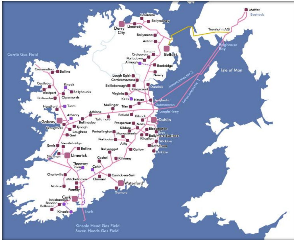
Figure 3.3 Map of Ireland's Natural Gas Grid (Bord Gáis Éireann)
