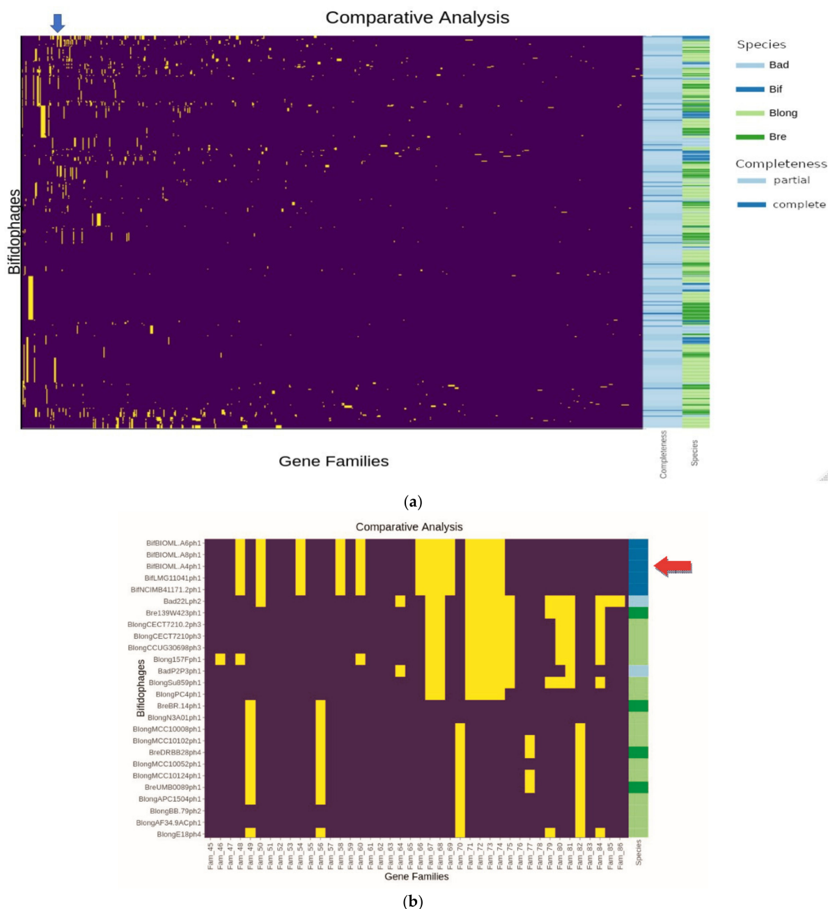
Figure 3. (a) Comparative Analysis heatmap produced by heatmaply. Gene families are presented on the horizontal axis, while bifidophages are presented on the vertical axis. We used a binary yes/no 100% gene similarity cut off. Gene families that are present are represented by a yellow cell, while purple indicates gene absence. Specifically, yellow cells on the same vertical line indicate a gene family present in multiple bifidophages, while yellow cells on the same horizontal line indicates multiple gene families present in a single bifidophages. The rowside legends indicates which species of bifidobacteria the phage belongs to and the degree of completeness predicted by PHASTER. B. longum is represented in pale green, B. breve in dark green, B. adolescentis in pale blue, and B. bifidum in dark blue. As previous, bifidophages predicted to be likely complete or complete are highlighted in dark blue and suspected partial or likely remnant bifidophages are highlighted in light blue. A blue arrow highlights an example of a cluster of multiple genes shared between the same Bifidobacterium bifidum strains highlighted in Figure 2. A red arrow indicates an example of gene families from a bifidophages shared across multiple Bifidobacterium species, highlighted in Figure 2. (b) Comparative analysis heatmap highlighting the same cluster represented in Figure 2 indicated here by a red arrow. This image is a zoomed-in view of the area highlighted in Figure 3a. Multiple gene families are shared between the B. bifidum phages BifBIOML-a4 phase 1, BifBIOML-a6 phase 1, BifBIOML-a8 phase 1, Bif LMG11041 phase 1 and BifNCIMB41171 phase 1. There is also an example of interspecies gene sharing between phages targeting hosts from B. adolescentis , B. breve , and B. longum directly below the bifidum example. Most notably, Bad22L phase 2, Bre139W423 phase 1 and BlongSu859 phase 1.
