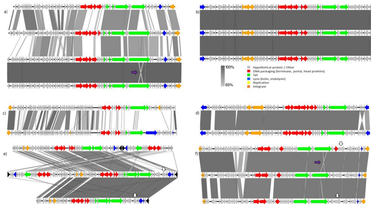
Figure 4. Bifidophages genomic comparison and characterisation by Easyfig. Each arrow indicates an open reading frame, orientated in the direction of transcription. The length of arrows is proportional to the length of the predicted open reading frame. Genes predicted to have similar functions are marked with the same color. Grey arrows indicate hypothetical proteins. Genome architecture and mosaic relationships between the prophage genomes are highlighted with pairwise alignments. The colour spectrum between genomes reflects amino acid identity as shown in the percentage based legend. The prophages in each alignment are described in descending order according to the above representations and are described further in the accompanying text. (a) Bre215W447aph1, BreDRBB30ph3, BadTF06-29ph2 and Bad11ph1. (b) BifBIOML-A4ph1, BifBIOML-A6ph1 and BifBIOML-A8ph1. (c) BlongATCC15697ph1 (from B. longum subsp. infantis ) and BlongTF06-12ACph1 (from B. longum subsp. longum ). (d) Bre139W423ph1 and BlongCECT7210ph3. (e) Bif85Bph3, BreDRBB30ph2 and BreLMC520ph1. (f) BlongAF05-2ph1 (from B. longum subsp. longum ), BreDRBB29ph1 and BreBR3ph5. The purple arrows highlight sequence inversions observed in phage tail-encoding genes. The white arrows highlight reverse transcriptase encoding genes mentioned in Section 3.3.3.
