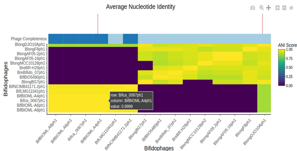
Figure 2. Interactive elements of ANI heatmap produced by heatmaply. Each cell can be highlighted to display the ANI value and the associated bifidophages. Representation of the lowermost left cluster in Figure 1 showing high intra-species ANI of a prophage-like region across several Bifidobacterium bifidum strains. Notably, five of the six regions were annotated as “likely complete” prophages by PHASTER.
