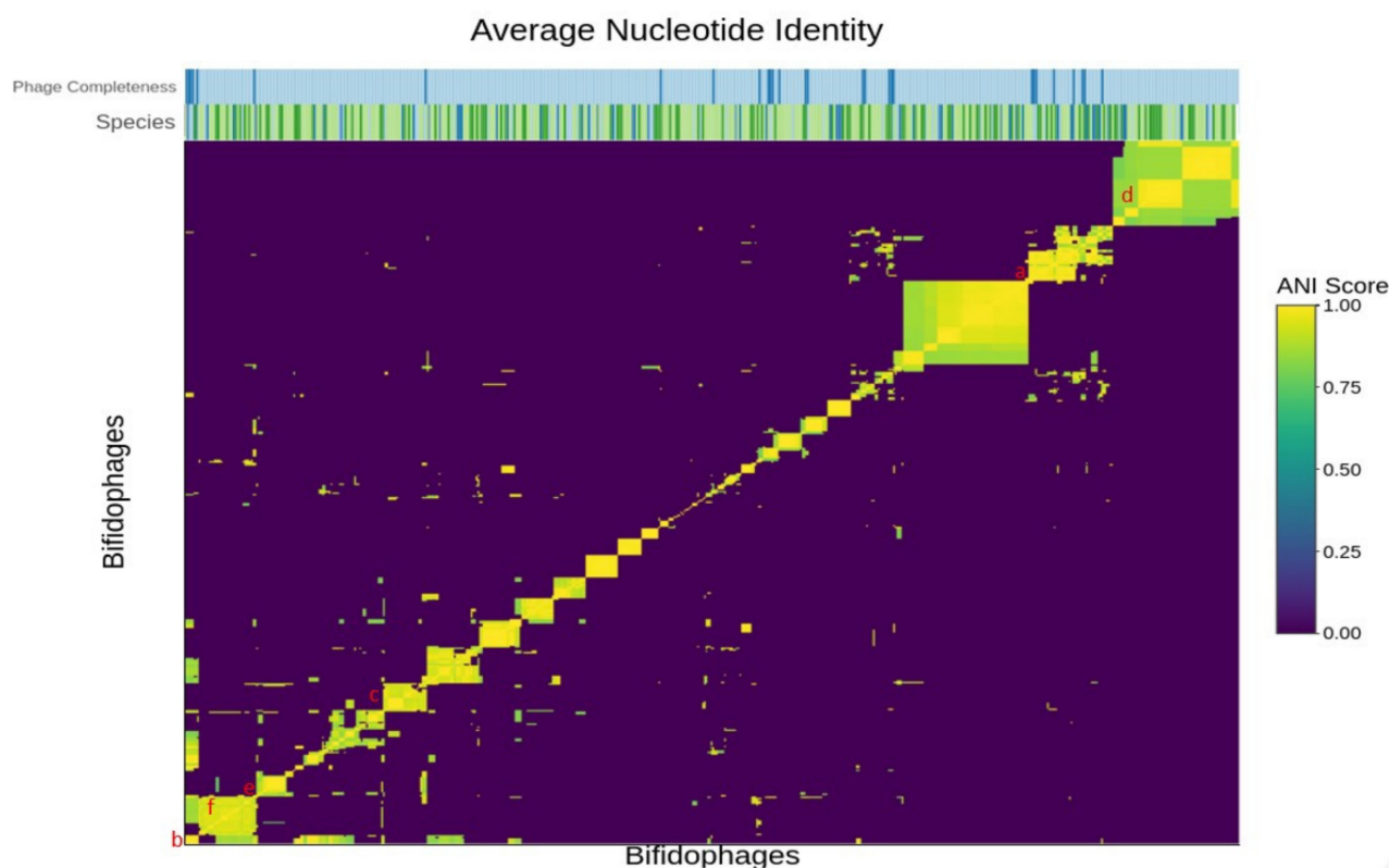
Figure 1. ANI heatmap produced by heatmaply. Yellow boxes in the heatmap signify prophage sequences with high levels of nucleotide similarity to each other. There are clusters of high similarity at both intra- and inter-species levels. The rowside legend indicates the degree of predicted completeness of the predicted prophages. Bifidophages predicted to be likely complete or complete are highlighted in dark blue on the “Completeness” column key. Suspected partial or likely remnant bifidophages are highlighted in light blue. The red letters a to f represent the six clusters highlighted in Figure 4.
