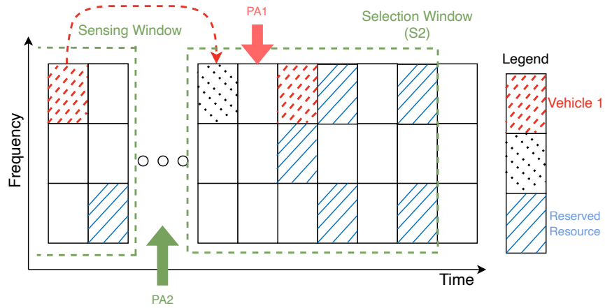
Figure 4.1: Impact of Missed Transmission on SB-SPS Scheduling
