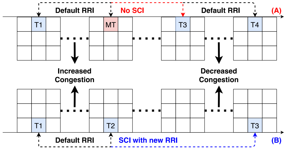
Figure 4.13: RRI DCC approaches versus default NR-V2X SB-SPS approach.
