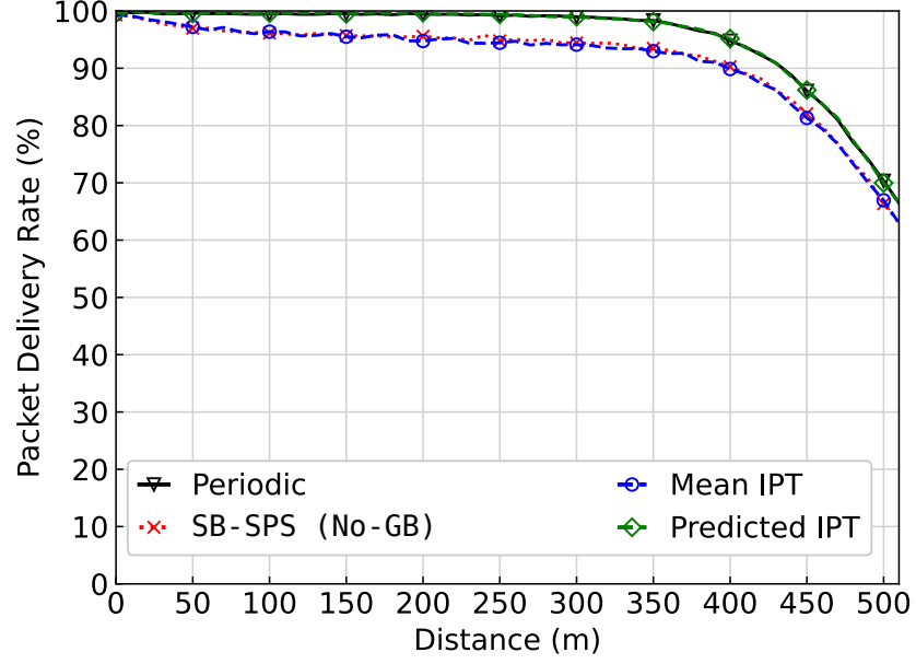
Figure 5.12: Performance of ETSI traffic model in a highway scenario (fixed vehicle speed).
