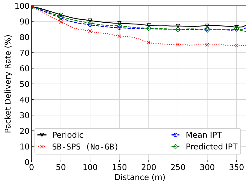
Figure 5.13: Performance of ETSI traffic model in a curved highway (varying vehicle headings).
