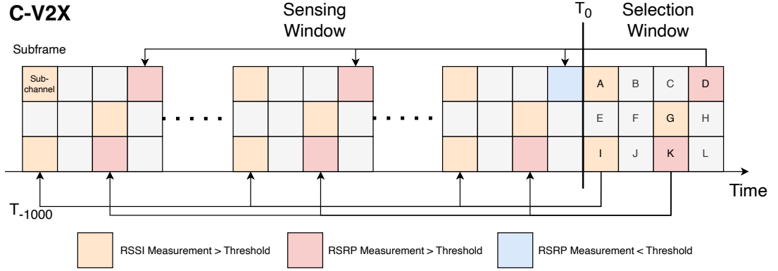
Figure 2.5: C-V2X SB-SPS mechanism
