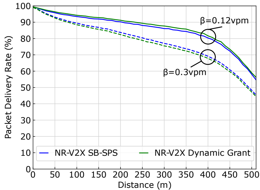
Figure 5.7: NR-V2X dynamic grant performance for fully aperiodic applications traffic. \beta=0.12 veh/m and \beta=0.3 veh/m.
