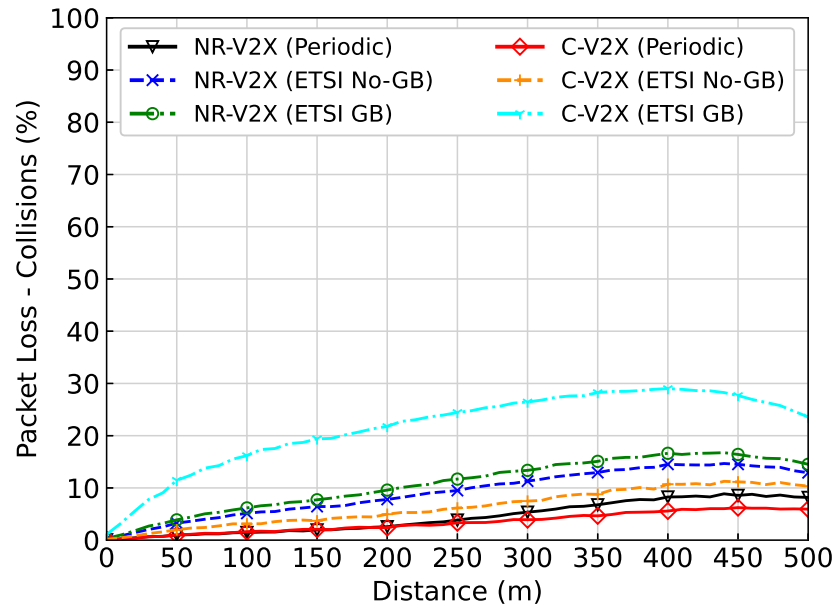
Figure 4.10: Packet collisions for periodic and ETSI application models, ( \beta = 0.12 veh/m)
