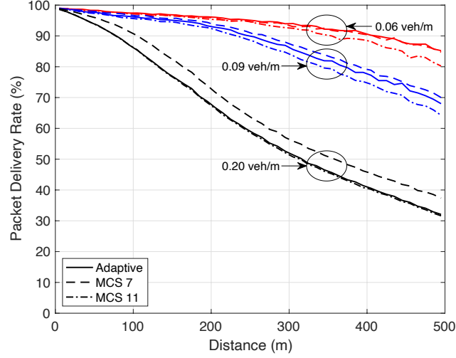
Figure 6.5: Packet Delivery Rate MCS congestion control.
