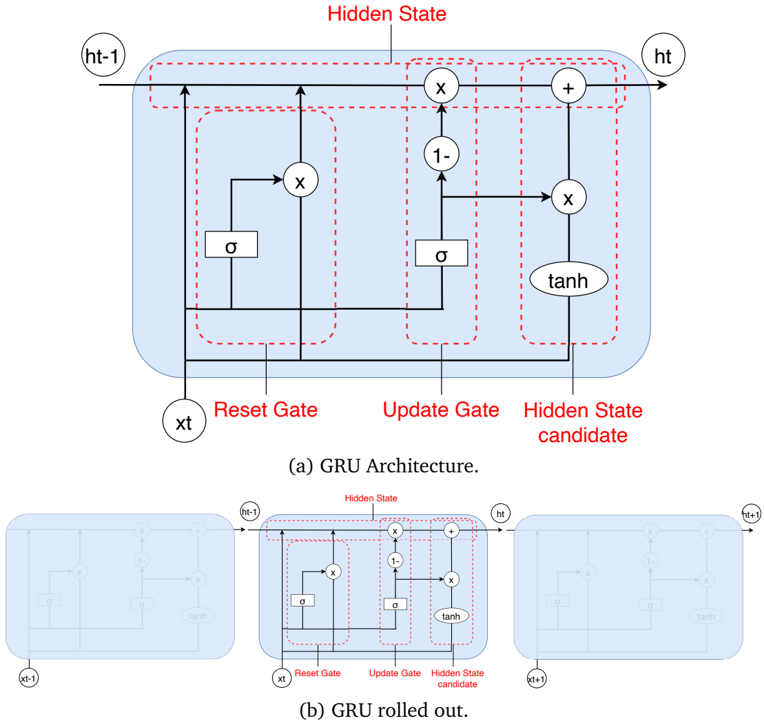
Figure 4.14: GRU (RNN) architecture diagram.
