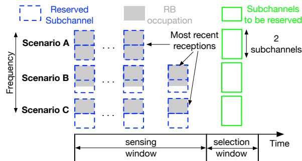
Figure 3.4: Subchannel and RB occupation during CSR selection with MCS adaptation.
