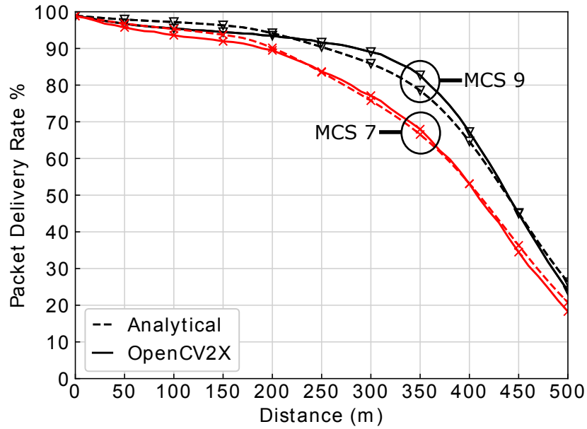
(b) PDR as a function of distance for variable MCS.
