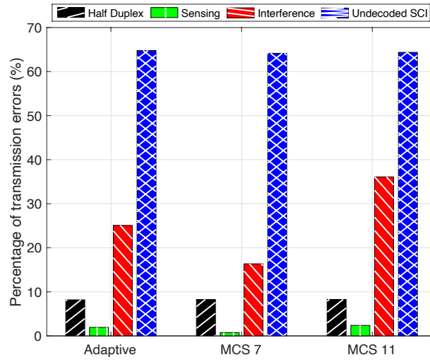
Figure 6.6: Percentage of transmission errors versus cause of error for all MCS configurations at 0.09 veh/m.
