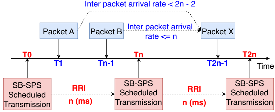
Figure 4.4: Interactions between packet inter-arrival rates and SB-SPS grant maintenance, where packet inter-arrival times are < 2n-2 (3GPP application model).
