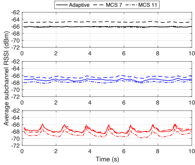
Figure 6.9: Average subchannel RSSI at 0.06 veh/m (lower figure), 0.09 veh/m (middle figure) and 0.20 veh/m (upper figure).
