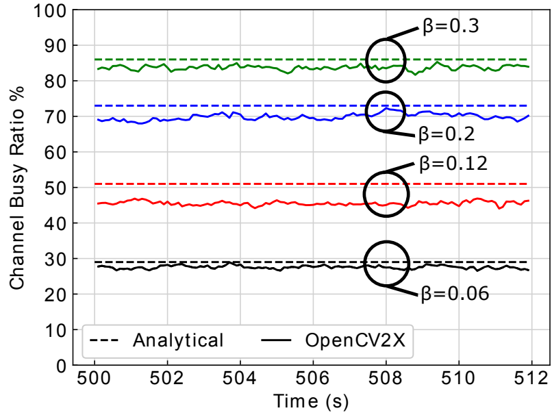
(a) PSSCH CBR for varying vehicular densities.
