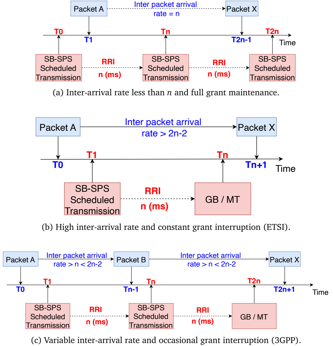
Figure 4.5: Grant maintenance and packet inter-arrival rate interactions.
