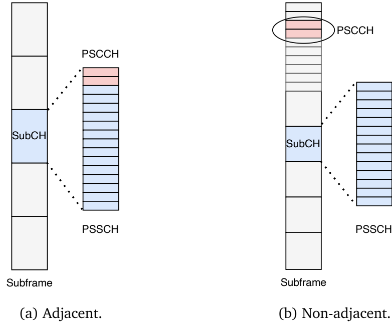
Figure 2.4: PSCCH &amp; PSSCH Adjacency.
