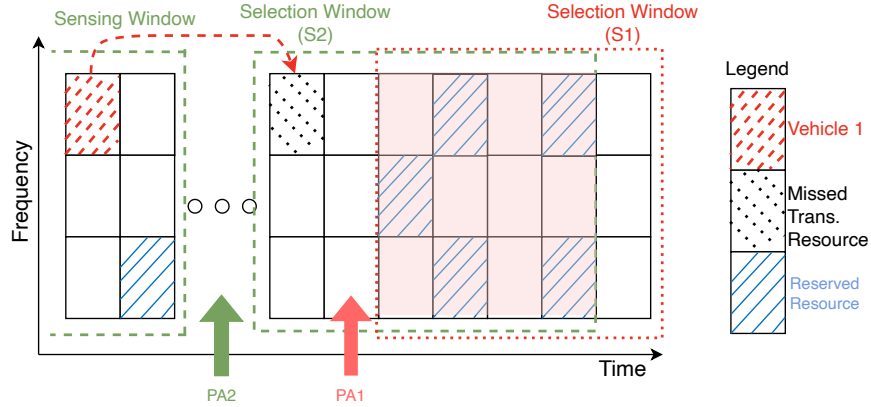
Figure 4.2: Impact of Grant Breaking on SB-SPS Scheduling
