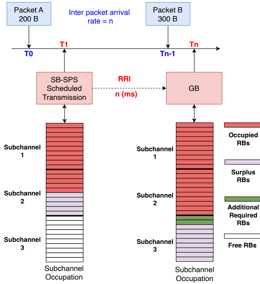
Figure 4.8: Impact of variable packet sizes
