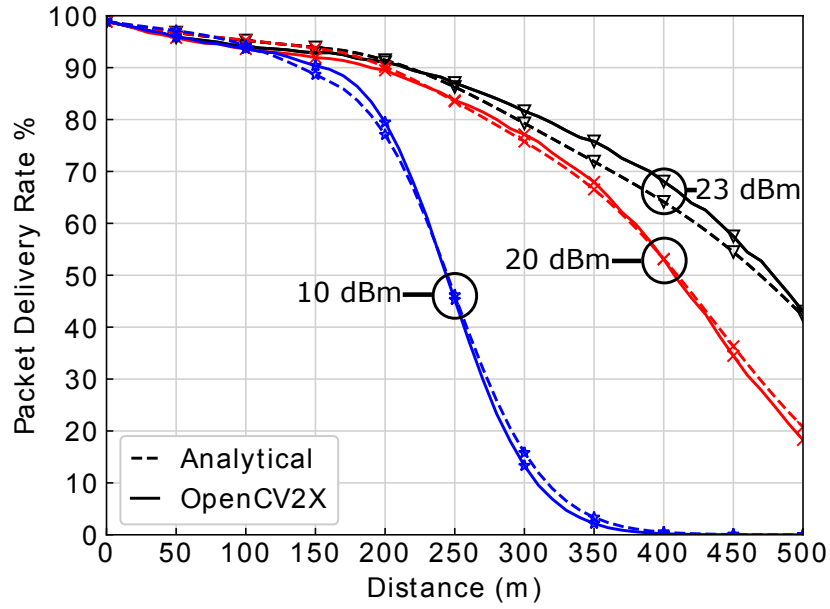
(a) PDR as a function of distance for variable transmission power.
