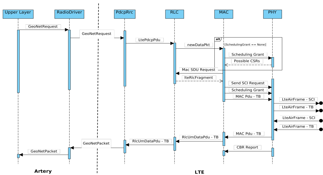
Figure 3.3: Sequence Diagram of packet exchange in OpenCV2X
