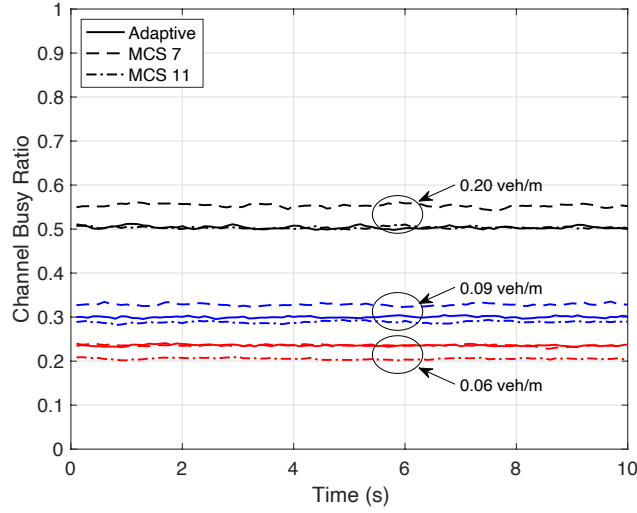
Figure 6.7: Channel Busy Ratio MCS congestion control.
