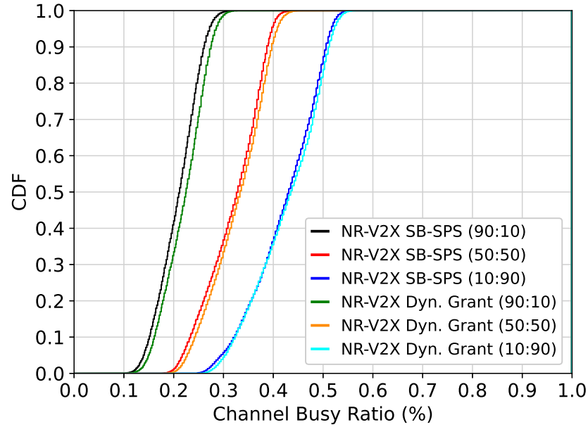
(b) NR-V2X CBR for SB-SPS & dynamic grant.
