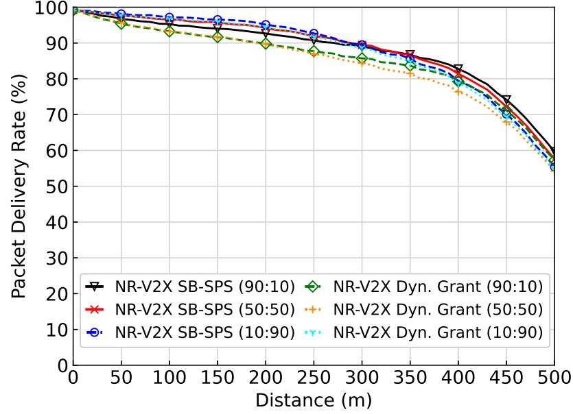
(a) NR-V2X PDR for SB-SPS & dynamic grant.
