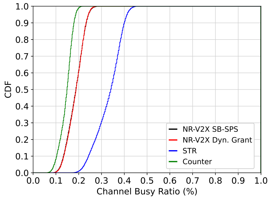
(b) Performance of default NR-V2X SB-SPS versus NR-V2X dynamic grant vs 2 alternative aperiodic scheduling mechanisms.
