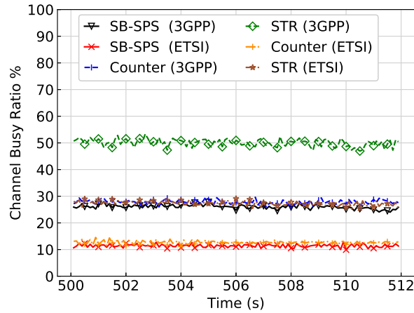
(c) PSCCH (Control Channel) Channel Busy Ratio (CBR) Comparison ( \beta=0.12 veh/m).
