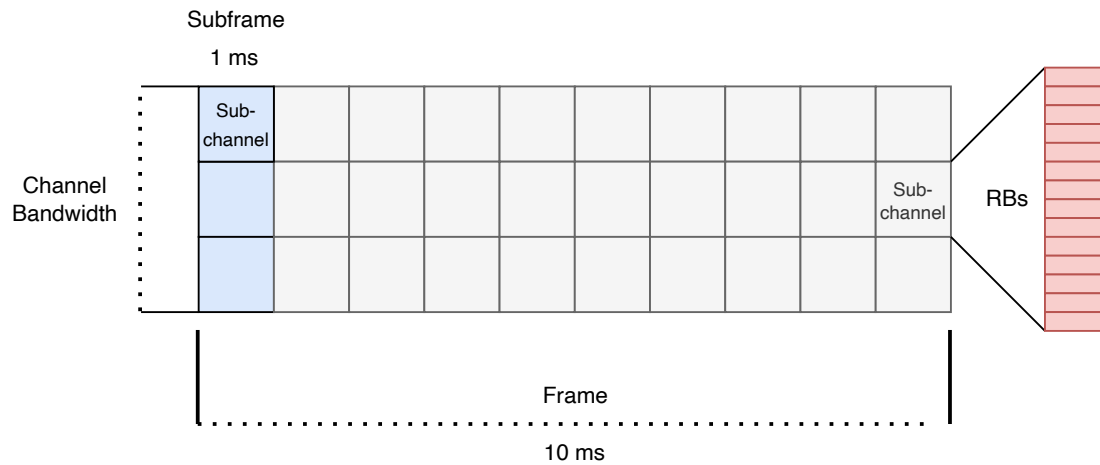
Figure 2.3: C-V2X Channelisation
