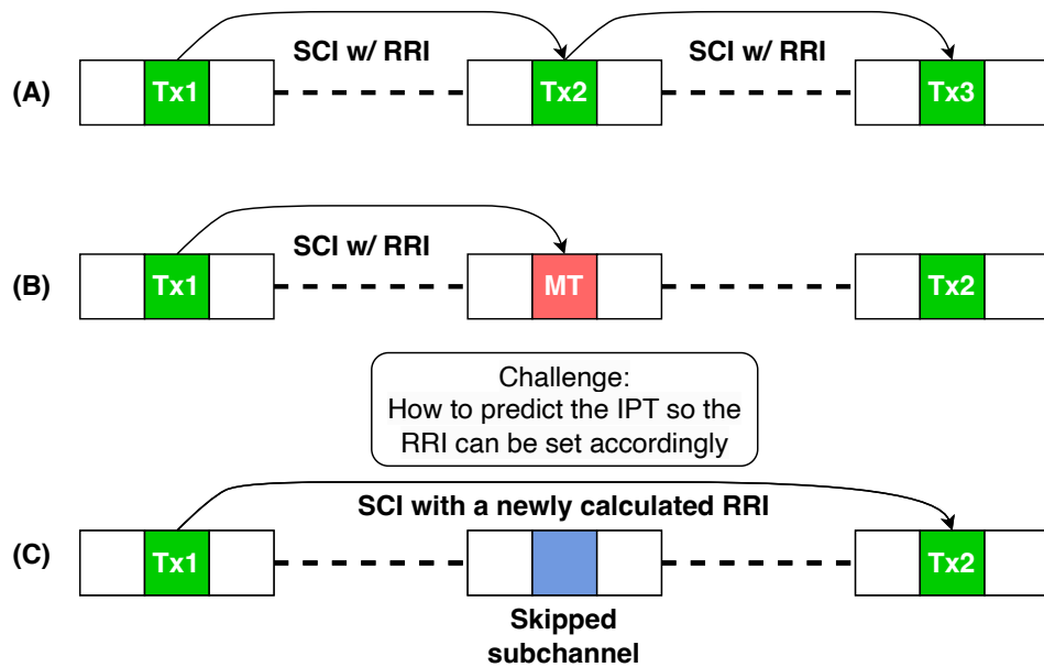
Figure 4.12: Overview of RRI Adaptation.
