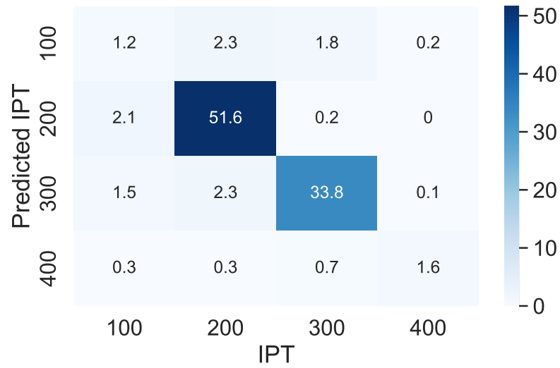
(b) RRI confusion matrix (overall percentage).
