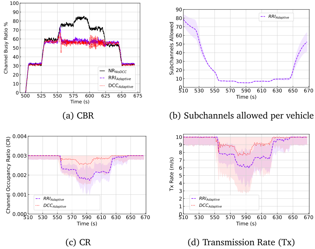
Figure 6.17: Long-form variable CBR simulation. Comparative stability statistics for a long form simulation exhibiting fluctuating congestion in the channel.
