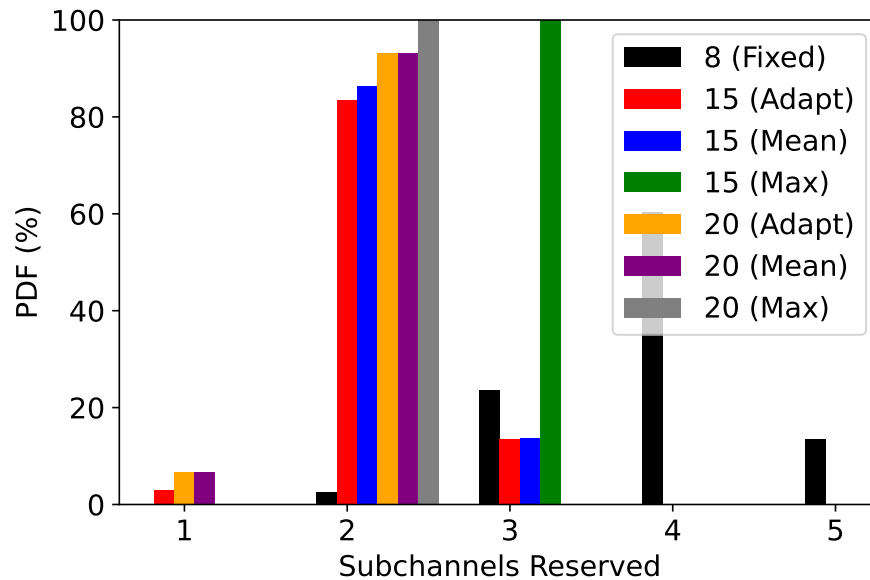
Figure 5.21: Subchannel Occupation (Renault)
