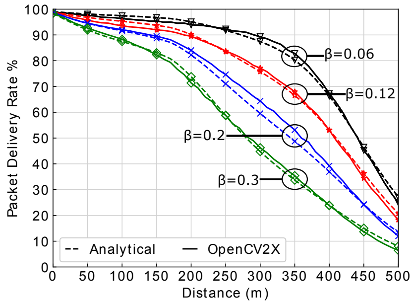
Figure 3.6: PDR as a function of the distance between the transmitter and receiver for varying vehicular densities for OpenCV2X versus analytical model.
