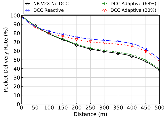
(a) ETSI DCC PDR (Reactive & Adaptive) Mode 2.
