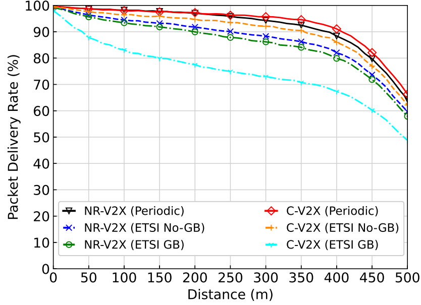
Figure 4.9: SB-SPS performance of NR-V2X and C-V2X for periodic and ETSI application models ( \beta = 0.12 veh/m, with and without grant breaking (GB & No-GB)).
