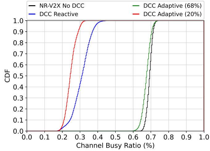
(b) ETSI DCC CBR (Reactive & Adaptive) Mode 2.
