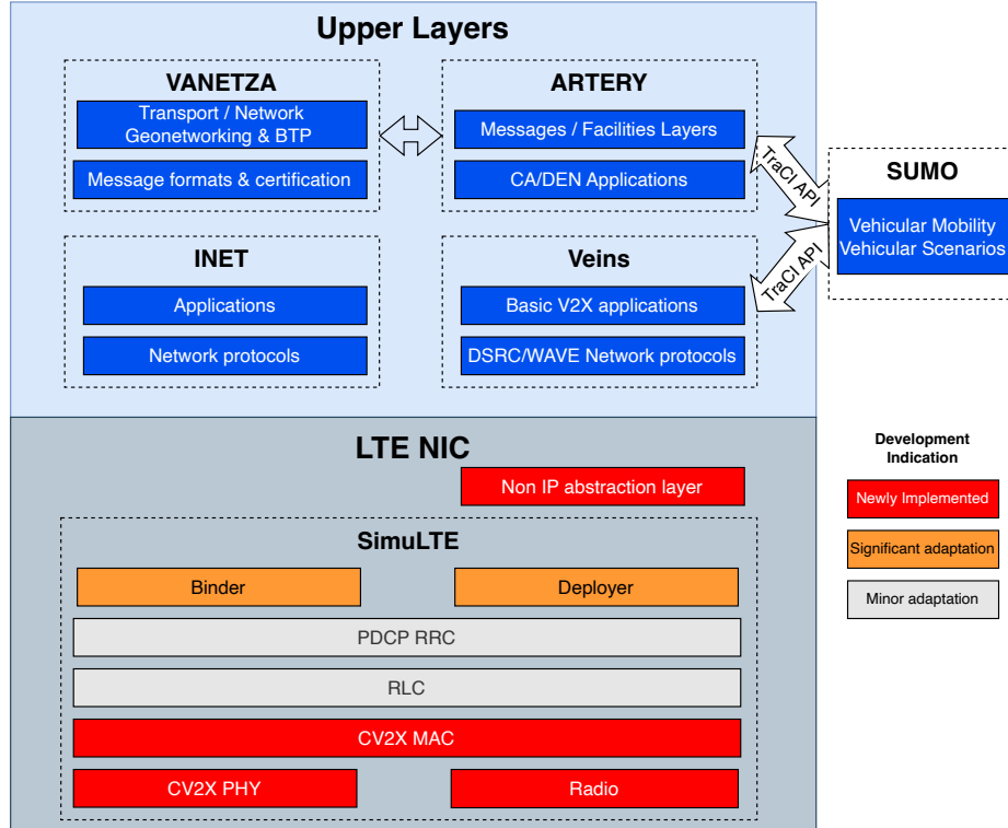
Figure 3.2: OpenCV2X model architecture with Artery.
