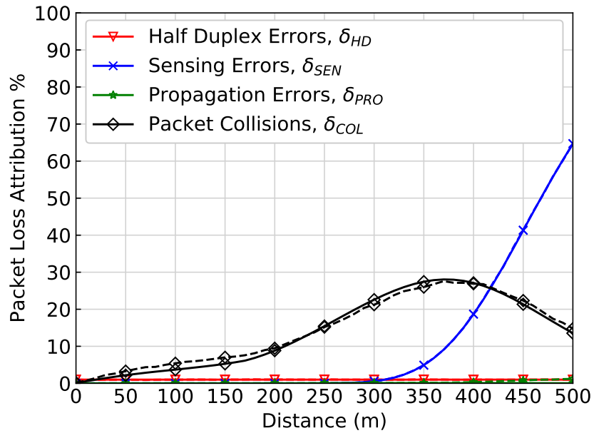
(b) Packet Loss Attribution per type of error ( \beta=0.12 veh/m) for OpenCV2X (solid lines) and the analytical model (dashed lines).
