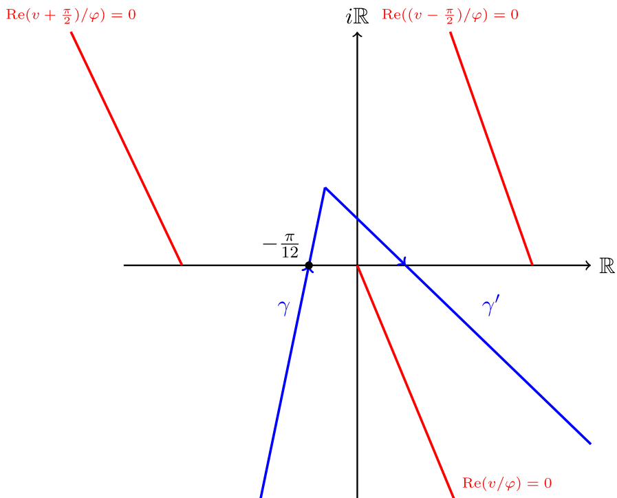
Fig. 7 The contours \mathcal{S} , parameterized by \gamma, \gamma' (after applying Lemma 2.1)
