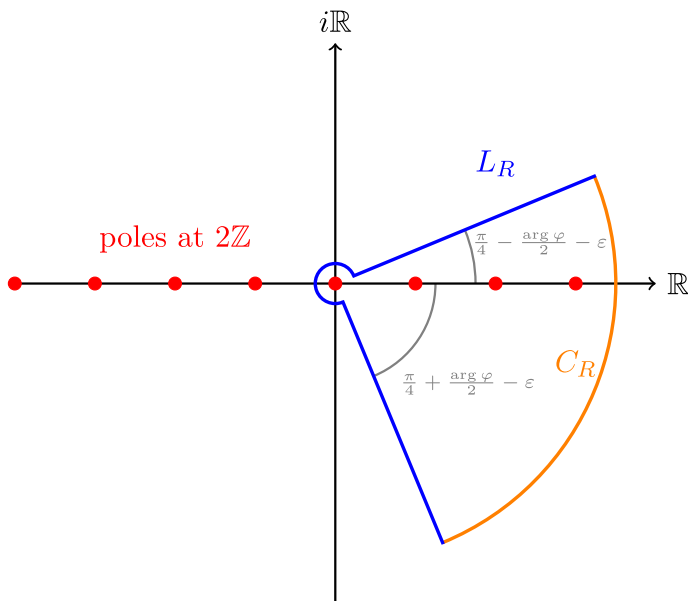
Fig. 4 Contours L_R and C_R
