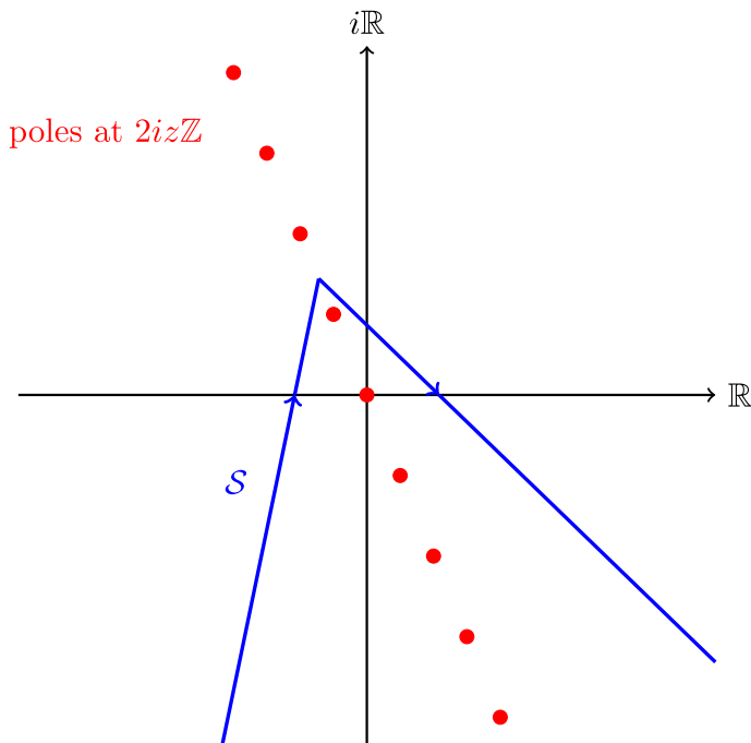
Fig. 6 A contour S (before applying Lemma 2.1)
