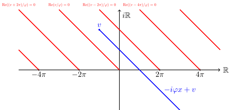
Fig. 3 The branch cuts of \text{Li}_s^\varphi(e^{-iv}) , s = 1, 2 and -i\varphi x + v for x \geq 0
