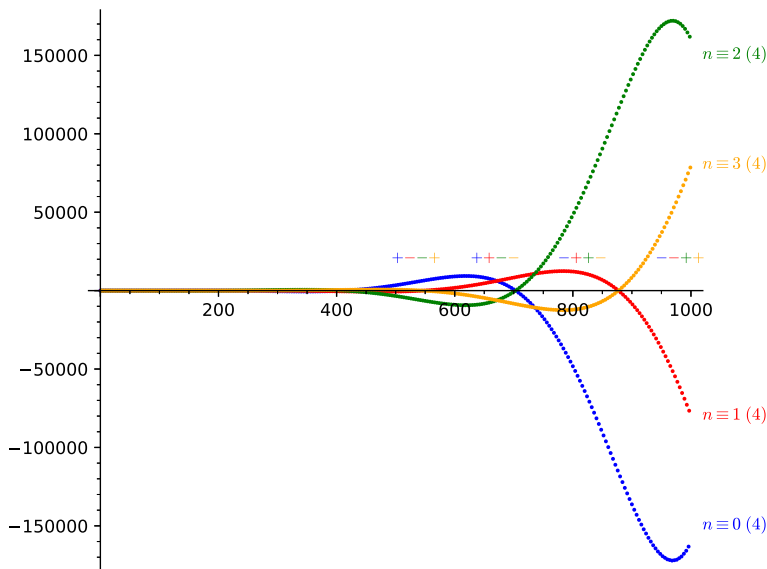
Fig. 1 V_1(n) for n = 1, \dots, 1000
