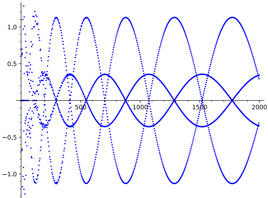
Fig. 2 V_1(n)e^{-\sqrt{2|V|n}}\sqrt{n} for 0 \leq n \leq 2000
