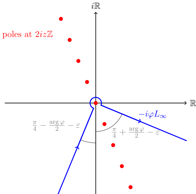
Fig. 5 The contour -i\varphi L_\infty
