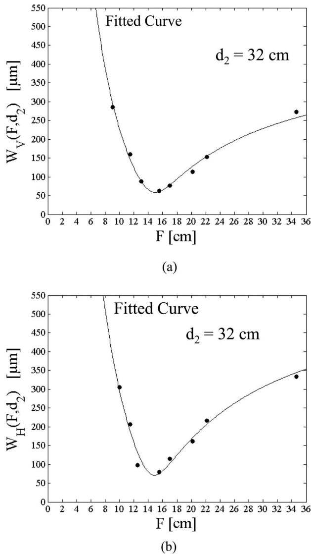
FIG. 4. Characterization of a multimode laser beam using the proposed DMD-ECVFL beam analyzer. Data shown are the second-moment irradiance beam waist radius as a function of the ECVFL focal length F for (a) the vertical (or y direction) and (b) the horizontal (or x direction) beams.
