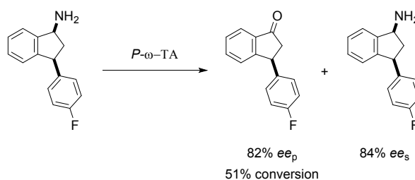
Scheme 6: Synthetic utility of P -ω-TA which yielded good enantiopurity in both recovered substrate and product
