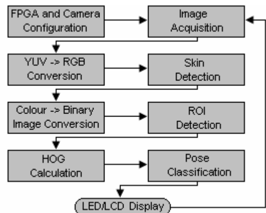
Fig. 5 Block diagram of the Handle-C algorithm operation
