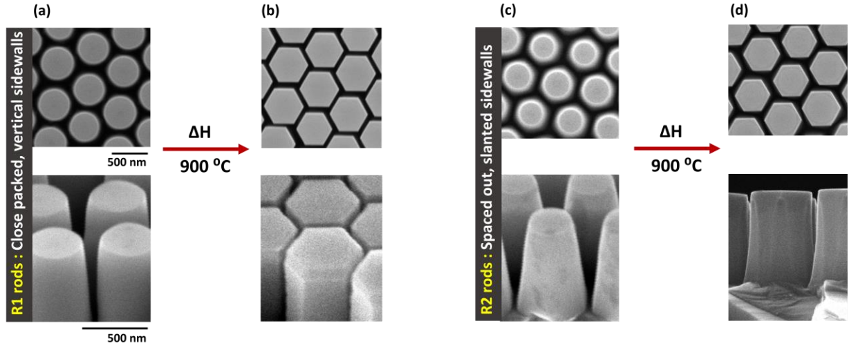
Figure 1. SEM surface analysis of R1 type nanorods (a) pre-anneal and (b) post 900 °C anneal, and R2 type nanorods (c) pre-anneal and (d) post 900 °C anneal.
