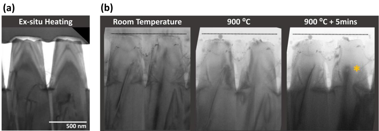
Figure 4. TEM image of R2 GaN nanorods after (a) ex-situ 900 °C and (b) in-situ 900°C anneal.
