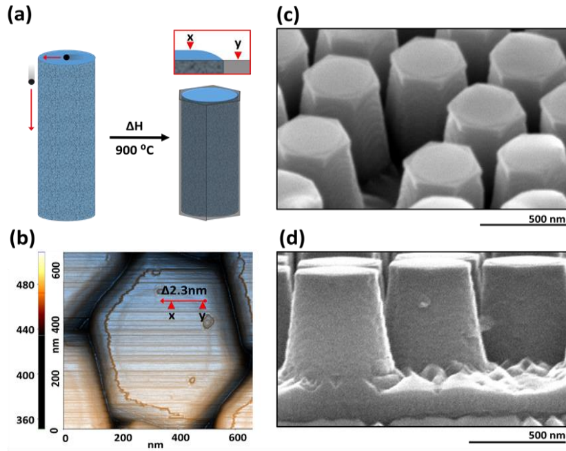
Figure 3. (a) schematic illustration of the change in morphology and decreasing height after annealing, (b) AFM scan revealing the downwards step at this boundary, (c) and (d) SEM scans of the GaN nanorods with a SiO 2 sidewall coating after annealing at 900 °C.
