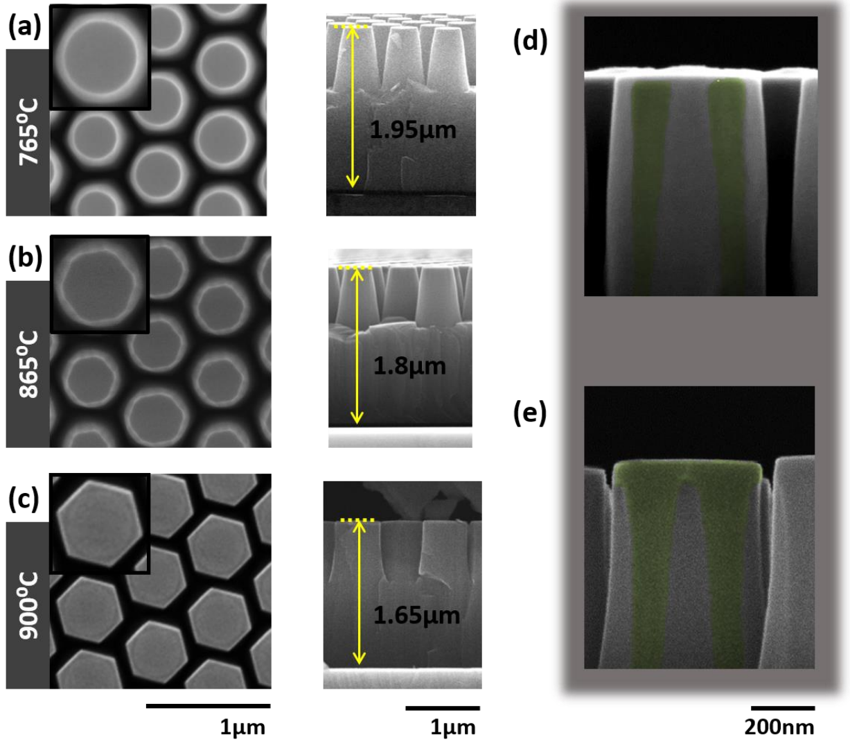
Figure 2. SEM scans of nanorod top surface and cross-section after anneals at (a) 765 °C, (b) 865 °C, (c) 900 °C, (d) and (e) higher magnification cross sectional SEM scans of (b) and (c) samples respectively, with new non-polar facets highlighted yellow.
