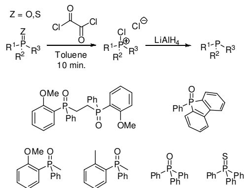
Chart 1. Phosphine chalcogenides that could be reduced by sequential treatment with oxalyl chloride and LiAlH 4 . a
