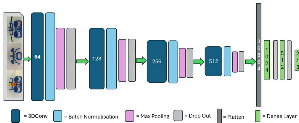
Fig. 4. Model architecture.
