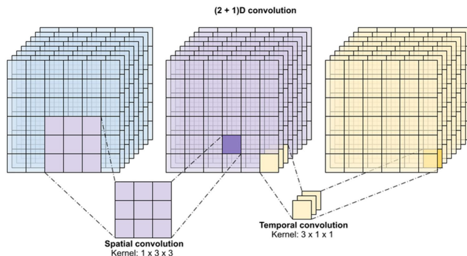
Fig. 3. Spatial and temporal kernel sliding in a 3DCNN. [figure from www.keras.io ].
