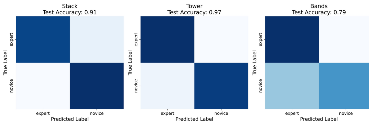
Fig. 14. Binary class confusion matrices.
