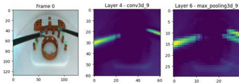
Fig. 5. Feature maps, left: input image, centre: conv layer, right: max pooling layer.
