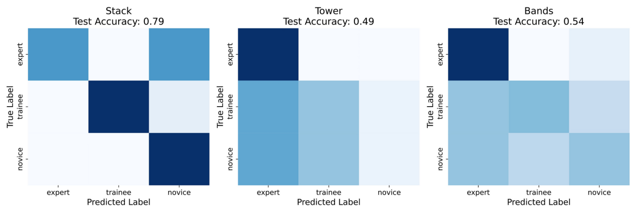
Fig. 13. Multi-class confusion matrices.
