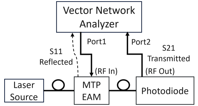
Figure 4. Schematic of measurement setup for S11 and S21 characterizations of MTP EAM
