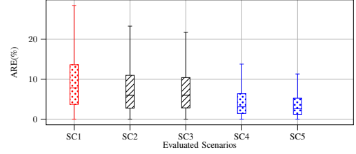
Fig. 1. Prediction accuracy for UDP traffic type under different scenarios (device-based and network-based), and data granularity (250ms and 1s)
