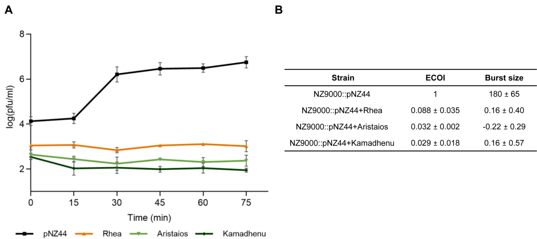
FIG 1 (A) One-step phage growth curve of phage sk1 and (B) ECOL and burst size of phage sk1 on L. cremoris NZ9000::pNZ44 and its phage-resistant derivatives harboring Rhea, Aristaios, and Kamadhenu antiphage systems. Experiments were performed in biological triplicate, and data are presented as means ± SD.
