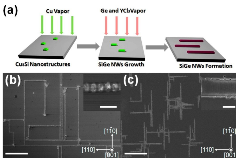
Figure 1.6 (a) Schematic illustration of the endotaxial SiGe nanowire formation process. SEM images of (b) the aligned SiGe nanowires synthesised at 720 °C on a Si wafer, where the inset shows the enlarged nanostructure, and (c) the same sample after silicate/oxide etching by HF, where the inset shows the enlarged SiGe nanowire surface. Scale bars for (b) and (c) are both 10 μm, 500 nm for the inset of (b), and 200 nm for the inset of (c) 55 .
