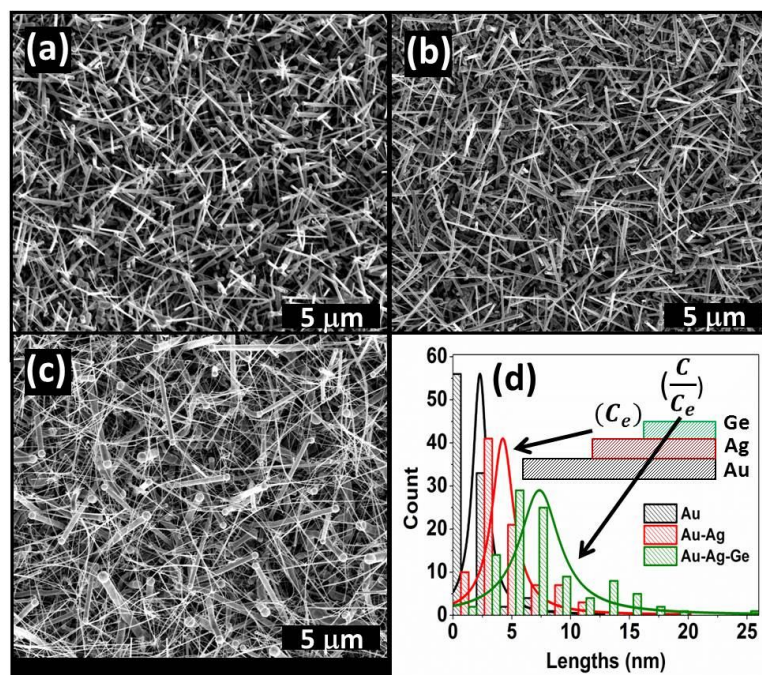
Figure 4.2 SEM images of Ge nanowires grown using a 3-part substrate. (a) Ge nanowires grown on the Au part of the 3-part substrate, (b) Ge nanowires grown on the Au/Ag bi-layer part of the 3-part substrate and (c) Ge nanowires grown on the Au/Ag/Ge part of the 3-part substrate. (d) Nanowire length distributions from the Au film, Au/Ag bi-layer and Au/Ag/Ge tri-layer showing how the mean nanowire length increases on proceeding from the Au film to the Au/Ag bi-layer and finally, to the Au/Ag/Ge tri-layer. The inset illustrates how each part of the substrate influences the growth kinetics, with the addition of Ag reducing C_{eq} in the bi-layer and the addition of Ge to Au/Ag increasing the solute concentration in the tri-layer.
