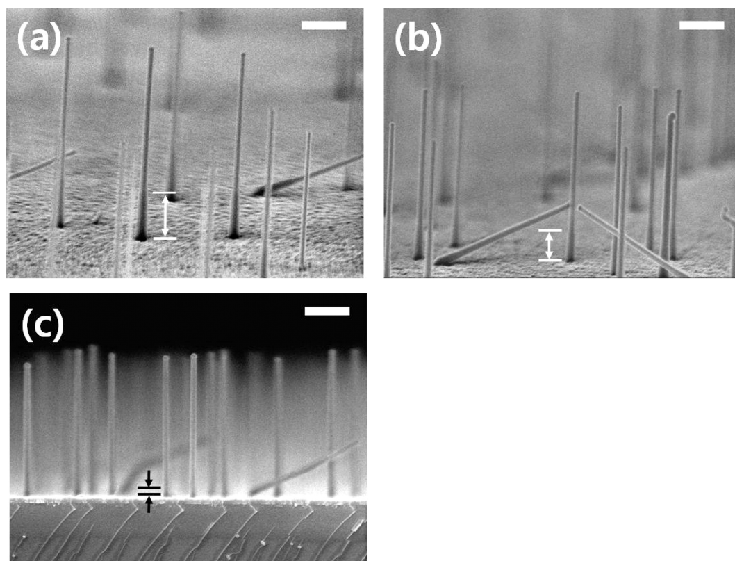
Figure 1.7 Side-view SEM images of Ge nanowires grown on a GeBSi substrate via a two-temperature process. The growth temperature during the base growth stage was 350 °C, while subsequent nanowire growth was performed at 300 °C for 20 min. The growth time during the base growth stage was: (a) 6 min, (b) 4 min and (c) 2 min. A 50 nm diameter Au colloidal solution was used. The regions marked by arrows in the SEM images are the part of nanowires grown during the base growth stage. Scale bar = 500 nm 56 .
