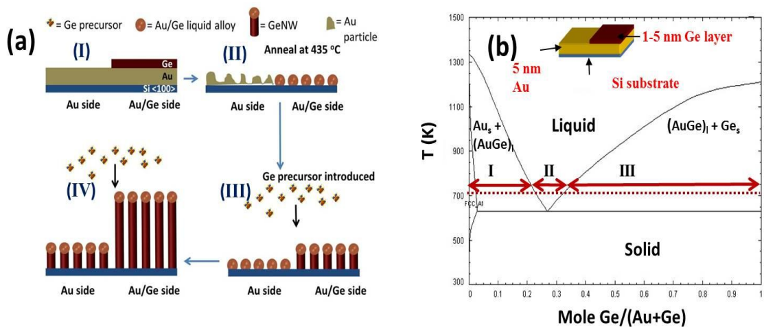
Figure 3.2 (a) Schematic illustrating the difference between Ge nanowire growth on the Au and Au/Ge bilayer side of a Si substrate. Nanowires grown on the bilayer side nucleate faster and thus have greater lengths than those on the Au side, for a given growth time. (b) Phase diagram of the Au/Ge alloy system tracing and comparing the evolution of Ge nanowires grown on the Au side and Au/Ge bilayer side of the substrate. Inset shows the 2-part substrate used which consists of a Au film on one side and a Au/Ge bilayer on the other side.
