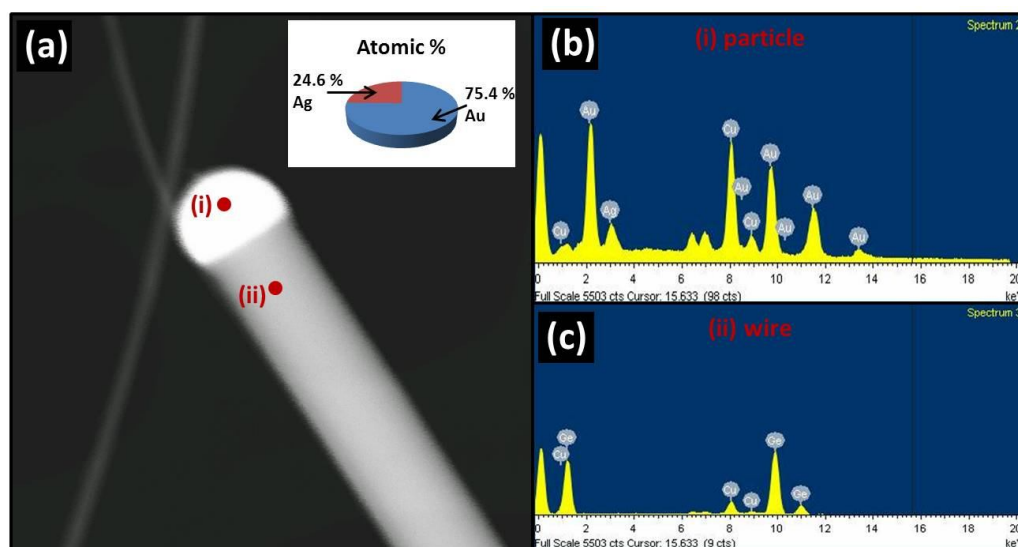
Figure 4.5 STEM analysis of a Ge nanowire grown from a Au/Ag seed. (a) High angle annular dark field (HAADF) STEM image of a Ge nanowire grown from a Au/Ag seed. Inset shows the atomic % of Ag and Au in the seed particle on top of the nanowire. (b) EDX spectrum of the seed taken at point (i) in (a). (c) EDX spectrum of the wire taken at point (ii) in (a).
