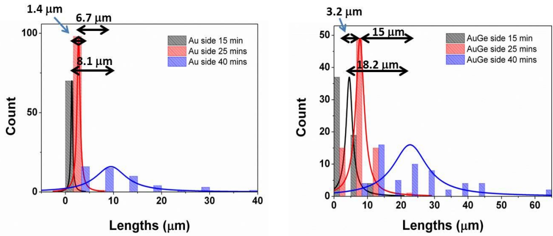
Figure 3.9 Length distributions of GeNWs at different growth times of 15, 25 and 40 mins. The length is shown to increase with growth time. (a) Length distribution for the Au side. (b) Length distribution for the Au/Ge side. The difference between mean lengths for different growth times is larger for the Au/Ge side, suggesting a higher growth rate.
