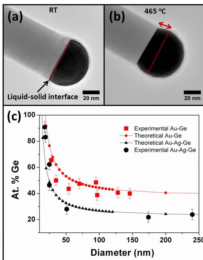
Figure 4.13. Data obtained from in-situ TEM heating of Ge nanowires grown from \text{Au}_{0.75}\text{Ag}_{0.25} and Au nanoparticle seeds. (a) TEM image of a \text{Au}_{0.75}\text{Ag}_{0.25} nanoparticle seeded Ge nanowire at room temperature. (b) TEM of the same nanowire after heating to the growth temperature of 465 °C. (a) and (b) show the expansion of the nanowire liquid-solid interface as a result of Ge uptake into the seed. (c) Plot of the equilibrium Ge atomic % calculated from particle expansion as a function of nanowire diameter for the Au/Ge (red squares) and Au/Ag/Ge (black hexagons) alloy systems. Simulated curves for the experimental data for the Au/Ge (red line) and Au/Ag/Ge (black line) of the supersaturation of Ge in Au and \text{Au}_{0.75}\text{Ag}_{0.25} nanoparticles are included.
