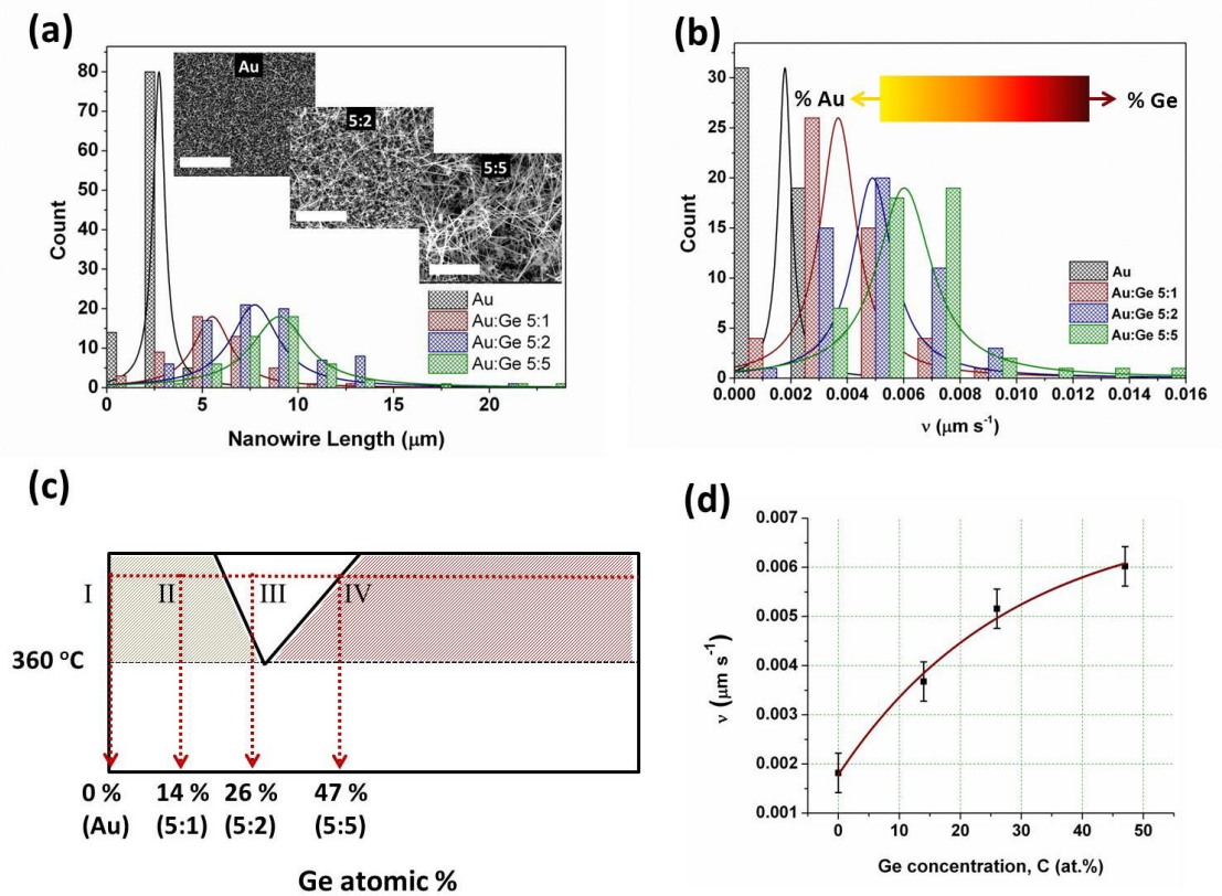
Figure 3.6 (a) Histogram showing the relative length distributions of Ge nanowires grown from a Au film and Au/Ge bilayers with varying Ge thicknesses. Growth time in all cases in 25 mins. Insets show SEM images of Ge nanowires grown from a Au film as well as Au/Ge bilayers, with Ge layer thickness of 2 and 5 nm. Scale bar is 5 \mu\text{m} (b) Histogram showing the relative growth rate distributions of Ge nanowires grown from a Au film and Au/Ge bilayers with varying Ge thicknesses. Lorentzian curves are fitted to all plots in (a) and (b), and show a broadening of the size distribution in the length and growth rate of GeNWs as the thickness of the Ge film increases. (c) Enhancement of the low-temperature regime of the Au/Ge phase diagram shown in figure 1(b) which traces the behavior of the binary alloy formed from bilayers with increasing Ge solute concentration, i.e. increasing Ge film thickness. (d) Mean nanowire growth rate as a function of the Ge solute concentration in the binary alloy.
