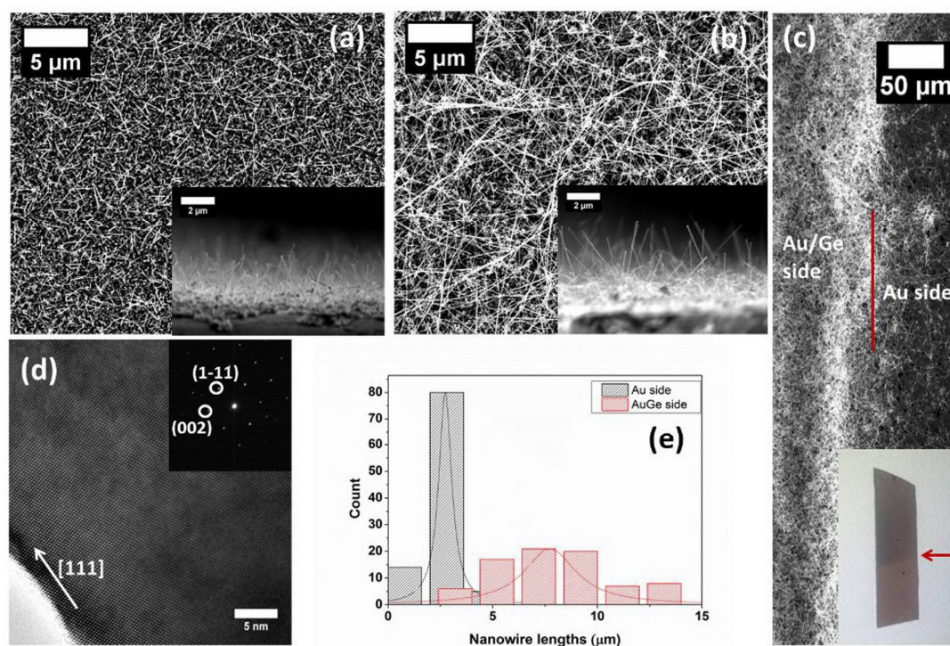
Figure 3.3 SEM and TEM images of Ge nanowires grown from a two-sided substrate. (a)–(b) Top-down SEM images showing Ge nanowires grown from the Au side and Au/Ge (5nm / 2 nm) side respectively; growth time was 25 min. Insets show cross-sectional SEM images of Ge nanowires on the Au side and Au/Ge side respectively. (c) Top-down SEM image showing the interface between the Au and Au/Ge side. Inset is a photograph taken of the substrate after removal from the CVD apparatus. The sharp interface implying different growth scenarios with the Au and Au/Ge film. (d) Lattice resolution TEM image of a Ge nanowires grown on the Au/Ge bilayer side. Inset is the SAED pattern viewed along the [110] zone axis which confirms the \langle 111 \rangle growth direction. (e) Histogram confirming the significant difference in nanowire lengths between the Au and Au/Ge side. Lorentzian curves are fitted to both plots to guide the eye, which show a much broader size distribution of the GeNWs grown on the bi-layer side
