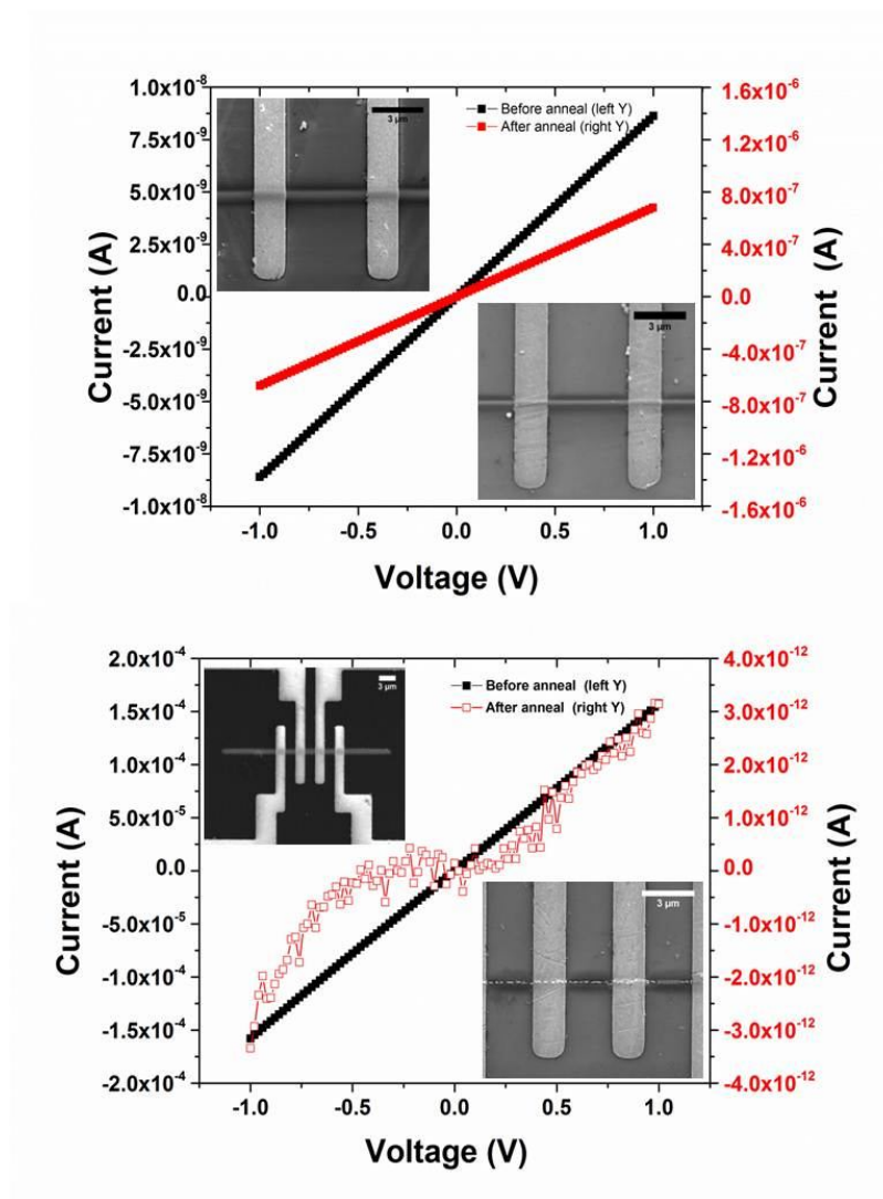
Figure 5.6 I-V measurements of Pt interconnects before and after annealing in forming gas (H 2 /Ar). Right (red) Y axis corresponds to current values after annealing. Top and bottom insets in both show Pt wire before and after annealing respectively. Scale bar for insets is 3 \mu m. (a) I-V curve for standard Pt interconnect before and after annealing under H 2 /Ar for two minutes. (b) I-V curve for liquid Pt interconnect before and after annealing under H 2 /Ar for two minutes.
