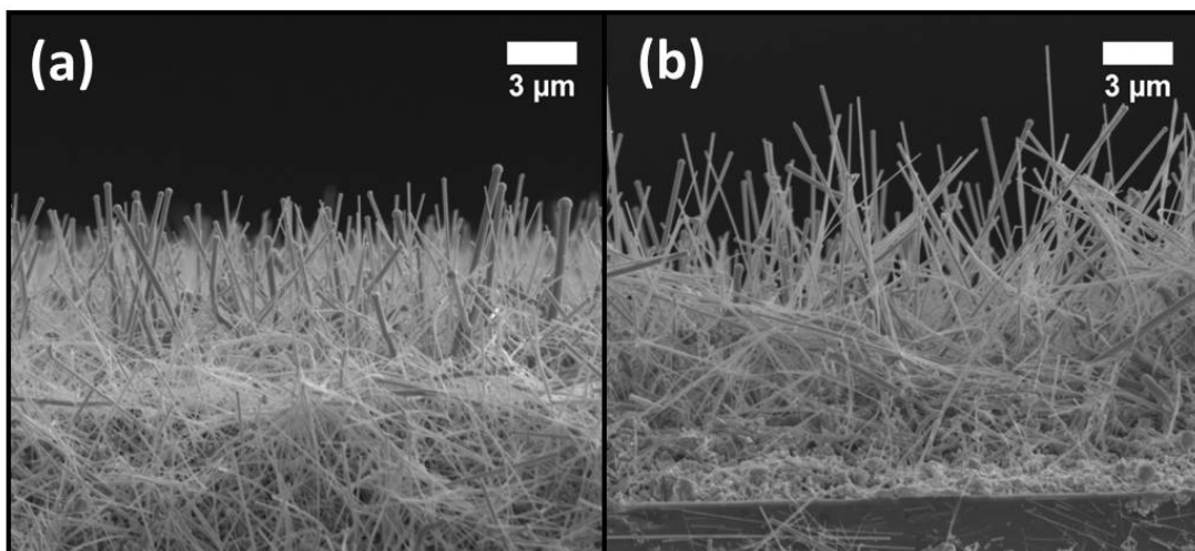
Figure 4.3 SEM images showing Ge nanowire growth at an angle of 90 degrees to the electron beam. (a) SEM image showing Ge nanowires grown on the Au side of a 3-part substrate (shown in figure S1). (b) SEM image showing Ge nanowires grown on the Au/Ag/Ge side of a 3-part substrate.
