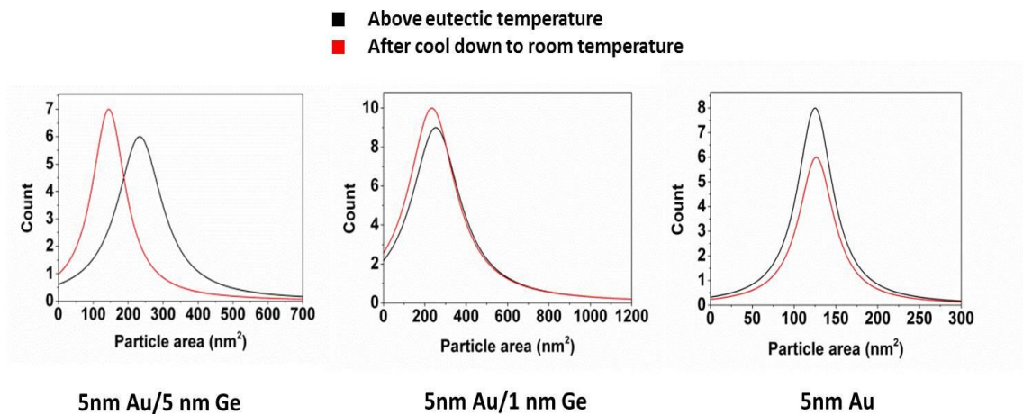
Figure 3.14 Summary of the particle size distributions from part (c) of figure 3.11, figure 3.12 and figure 3.13. As the thickness of the Ge layer decreases from 5 nm to 1 nm to 0 nm (Au film), the difference in particle sizes above the eutectic temperature and at room temperature becomes less significant.
