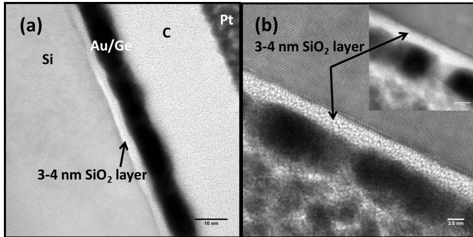
Figure 3.1 Phase-contrast TEM micrographs of a Au/Ge (5 nm/1nm) bi-layer cross-section. While the Ge layer is hard to distinguish due to its thickness, EDX analysis was used to confirm its presence. (a) Au/Ge bi-layer film before annealing. A 3-4 nm SiO 2 layer is clearly visible beneath the Au. (b) Au/Ge bilayer film after annealing at 430 °C for 30 mins. Note that the 3-4 nm SiO 2 layer is still intact, which prevents intermixing of Si and Au.
