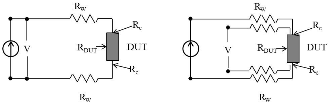
Figure 2.2 2-point (left) and 4-point (right) probe resistance measurements 3 .
