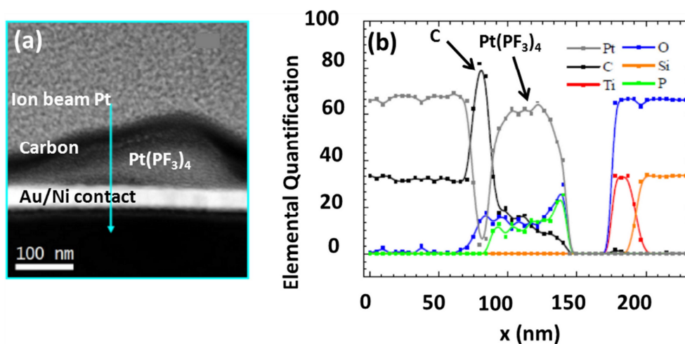
Figure 5.7 Cross-sectional TEM micrograph and EELS analysis of interconnect deposited from Pt(PF 3 ) 4 . (a) Low-resolution cross-sectional TEM micrograph of the interconnect deposited on Au/Ni electrode (b) EELS profile taken along the blue arrow shown in (a).
