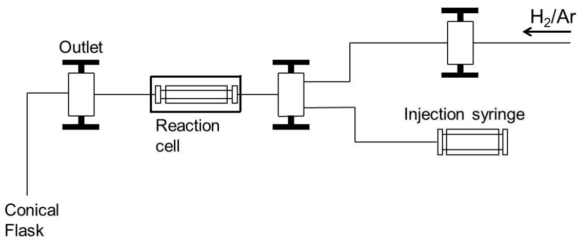
Figure 2.1. Schematic of the liquid-injection chemical vapour deposition set-up used to synthesise germanium nanowires.
