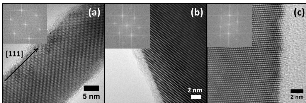
Figure 4.4 TEM images of Ge nanowires grown from a 3-part substrate. (a) A nanowire grown from the Au film. (b) A Ge nanowire grown from the Au/Ag bi-layer and (c) a nanowire grown from the Au/Ag/Ge tri-layer. The images all show monocrystalline Ge nanowires with a [111] growth orientation. Insets are the fast fourier transforms (FFTs) taken of the respective nanowires confirming the growth direction.
