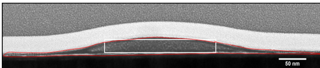
Figure 5.3 Cross-sectional TEM image of a carbon-free interconnect before annealing outlining the nominal area (in white) of the interconnect set to 4000 \text{ nm}^2 and the actual cross-sectional area of the interconnect (in red) that is estimated to be 6000 \text{ nm}^2 . The latter is used to calculate the “true” resistivity of the material instead of the widely used nominal cross-sectional area.
