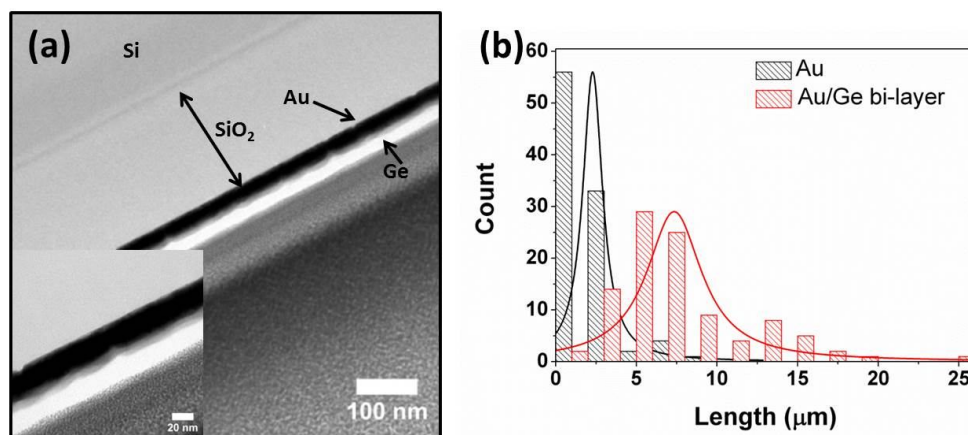
Figure 3.7 (a) TEM micrograph showing a cross-section the Si/SiO 2 substrate that was used to grow GeNWs, as a compliment to the growth already carried out using Si wafers. The 200 nm SiO 2 layer is clearly visible. Inset is higher magnification of the same cross-section, highlighting the Au/Ge bi-layer. (b) Length distribution of GeNWs grown on the Au and Au/Ge bi-layer deposited on the Si/SiO 2 substrate. The distribution clearly shows longer nanowires on the bi-layer side
