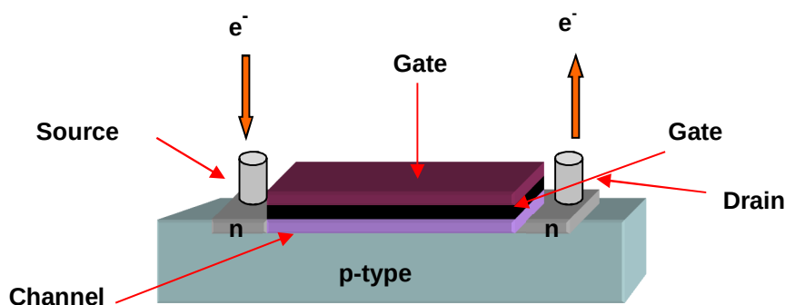
Figure 1.3 Schematic of a MOSFET structure
