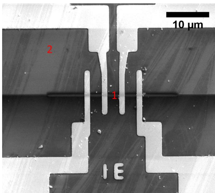
Figure 5.8 SEM micrograph of a carbon-free Pt interconnect deposited on Au/Ni contact pads for EDX analysis. Points 1 and 2 represent the locations of the EDX scans which were taken on both the carbon-free and standard Pt interconnects. Point 1 represents the interconnect while point two is the underlying substrate. The EDX data is given in Table 1 and 2 below.
