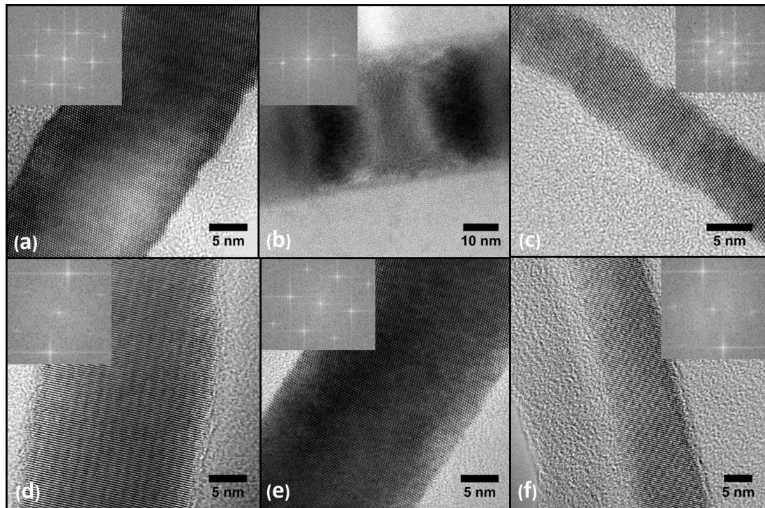
Figure 3.4 TEM micrographs of nanowires grown from the Au/Ge bi-layer side ((a), (b) and (c)) and nanowires grown from the Au film side ((d), (e) and (f)). Insets are fast fourier transforms (FFTs) taken from the lattice resolved image and confirm the common growth orientation of (111).
