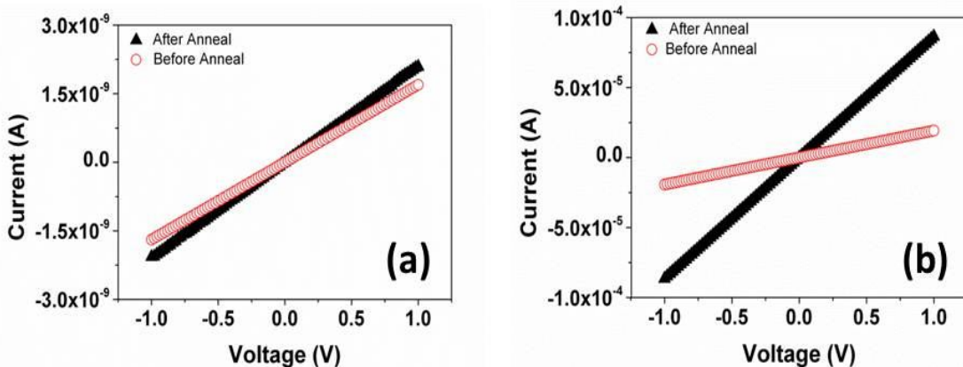
Fig 5.5 I-V measurements of Pt interconnects before and after annealing. (a) I-V curve for a standard Pt interconnect before and after annealing under nitrogen for 1 min. (b) I-V curve for carbon-free Pt interconnect before and after annealing under nitrogen for 1 min.
