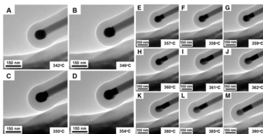
Figure 1.13 TEM images of a Au seed particle melted at 346 °C which migrates into the stem of the nanowire with increasing temperature. Ge recrystallised in the spherical end as the Au/Ge melt shifts into the neck of the nanowire 140 .
