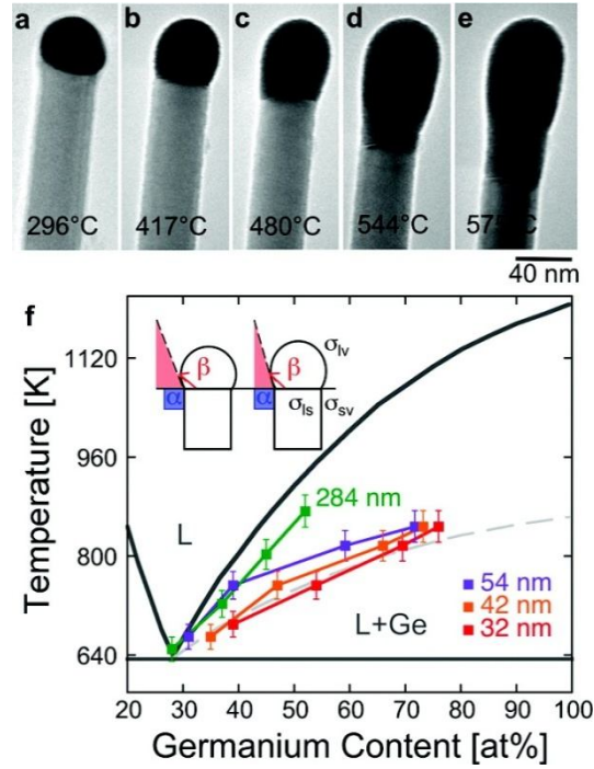
Figure 1.14 (a) to (e) Sequence of TEM images of a Ge nanowire close to the nanowire tip during in-situ annealing experiments at different temperatures; between room temperature and 575 °C. (a) Au–Ge alloy crystalline nanoparticle adjacent to the Ge nanowire before surface melting starts, (b) to (e) exchange of material across the Ge nanowire/liquid drop interface after melting of the alloy Au–Ge nanoparticle and (f) Au–Ge binary alloy phase diagram 138 .
