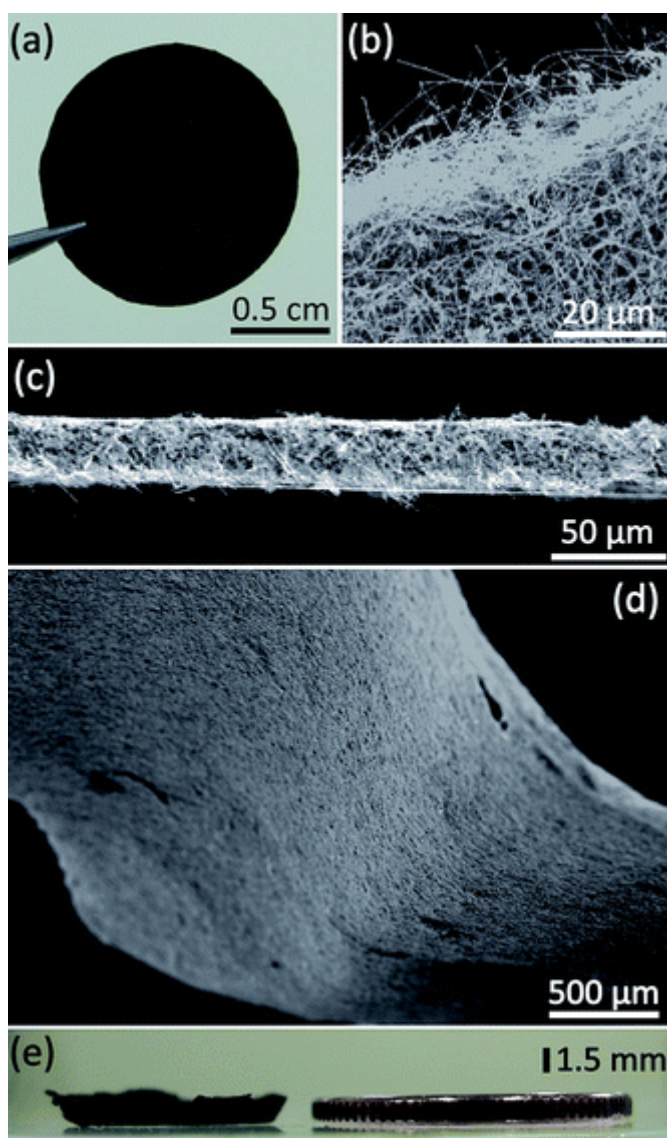
Figure 1.8 (a) Photograph of Ge nanowire fabric (diameter = 13 mm). SEM images of (b) the edge and (c) the cross-sectional area of a 30 \mu\text{m} thick fabric. (d) SEM image of the surface morphology of the Ge nanowire fabric. (e) Photograph of a 1.5 mm thick Ge nanowire fabric 59 .
