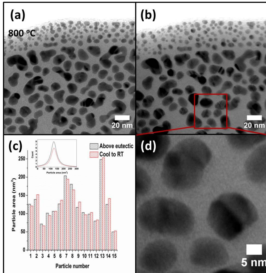
Figure 3.13 TEM analysis of Au alloy particles during in-situ temperature studies of the 5 nm Au film. (a) Low resolution TEM micrograph of the sintered Au islands above the eutectic temperature. (b) Low resolution TEM micrograph of the Au islands shown in part (a) after cooling down to room temperature. (c) Bar chart showing the size differences between 15 particles measured at 800 °C and after cooling to room temperature. Inset shows the Lorentzian curves of histograms plotted from the sizes of the same 15 particles at high temperature and after cooling to room temperature. (d) High resolution TEM micrograph of the area inside the red box in (b).
