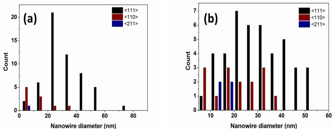
Figure 3.5 Diameter-dependent growth orientation distributions. (a) Distribution of nanowire diameters obtained by TEM on the Au/Ge bi-layer side. Diameters for (111), (110) and (211) are given. (b) Distribution of nanowire diameters obtained by TEM on the Au film side. Diameters for (111), (110) and (211) are given. No significant difference in diameters or growth orientations was observed between the Au film and the Au/Ge bi-layer.
