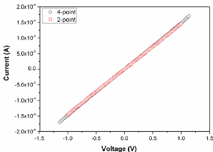
Figure 5.2 2- and 4-point I-V measurements of a liquid Pt precursor which suggest negligible contact resistance due to identical slopes.
