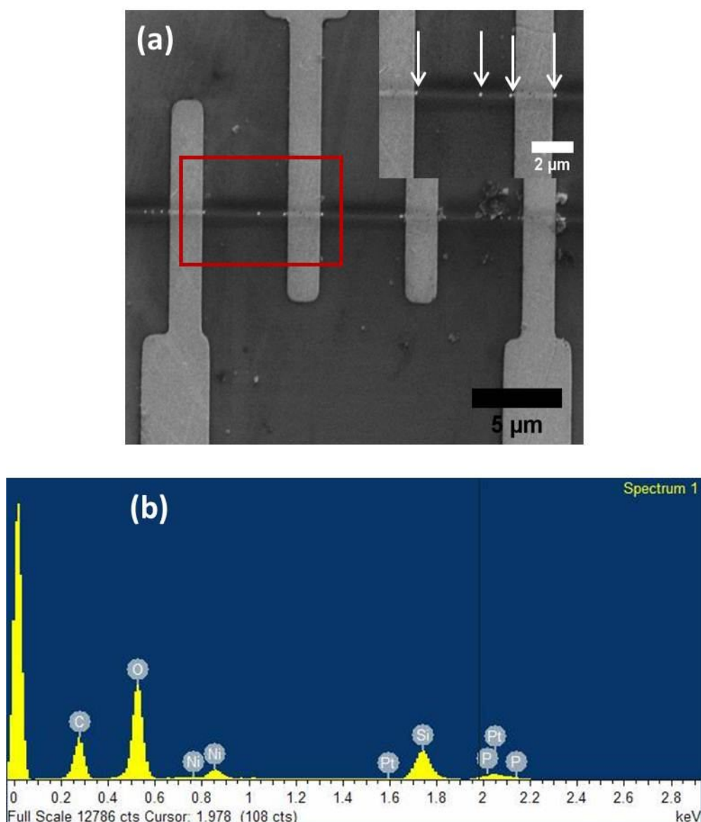
Figure 5.9 (a) SEM micrograph of a carbon-free interconnect deposited on Au/Ni electrodes after additional annealing at 120 °C for 60 minutes under atmospheric conditions. Inset shows the area highlighted in the red box and illustrates the formation of phosphorous clusters (shown by white arrows) along the length of the interconnect. (b) EDX spectrum of the cluster highlighted by the red arrow in (a). The analysis confirms the presence of phosphorous in the clusters. The nickel peaks are from the sample holder in the SEM.
