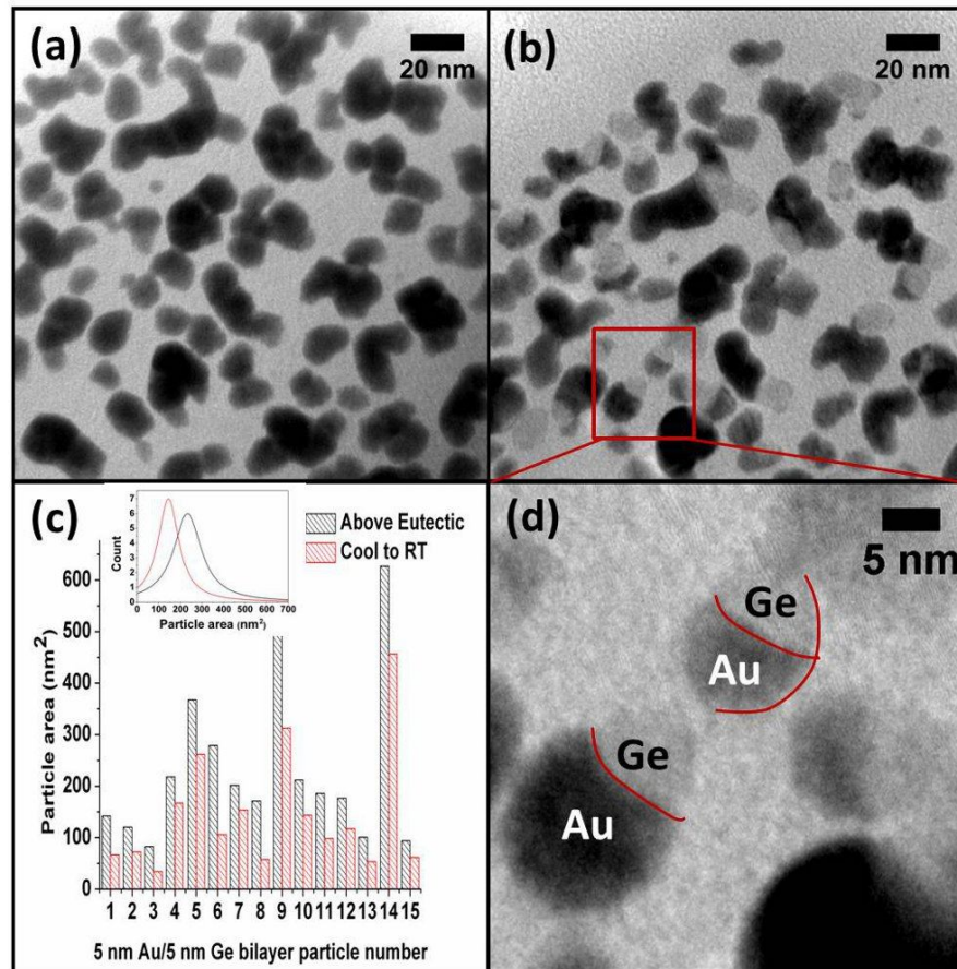
Figure 3.11 TEM analysis of Au/Ge alloy particles during in-situ temperature studies of the 5 nm Au/5nm Ge bilayer film. (a) TEM image of Au/Ge alloy particles above the eutectic temperature. (b) TEM micrograph of the Au/Ge particles shown in part (a) after cooling down to room temperature. (c) Bar chart showing the size differences between 15 particles measures above the eutectic temperature and after cooling to room temperature. Inset shows the Lorentzian curves of histograms plotted from the sizes of the same 15 particles at high temperature and after cooling to room temperature. (d) TEM image of the area inside the red box in (b), highlighting the separation of Ge from Au after cooling to room temperature. Red lines outline the interface between the Au and Ge.
