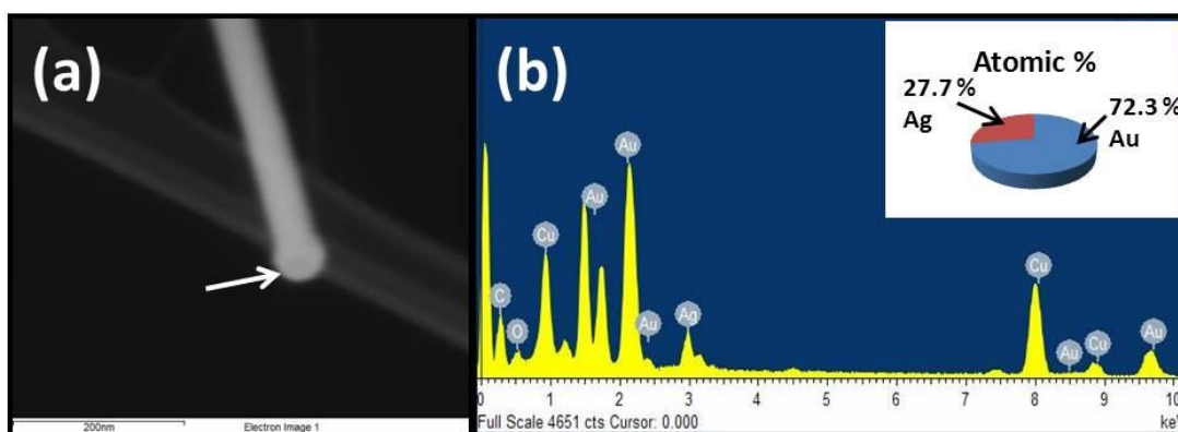
Figure 4.11 STEM analysis of a Ge nanowire grown from a \text{Au}_{0.75}\text{Ag}_{0.25} nanoparticle. (a) Dark field STEM image of a Ge nanowire grown from a \text{Au}_{0.75}\text{Ag}_{0.25} nanoparticle. (b) EDX spectrum of the seed marked by the white arrow in (a). Inset shows the atomic % of Ag and Au in the seed particle on top of the nanowire.
