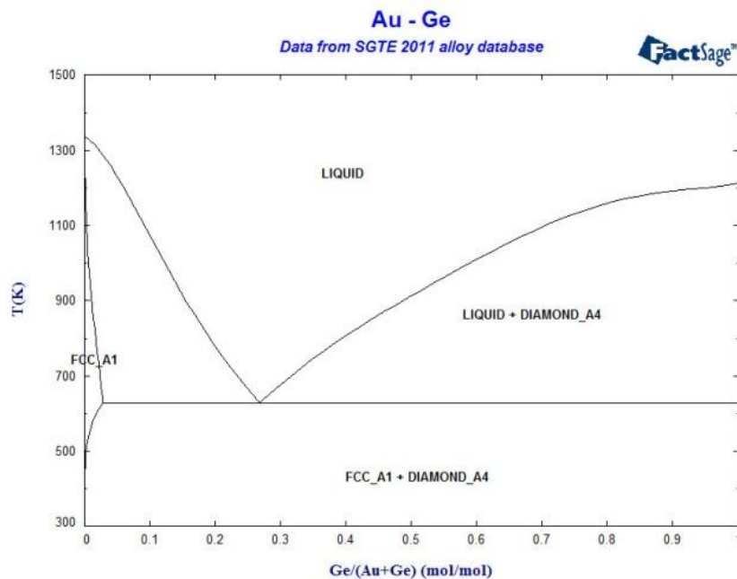
Figure 1.11 Au-Ge binary phase diagram. The diagram is dominated by a single eutectic point at 360 °C with 28 % Ge in Au.
