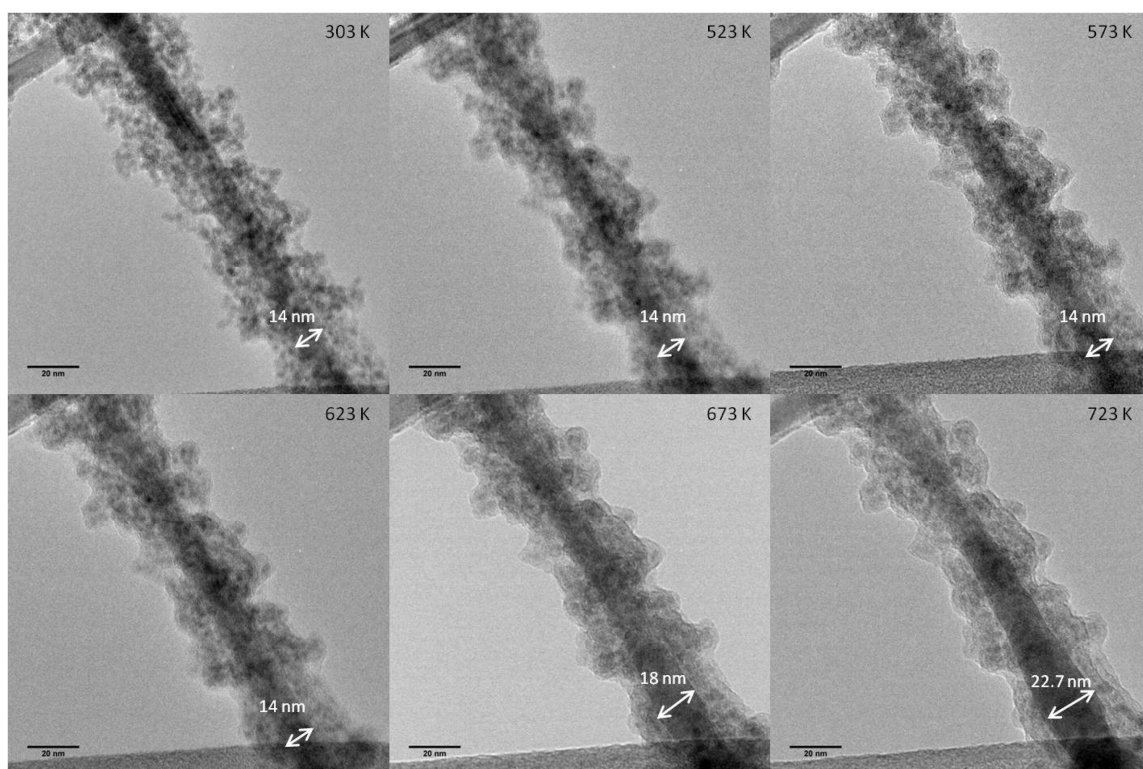
Figure 1.10 Ge nanowire grown using a self-seeded growth mechanism. In situ TEM heating stage experiments showing the Ge nanowire diameter increasing with temperature 78 .
