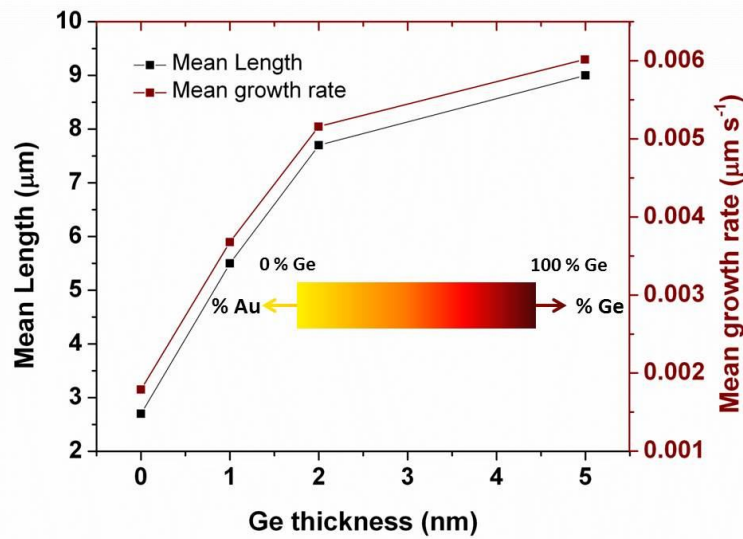
Figure 3.8 Summary of length and growth rate behaviour of nanowires grown from bi-layers of increasing Ge thickness.
