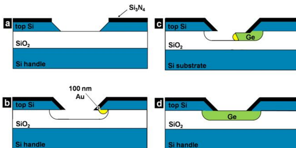
Figure 1.17 Process flow schematic: (a) SOI substrate etched with KOH, (b) selective deposition of Au nanoparticles on the exposed Si surfaces, (c) growth of guided Ge nanowires and (d) bridging Ge nanowires 202 .
