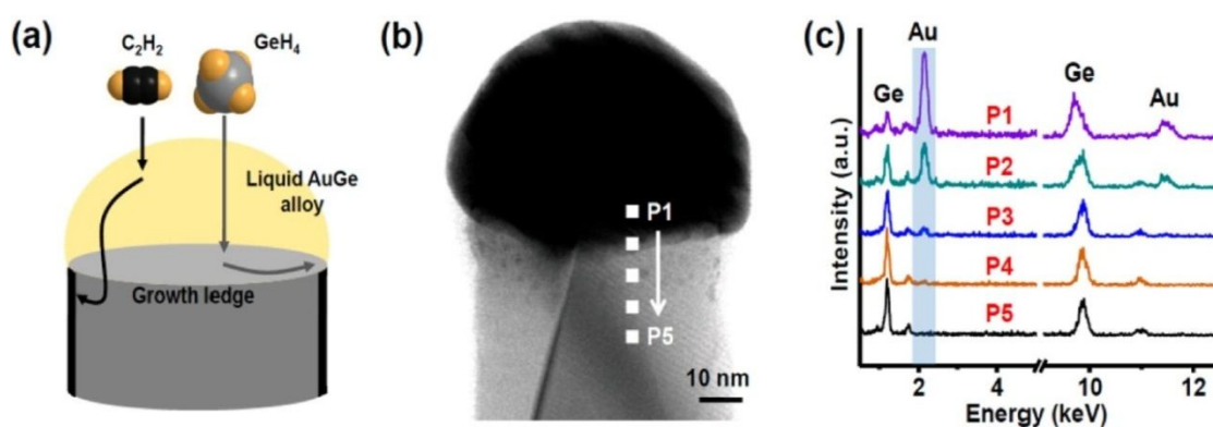
Figure 1.16 (a) Schematic for carbon sheath formation during the Ge nanowire growth process, (b) bright-field STEM image of a single Ge nanowire with a carbon sheath and (c) EDS analysis of the corresponding nanowire from the positions P1 to P5. This data shows that Au diffusion does not occur below the carbon sheath 193 .
