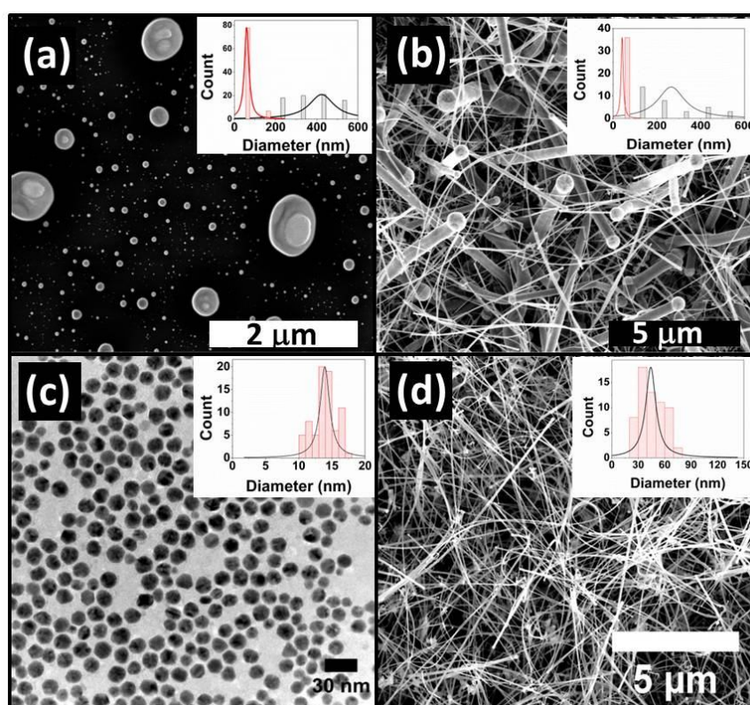
Figure 4.8 Nanowires grown from monodisperse nanoparticles. (a) SEM image of Au/Ag/Ge tri-layer after annealing for 30 min at 465 °C. (b) Ge nanowires grown from the annealed particles shown in (a). A bimodal diameter distribution is present for both the particles and nanowires. (c) TEM image of monodisperse \text{Au}_{0.75}\text{Ag}_{0.25} nanoparticles dispersed on a lacey carbon grid with a mean diameter is 13.9 \pm 1.9 nm. (d) SEM image of Ge nanowires grown from the \text{Au}_{0.75}\text{Ag}_{0.25} nanoparticles shown in (c), with a mean diameter is 44.2 \pm 14 nm. Insets in (a)-(d) are diameter distributions confirming the presence ((a) and (b)) or absence ((c) and (d)) of a bi-modal diameter regime. SEM images in (a), (b) and (d) taken using the SEM backscattered electron detector.
