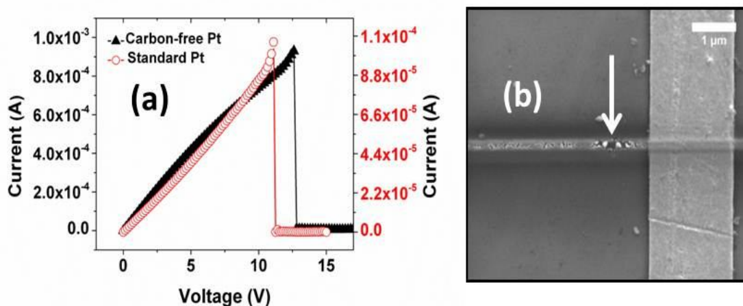
Figure 5.4 Electrical transport measurements performed on carbon-free and standard Pt interconnects. (a) I-V measurements recorded at higher applied voltages for standard Pt (open red circles) and carbon-free Pt (solid black triangles) interconnects. The rapid drop in current around 12 V for both interconnects is due to electrical breakdown of the wire. (b) SEM image showing the point of breakdown of the wire between the two inner electrodes. Scale bar is 1 \mu\text{m} .
