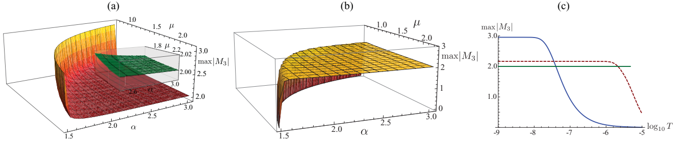
FIG. 2. (Color online) (a) The maximum value of |M_3| as a function of \alpha and \mu at zero temperature. The inset shows that the quasiplateau seen in the main panel is always above the local-realistic bound. (b) The maximum value of |M_3| as a function of \alpha and \mu at temperature T = 10^{-6} K, with \omega_z = 1 MHz. (c) We show the maximum of |M_3| against \log_{10} T for two different working points. The solid line is for (\mu, \alpha) = (1.2, 1.909) while the dashed one is for (\mu, \alpha) = (1.2, 3) . The straight line indicates the boundary imposed by local hidden-variable theories. We have assumed the same value of \omega_z as in panel (b).
