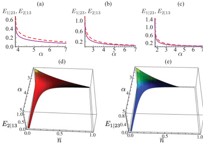
FIG. 3. (Color online) Panels (a), (b), and (c): We show the behavior of E_{1|23} (solid lines) and E_{2|13} (dashed ones) against \alpha for T = 0 and \mu = 0.5, 1 , and 1.5 , respectively. Panels (d) and (e): The same quantities are plotted against \alpha and \bar{n} for \mu = 1 . Qualitatively similar behaviors hold for other values of \mu .
