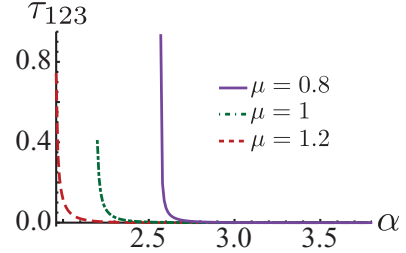
FIG. 4. (Color online) Residual tripartite entanglement in the vibrational state of the transverse modes of our system. We study \tau_{123} against \alpha at T = 0 and for three values of \mu . Each curve is given in a range of parameters such that both stability and the validity of the second-order approach are guaranteed. The residual tripartite entanglement is always finite, with a maximum value that depends on \mu .
