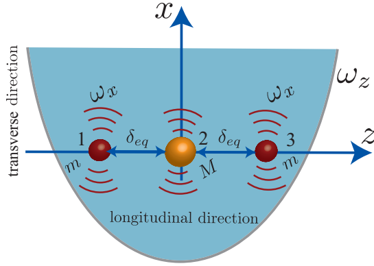
FIG. 1. (Color online) Scheme of the physical system at hand. We consider three ions in a parabolic potential along the longitudinal direction (the trapping potential \omega_z is the same for all the ions). Ions 1 and 3 have the same mass m , while ion 2 (which occupies the position z = 0 in our reference frame) has mass M . The ions are also confined in the transverse direction with the two end-chain ions having trapping frequency \omega_x . The transverse trapping frequency scales inversely with the mass of the ion, so it will be different for the central one. The equilibrium distance between an ion and its nearest neighbor is \delta_{eq} (see text for details).
