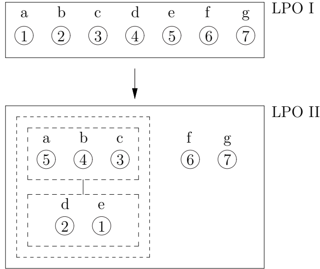
Figure 3.3: LPO I, the MOQA-Java representation of a discrete partial order of size seven, becomes LPO II after the MOQA product function products elements a, b and c above elements d and e
