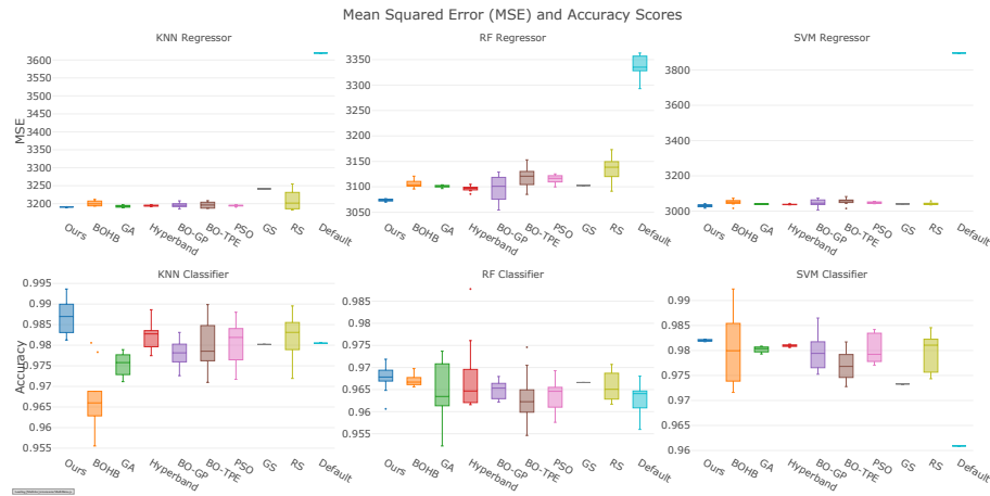
Fig. 3. Comparisons of the accuracy and mean squared errors between ours and the other methods on 2 different data sets with 3 different algorithms over 10 different runs.
