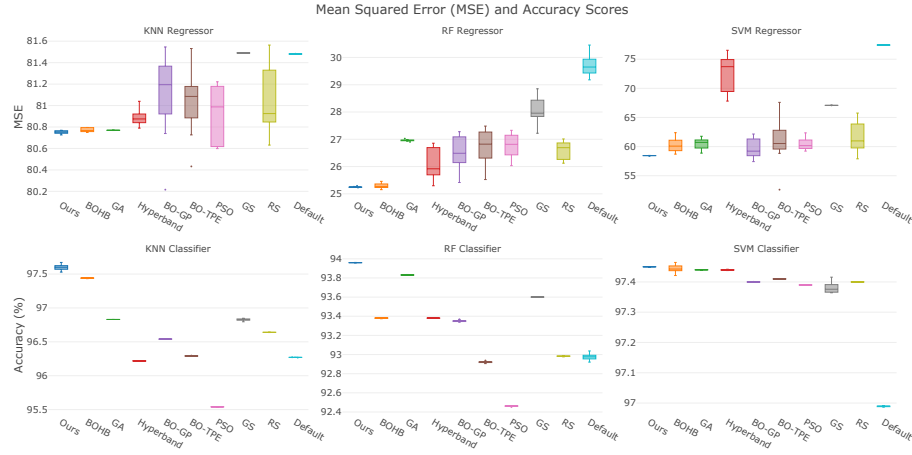
Fig. 2. Comparisons of the accuracy and mean squared errors between ours and the other methods on 2 different data sets with 3 different algorithms over 10 different runs.
