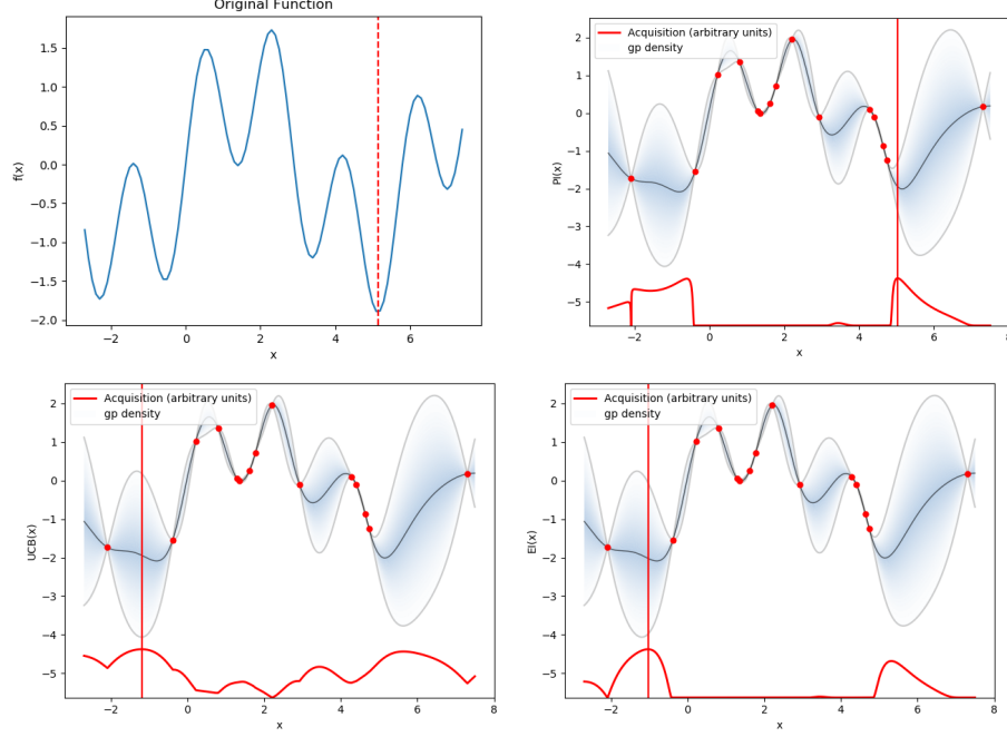
Fig. 1. Illustration of the difference of acquisition function search strategies.
