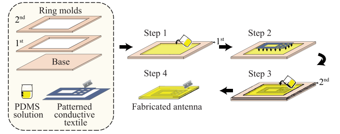
Fig. 8. Schematic illustration of the antenna fabrication process through layer-by-layer PDMS-textile assembly.
