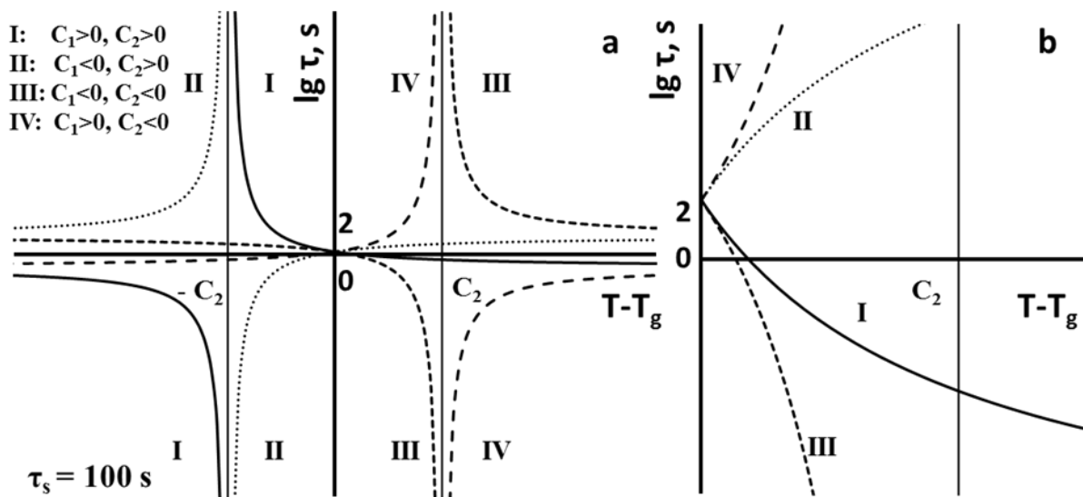
Figure 2.6. Calculated WLF curves with positive and negative values of C_1 and C_2 constants.
