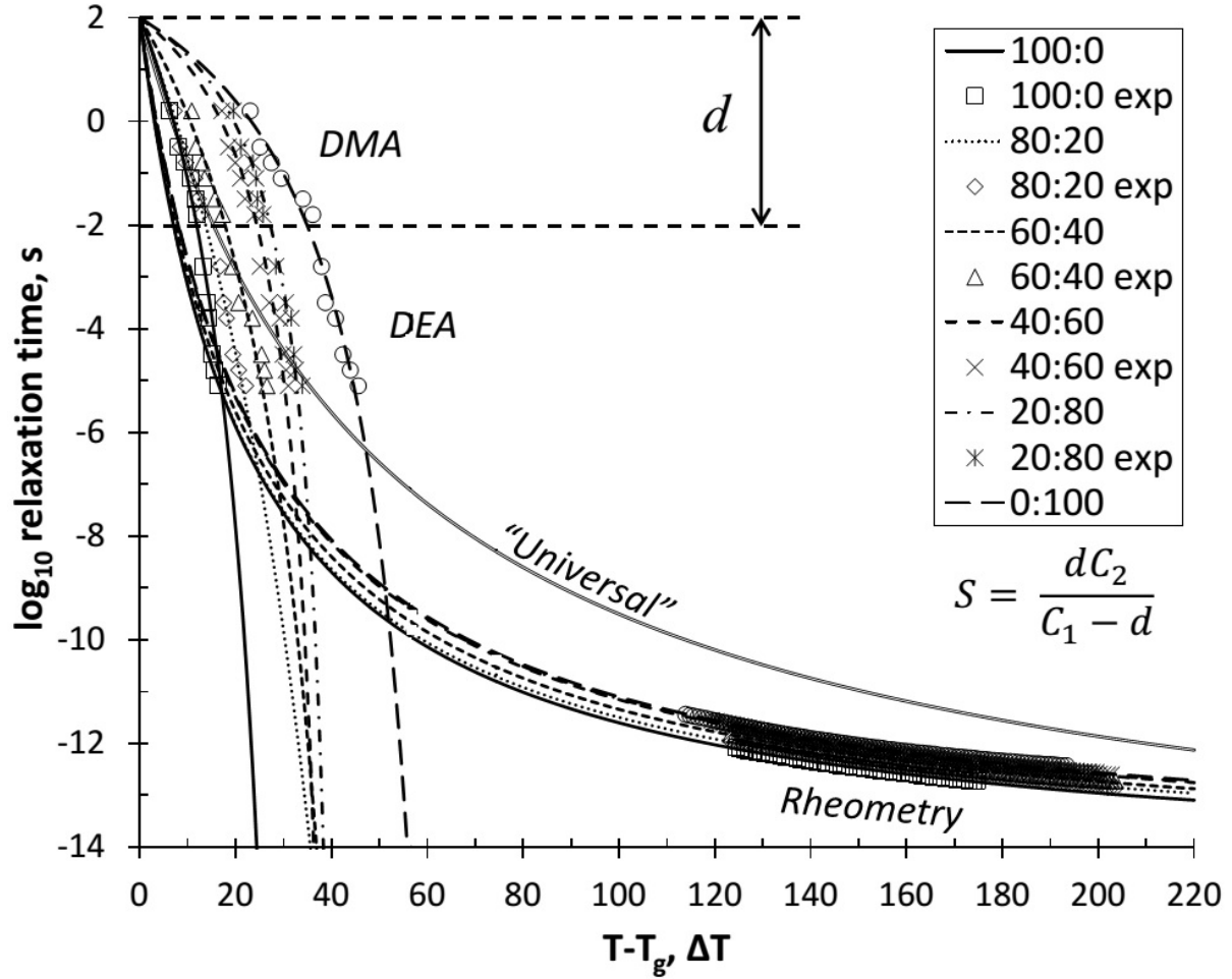
Figure 4.6. Modified WLF curves with calculated and "universal" constants (lines) and experimental data (symbols) for humidified (RH 33%) and high water content (70% of water) trehalose-maltodextrin systems.
