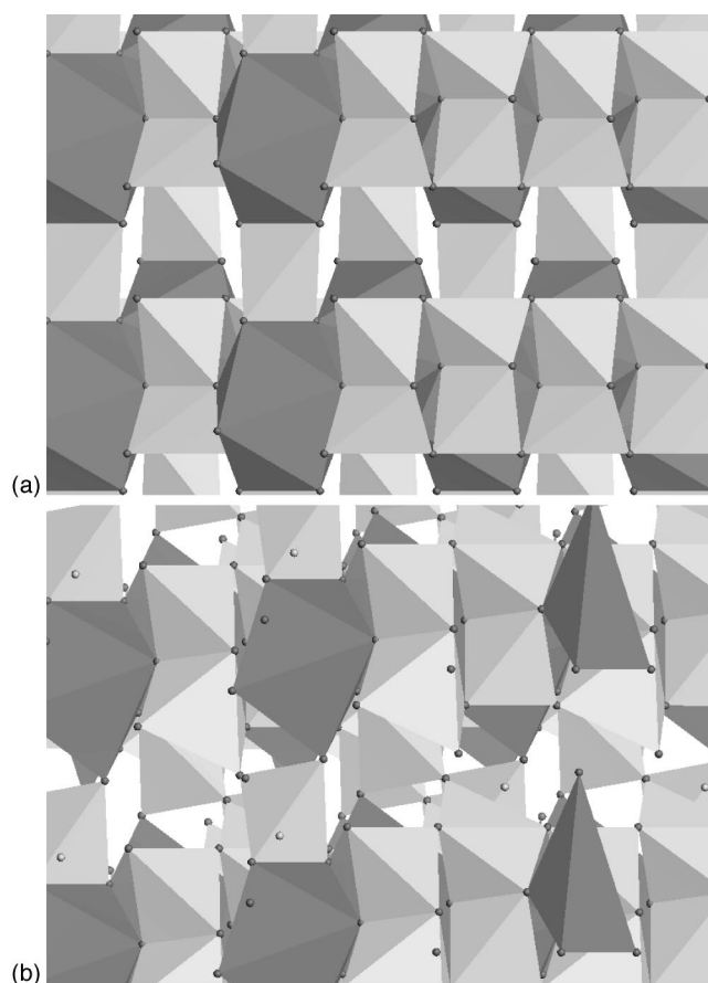
FIG. 6. Polyhedral structure of (a) preanneal \text{Zr}_2\text{Si}_6\text{O}_{16} and \text{Hf}_2\text{Si}_6\text{O}_{16} , and (b) postanneal \text{Zr}_2\text{Si}_6\text{O}_{16} , viewed along [1\ 1\ 0] , with silica polyhedra light gray and \text{MO}_8 dodecahedra or \text{MO}_7 decahedra dark gray. The postanneal configuration of \text{Hf}_2\text{Si}_6\text{O}_{16} is similar to (a). See also Fig. 5. (a) Compared to the ideal configuration of zircon/hafnion in Fig. 2, neighboring silicon tetrahedra are formed within the \text{SiO}_2 -rich regions, breaking the characteristic zircon/hafnion chains along [0\ 0\ 1] . (b) Postanneal, Zr polyhedra show distortion and a drop from eight to seven coordination, which is a motif of a monoclinic crystal structure.
