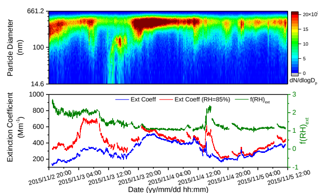
Fig. 7. Upper panel: time series of the aerosol number size distribution of dry PM 1.0 particles measured by SMPS. Lower panel: extinction coefficient of dry PM 1.0 sample, 85% RH humidified sample, and the extinction enhancement factor ( f(\text{RH}) ).
