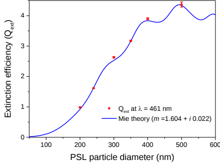
Fig. 5. The extinction efficiency ( Q_{\text{ext}} ) as a function of particle diameter for six different sizes PSL particle at \lambda = 461 nm.
