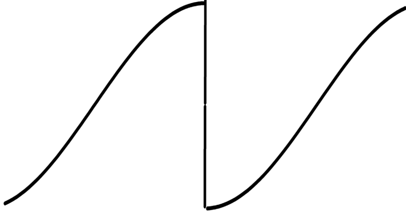
FIGURE 1. The two branches of the solution (2.21) joined with a shock.
