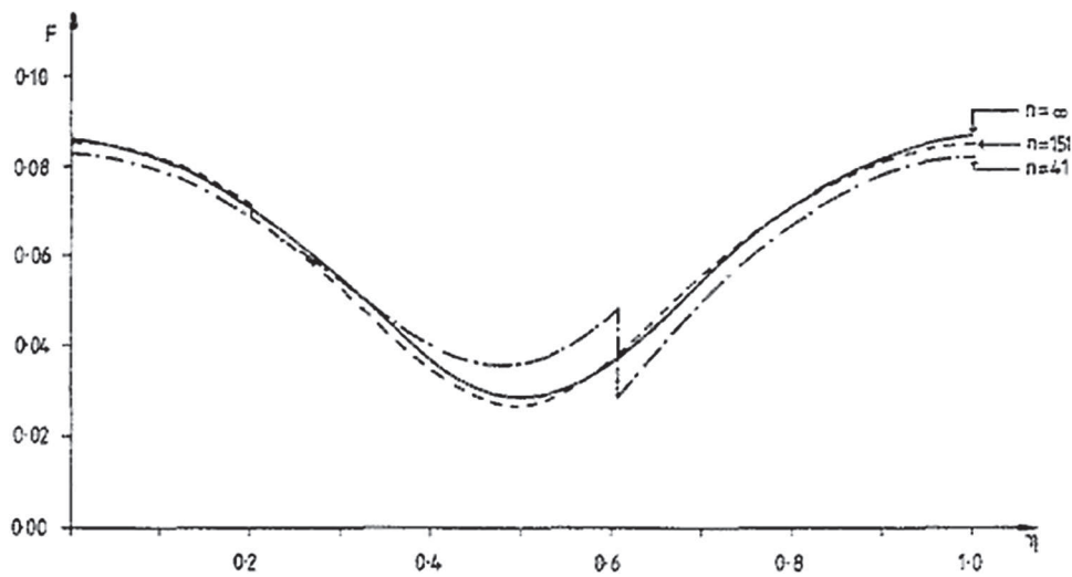
FIGURE 4. Outside resonant band. A = 0.01 , \Delta = 0.06 .
