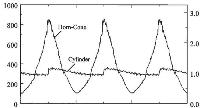
FIGURE 5. Output pressure from cylinder and horn-cone, from [22].
