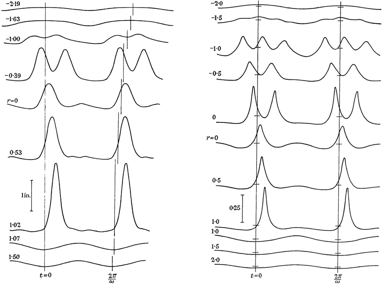
FIGURE 8. Experimental ( left ) and theoretical results ( right ) from [6] and [5].
