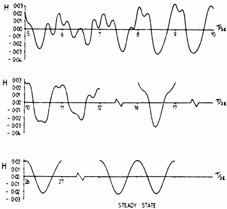
FIGURE 9. Evolution outside resonant band.
