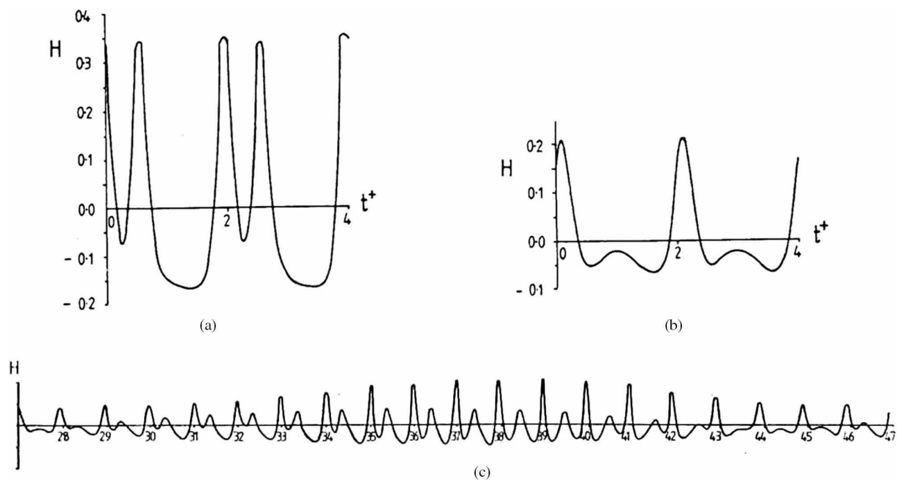
FIGURE 10. (a) and (b) Two solutions at a particular frequency. (c) Beat oscillations.
