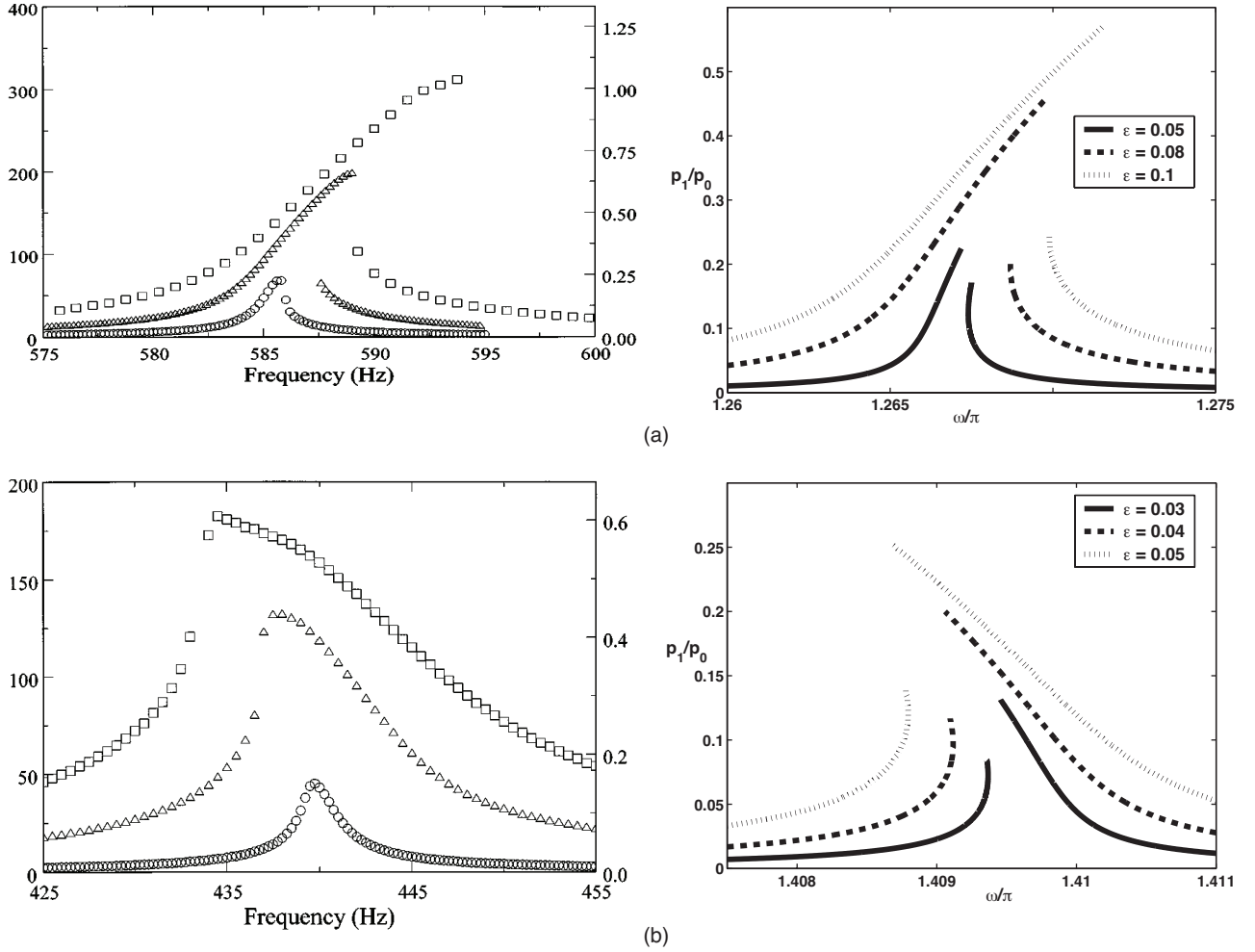
FIGURE 6. Left , Lawrenson experiment from [22]; right , theoretical from [26]. (a) Cone response; (b) bulb response.
