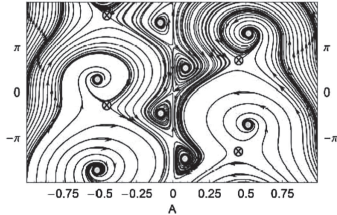
FIGURE 7. Phase plot for cone, \delta = 0.5 .
