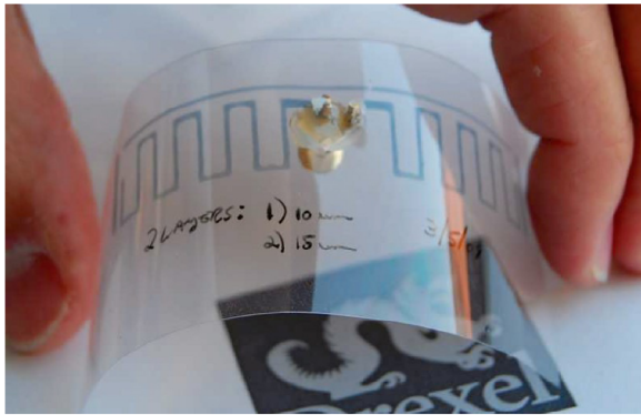
FIGURE 6. RFID Meandering dipole antenna realized with conductive polymer Clevios PH500 PEDOT-PSS. (Reproduced from [36] with permission. Copyright © 2009 IEEE).
