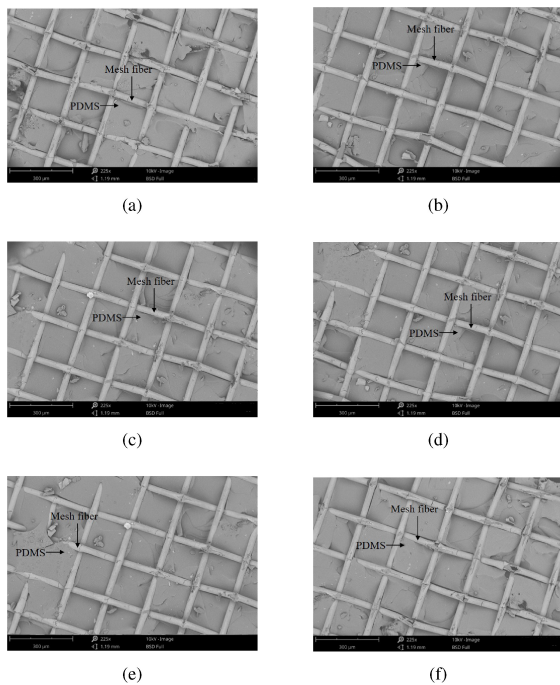
FIGURE 17. SEM images of the composite-(a) no bent, (b) after 10x bending cycle, (c) after 20x bending cycle, (d) after 30x bending cycle, (e) after 40x bending cycle, (f) after 50x bending cycle. (Reproduced from [73] with permission. Copyright © 2020 IOP).
