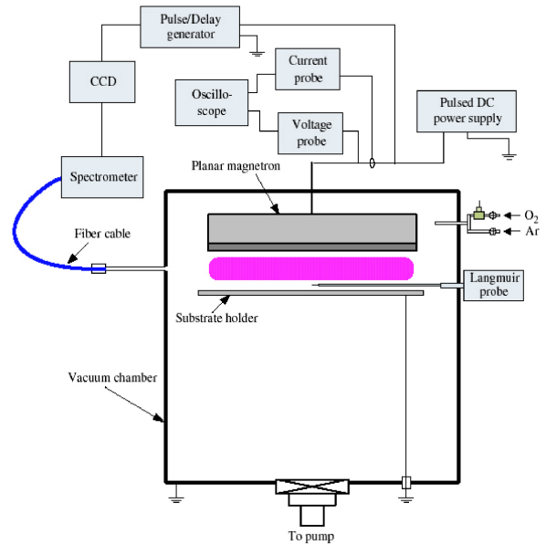
FIGURE 23. Schematic diagram of the mechanism of a pulsed DC magnetron sputtering system. (Reproduced from [92] under a Creative Commons Attribution 4.0 International License (CC BY 4.0)).
