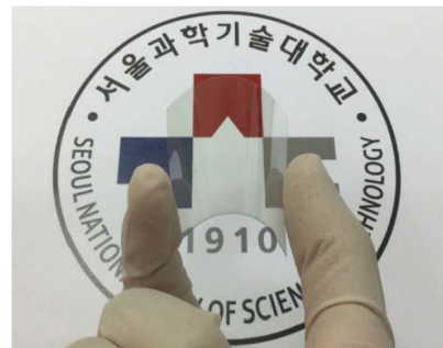
FIGURE 4. Flexible IZTO/Ag/IZTO nanocomposite film. (Reproduced from [11] with permission. Copyright © 2016 IEEE).
