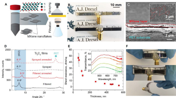
FIGURE 16. Development of Ti_3C_2 MXene antennas. (A) 2D Ti_3C_2 MXene solution. (B) Prototypes of MXene dipole antennas (top antenna is 62-nm-thick and bottom antenna is 1.4-mm-thick). (C) SEM image of the sprayed MXene. Individual Ti_3C_2 flakes are highlighted with red dotted lines. (D) X-ray diffraction (XRD) patterns of MXene films prepared by vacuum-assisted filtration (black solid line) and thermal treatment at 150°C (red solid line). Thermal treatment of the MXene film shifts the (002) MXene peak position from 6.8° to 8.3°. The same comparison was made with the sprayed 1.4-mm-thick MXene film on PET, as-sprayed MXene film (black dashed line), and the film was heated at 150°C (red dashed line). Annealing changed the (002) peak position from 5° to 6.1° and increased its intensity. The peak around 23° is attributed to the PET substrate. (E) Sheet resistance versus thickness of the sprayed MXene films. (F) Sprayed MXene dipole antennas under bending at different curvature radius demonstrating its stability in conformal operations. (Reproduced from [68] under a Creative Commons Attribution 4.0 International License (CC BY 4.0)).
