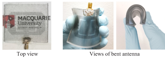
FIGURE 18. Photo of the fabricated prototype of the flexible and transparent dual band antenna developed from VeilShield-PDMS composite. (Reproduced from [70] with permission. Copyright © 2019 IEEE).
