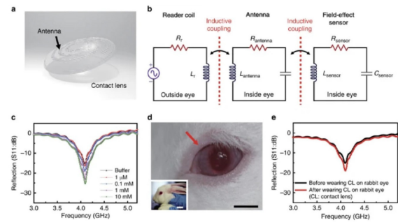
FIGURE 15. (a) Geometry of the transparent glucose sensor on contact lens. (b) Equivalent circuit for wireless sensing on contact lens. (c) Wireless monitoring of glucose concentrations from 1 \mu m to 10 mM. (d) Wireless sensor integrated on the eyes of a live rabbit. (e) Reflection-coefficient results before and after integrating contact lens on an eye of live rabbit. (Reproduced from [7] under a Creative Commons Attribution 4.0 International License (CC BY 4.0)).
