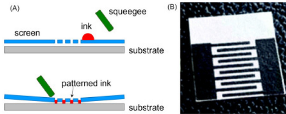
FIGURE 32. Block diagram of screen printing technique. (Reproduced from [46] under a Creative Commons Attribution 4.0 International License (CC BY 4.0)).
