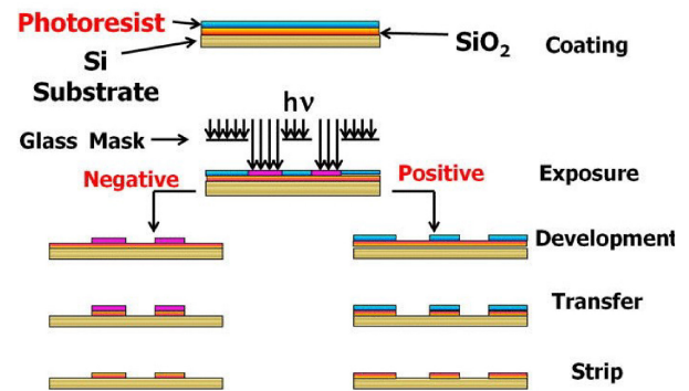
FIGURE 26. Typical photo-lithography process. (Reproduced from [94] with permission. Copyright © 2013 AIP Publishing).
