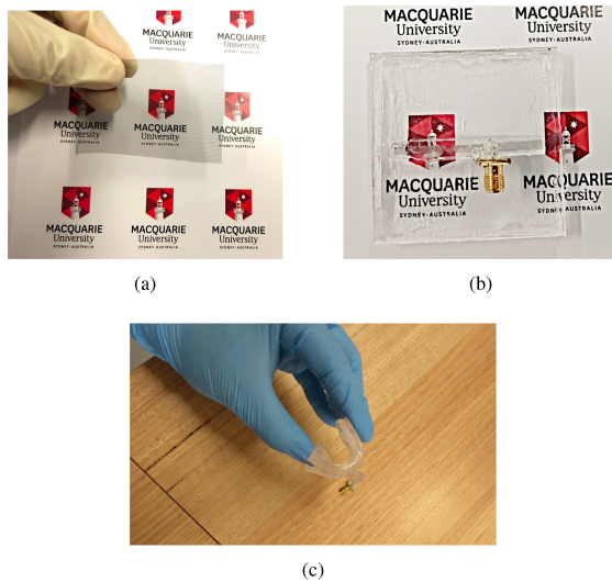
FIGURE 22. (a) A VeilShield sample demonstrating its transparency, (b) The antenna prototype made with VeilShield, PDMS and water, (c) Antenna bent to a very low radius. (Reproduced from [86] with permission. Copyright © 2020 IEEE).
