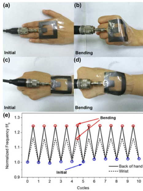
FIGURE 14. Semitransparent and flexible antenna sensor system for human motion detection. (a) Flexible antenna sensor attached to the back of the hand in the unbent (Initial) state, (b) antenna sensor wrapped on hand exhibiting bent state. (c) Antenna sensor on the wrist in unbent (Initial) state. (d) Antenna sensor wrapped on wrist in bent state. (e) Response of normalized frequency in initial and bending states. (Reproduced from [63] with permission. Copyright © 2020 ACS Publications).
