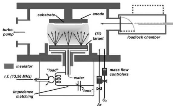
FIGURE 29. Schematic diagram of the RF sputtering deposition method. (Reproduced from [26] with permission. Copyright © 2009 IET).
