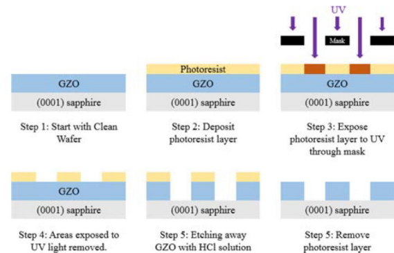
FIGURE 27. Photolithography process for GZO antenna. (Reproduced from [9] with permission. Copyright © 2017 Wiley Periodicals, Inc).
