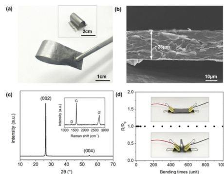
FIGURE 13. Characterization approaches of GAF. (a) Photo of GAF demonstrating high flexibility. (b) Scanning electron microscopy (SEM) image of the cross-sectional view of GAF having a thickness of 28 \mu\text{m} . (c) X-ray diffraction pattern and Raman spectrum of GAF. (d) Testing the mechanical stability of GAF. (Reproduced from [63] with permission. Copyright © 2020 ACS Publications).
