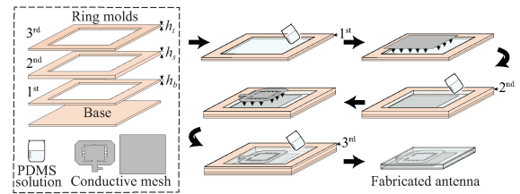
FIGURE 35. Fabrication technique of layer-by-layer polymer-textile assembly technology. (Reproduced from [70] with permission. Copyright © 2019 IEEE).
