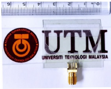
FIGURE 5. Antenna fabricated with AgHT-8 film. (Reproduced from [34] with permission. Copyright © 2015 IEEE).
