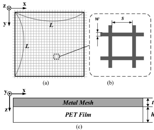
FIGURE 7. Geometry of a Cu-mesh deposited on PET. (Reproduced from [43] with permission. Copyright © 2020 IEEE).
