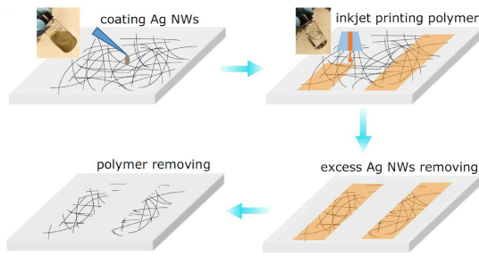
FIGURE 33. Coating and printing method of AgNW. (Reproduced from [89] under a Creative Commons Attribution 4.0 International License (CC BY 4.0)).
