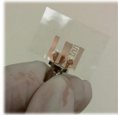
FIGURE 8. Flexible and transparent frequency reconfigurable mesh antenna. (Reproduced from [42] with permission. Copyright © 2017 IEEE).
