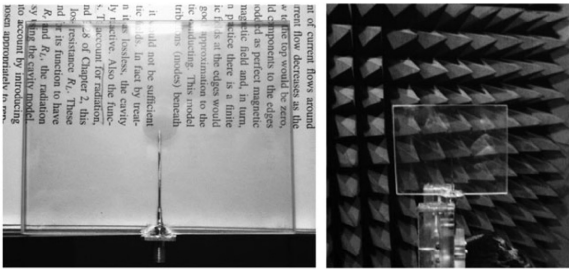
FIGURE 31. Photographs of the fabricated FTO transparent microstrip antenna. (Reproduced from [96] with permission. Copyright © 2015 Taylor & Francis).
