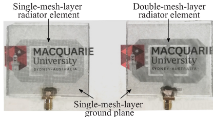
FIGURE 19. Photo of the fabricated prototype of the flexible and transparent dual band antenna developed from double layer VeilShield and PDMS composite. (Reproduced from [70] with permission. Copyright © 2019 IEEE).
