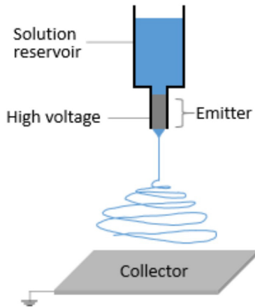
FIGURE 34. Typical electro-spinning process [90]. (Source: www.nanoscience.com).
