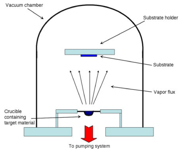
FIGURE 24. Schematic diagram of a typical thermal or electron beam evaporation system. (Reproduced from [91] with permission. Copyright © 2013 Elsevier Inc).
