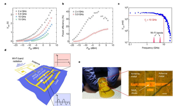
FIGURE 12. An RF energy harvester realized with \text{MoS}_2 based rectenna. (a) Output voltage vs input RF power for the frequencies 2.4 GHz, 5.9 GHz, 10 GHz and 15 GHz. (b) Power efficiency vs input power. (c) Output voltage as a function of frequency of the input signal for the applied RF power P_{RF} = 5\text{ mW} . (d) Prototype of the flexible rectifier. (Reproduced from [49] with permission. Copyright © 2019, The Author(s), under exclusive licence to Springer Nature Limited).
