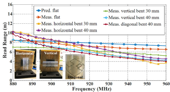
FIGURE 21. Read range of the CP tag antenna in flat state and various bending configurations. The inset shows the bending test set-up. (Reproduced from [72] with permission. Copyright © 2020 IEEE).
