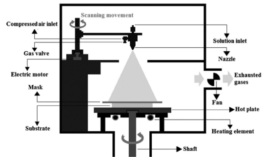
FIGURE 30. Schematic diagram of the spray pyrolysis deposition technique. (Reproduced from [96] with permission. Copyright © 2015 Taylor & Francis).
