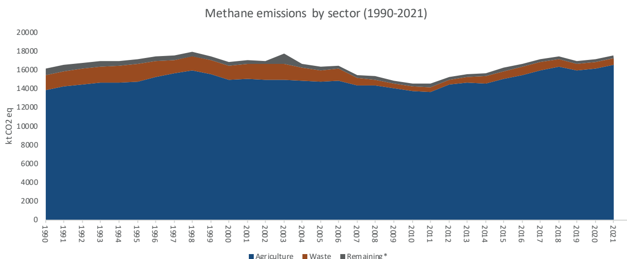
Figure A.11 Ireland's CH 4 emissions by sector from 1990 to 2021. *Very small levels (< 0.5MtCO 2 -eq) in remaining sectors (residential, energy industries, transport, manufacturing combustion and services). Source: EPA (2022f).
