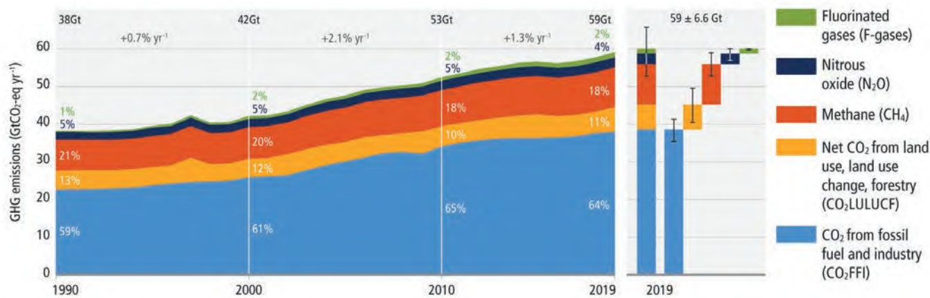
Figure 1.1 Global net anthropogenic greenhouse gas emissions (GtCO 2 -eqyr -1 ) 1990–2019. Source: IPCC (2022b; their figure SPM.1).
