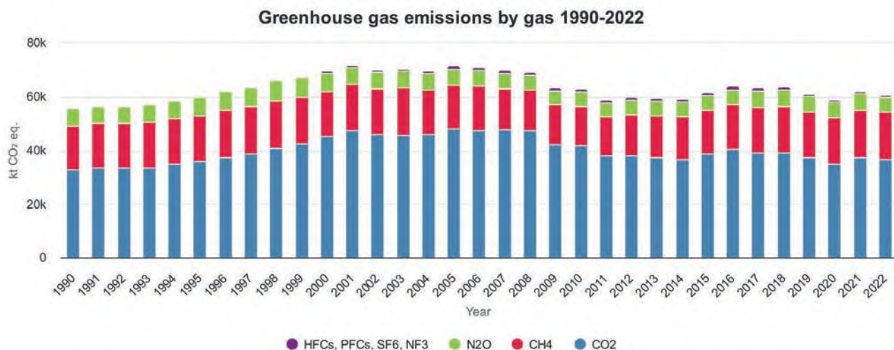
Figure 2.7 Ireland's total GHG emissions per gas (excluding LULUCF) 1990–2021. Source: EPA (2022e).
