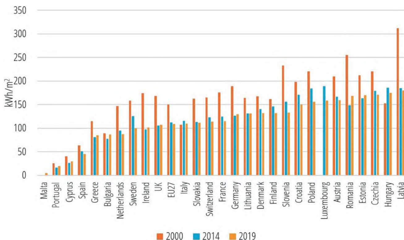
Figure 5.5 Household heating demand ( \text{kWh/m}^2 ) in European countries and the EU. Source: Reproduced with permission from Enerdata (2021).
