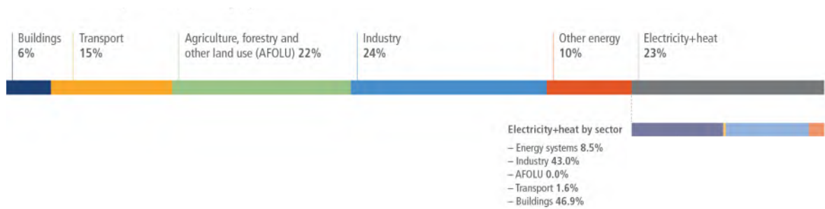
Figure 1.2 Total anthropogenic direct greenhouse gas emissions (59 GtCO 2 -eq) for the year 2019. Source: IPCC (2022b; their figure TS.6, top panel).
