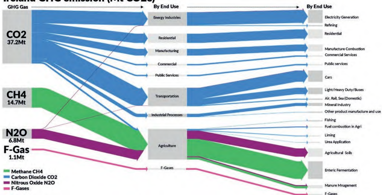
Figure 2.5 Ireland's GHG emissions (MtCO 2 -eq) in 2019 by sector and end use; based on EPA (2021a).
