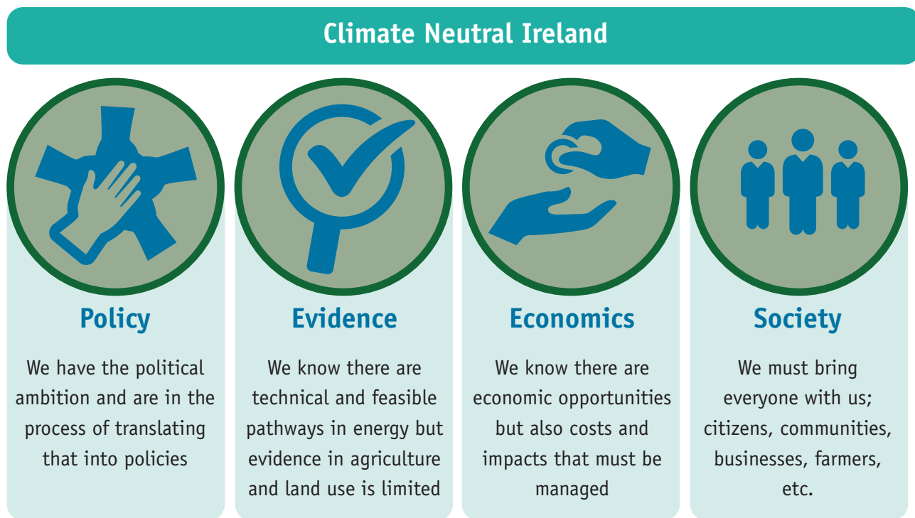
Figure SPM.1 Ireland's strategy towards climate neutrality 1 .
