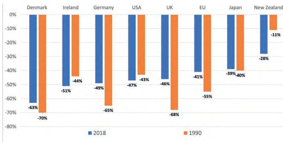
Figure 2.1 Comparison of EU and different country 2030 emission reduction targets relative to 1990 and 2018. Source: Authors.
