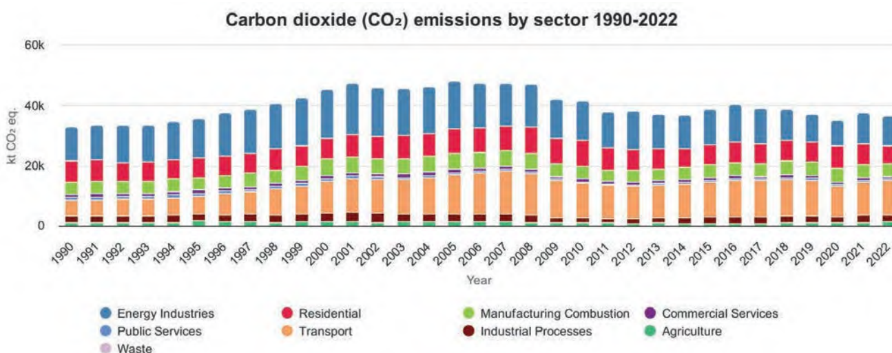
Figure 2.8 Ireland's total GHG emissions per sector (excluding LULUCF) 1990–2020. Source: EPA (2022e).
