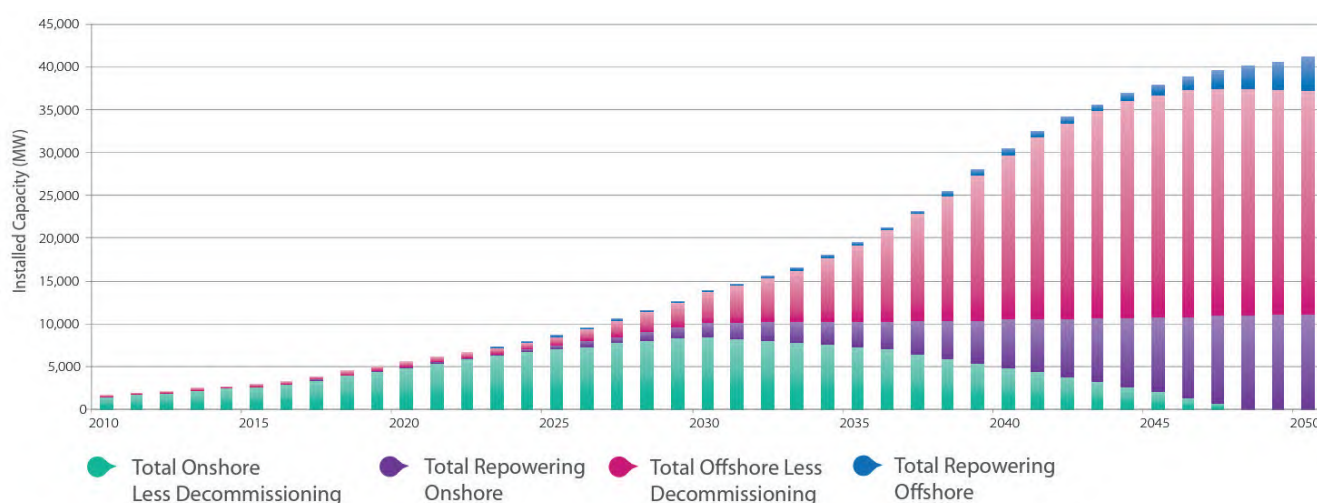
Figure 4.1 Cumulative capacity with repowering of onshore and offshore wind energy. Source: SEAI (2011b).
