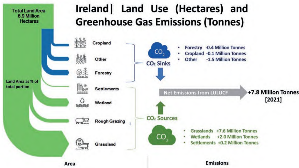
Figure 6.6 Land use and GHG emissions generated from the LULUCF sector in 2021.
