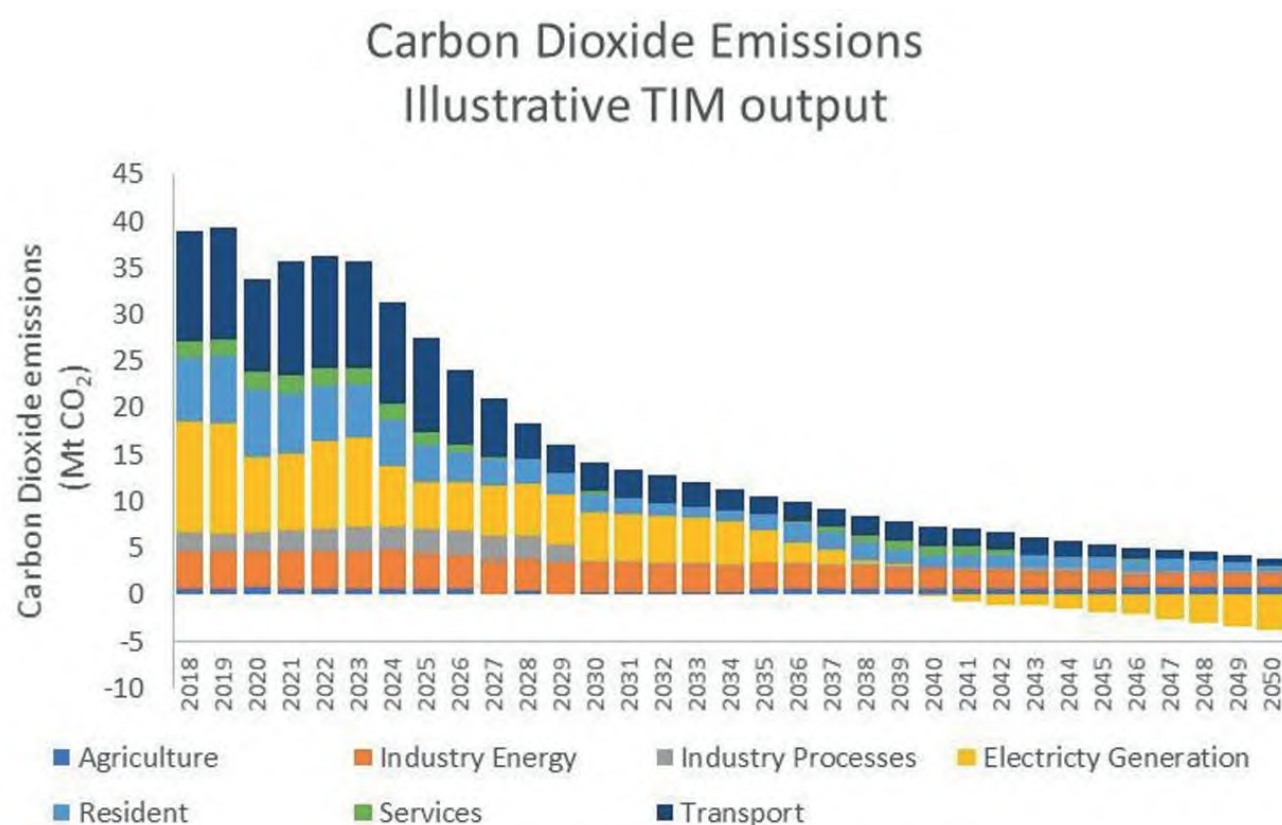
Figure A.5 Example of an emissions reduction and removals deployment pathway for 2018–2050 from the Times Ireland model. Source: Climate Change Advisory Council (2021).
