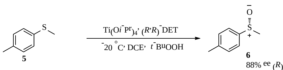
Scheme 2 Modena Oxidation
