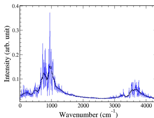
Fig. 6 Power spectrum of calculated proton diffusion in the fully relaxed BaZrO 3 bulk. The spectrum was obtained by Fourier transform of the velocity–velocity correlation function. The high wave number peak is consistent with that of the O–H bond in water at around 3600 \text{cm}^{-1} , while the peak at low wave number resembles that measured by Karlsson et al in similar systems [28]
