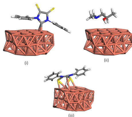
Fig. 4 (i) shows the S-NHC carbene chemisorbed onto the bare copper surface via C. (ii) shows the acacH ligand physisorbed onto the surface. (iii) shows the (S-NHC)CuH adsorbed onto the surface via Cu and S.
