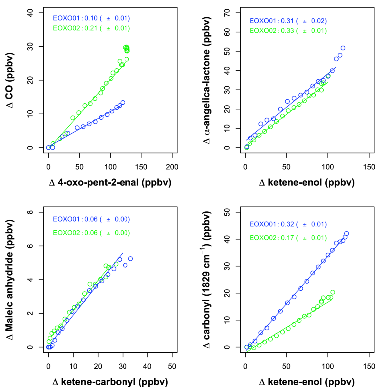
Figure S9 Rate of change (ppbv) of products plotted against reactant for the (E)-4-oxo-2-pentenal experiments. CO is assumed to be a primary photolysis product. 5-methyl-2(3H)-furanone and the unidentified carbonyl at 1829 \text{cm}^{-1} are assumed to come from the ketene-enol, and maleic anhydride is assumed to come from the ketene-carbonyl.
