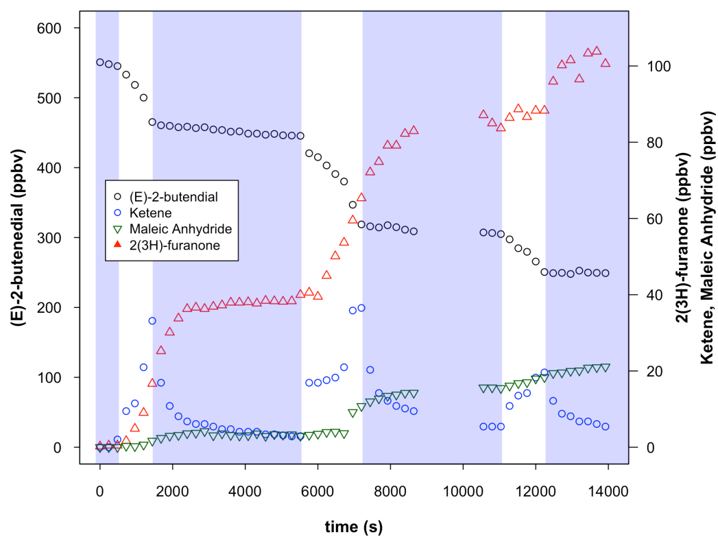
Figure S10 Experiment EBT03. The chamber was opened (white space) and closed (blue space) several times.
