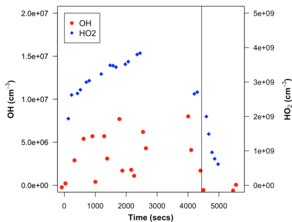
Figure S6 OH (red circles, left axis) and HO 2 (blue diamonds, right axis) concentrations measured by LIF-FAGE during experiment EBUT05. Chamber open at t = 0 s, chamber closed at vertical line; t = 4440 s.
