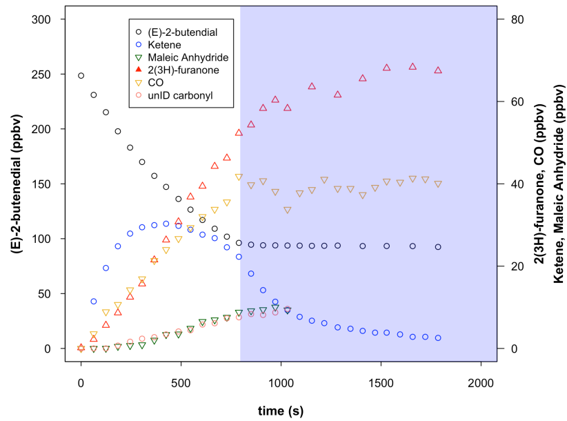
Figure S12 Experiment EBUT04. The chamber was closed at t = 780 s (blue space).
