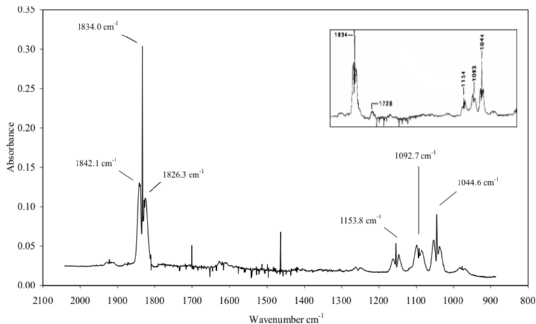
Figure S2 Gas-phase FTIR spectrum of 2(3H)-furanone. Inset: Corresponding spectrum reported by Bierbach et al. 4 .
