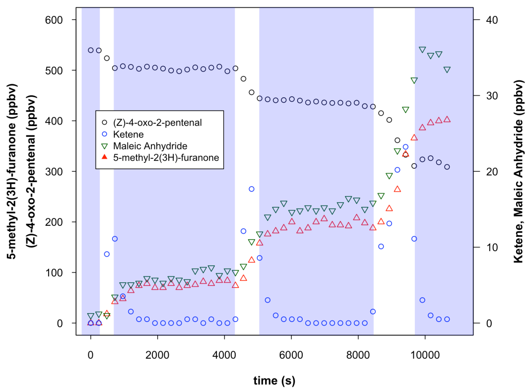
Figure S11 Experiment ZOZO03. The chamber was opened (white space) and closed (blue space) several times.
