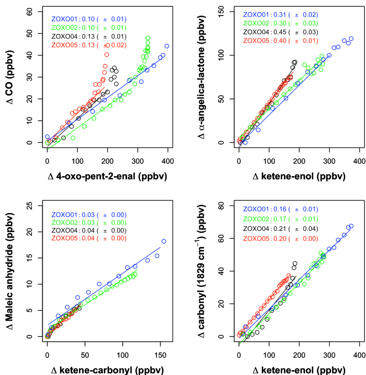
Figure S8 Rate of change (ppbv) of products plotted against reactant for the (Z)-4-oxo-2-pentenal experiments. CO is assumed to be a primary photolysis product. 5-methyl-2(3H)-furanone and the unidentified carbonyl at 1829 \text{cm}^{-1} are assumed to come from the ketene-enol, and maleic anhydride is assumed to come from the ketene-carbonyl.
