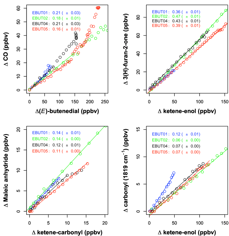
Figure S7 Rate of change (ppbv) of products plotted against reactant for the (E)-2-butenedial experiments. CO is assumed to be a primary photolysis product. 2(3H)-furanone and the unidentified carbonyl at 1819 cm -1 are assumed to come from the ketene-enol, and maleic anhydride is assumed to come from the ketene-carbonyl.
