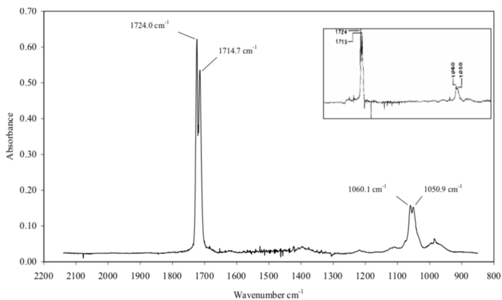
Figure S5 Gas-phase FTIR spectrum of synthesized (E)-2-butendial. Inset: Corresponding spectrum reported by Bierbach et al. 4 .
