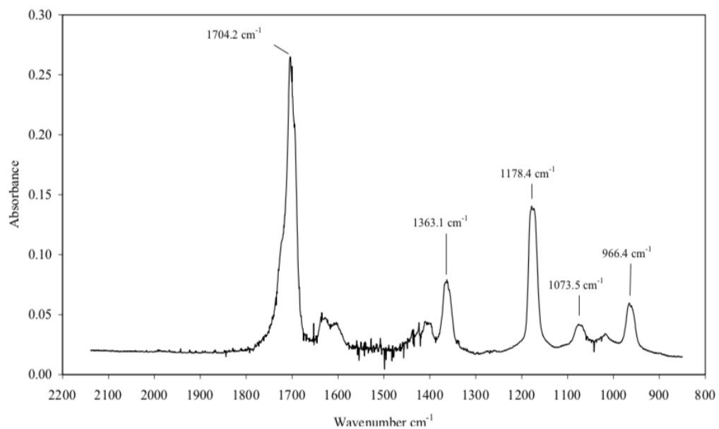
Figure S4 Gas-phase FTIR spectrum of synthesized (Z)-4-oxo-2-pentenal.
