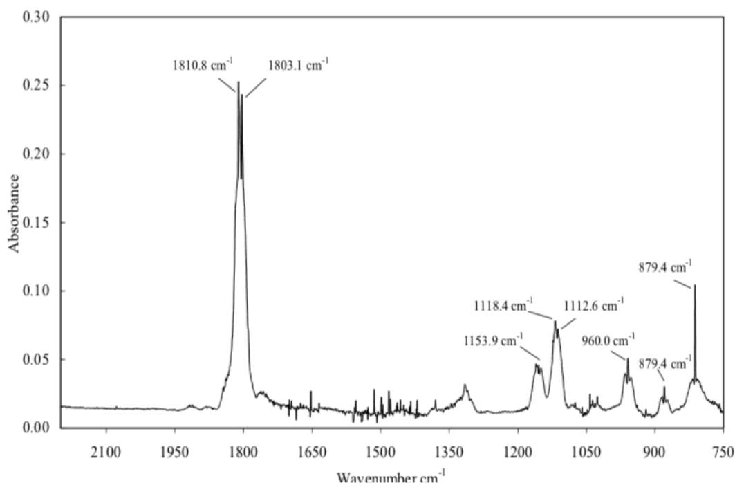
Figure S1 Gas-phase FTIR spectrum of 5-methyl-2(5H)-furanone ( \beta -angelicalactone).
