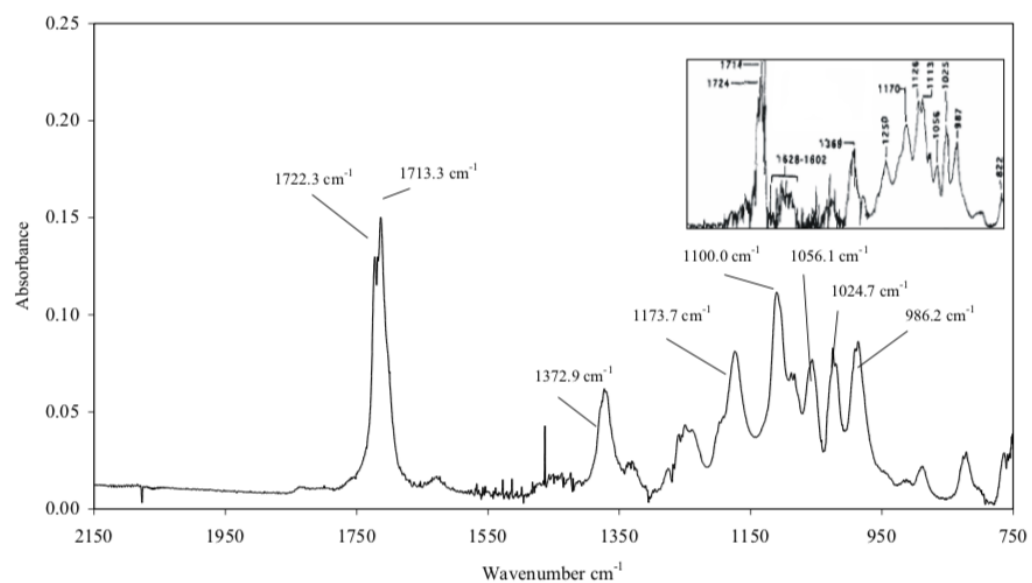
Figure S3 Gas-phase FTIR spectrum of synthesized ( E )-4-oxo-2-pentenal. Inset: Spectrum of ( Z )-4-oxo-2-pentenal reported by Bierbach et al. 4 .
