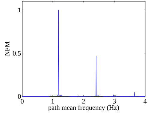
(f) Whitened Seizure ( \text{NFM}_{0.3} )
