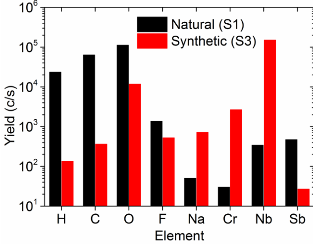
Figure 3: SIMS raw yields of impurities in natural MoS 2 (S1) and in synthetically-grown Nb-doped MoS 2 (S3). H, C, O, F and Sb were collected as negative ions while sputtering with a Cs + beam. Na, Cr and Nb were collected as positive ions while sputtering with a O 2 + beam. No direct same-sample yield comparisons are given, only between different samples.
