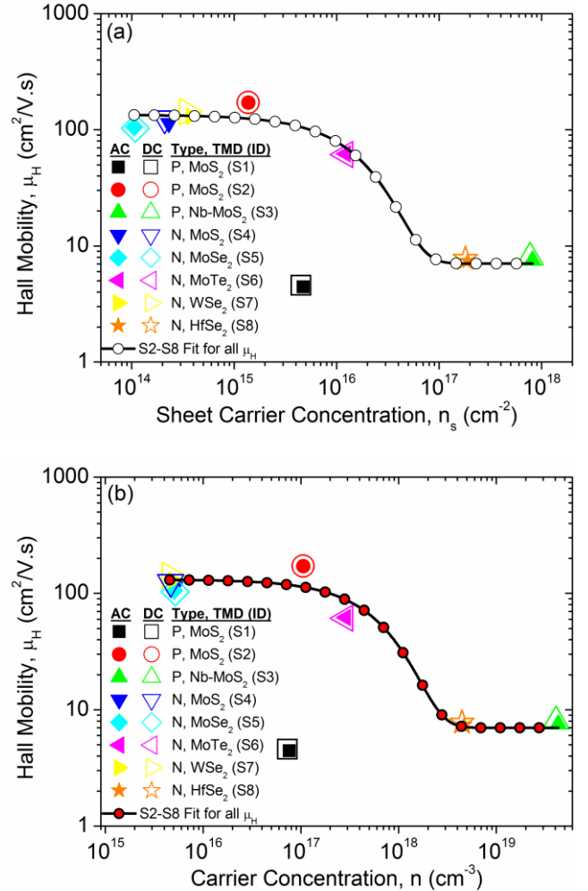
Figure 2: DC-AC Hall mobility versus (a) sheet carrier concentration and (b) carrier concentration. Best non-linear curve fit lines to crystals S2-S8 ( S1 is excluded from the best fit exercise as it is abnormally too resistive). Note that the y-axes of the log-log plots (a) and (b) have the same Hall mobility scale to assist in comparing behavior.
