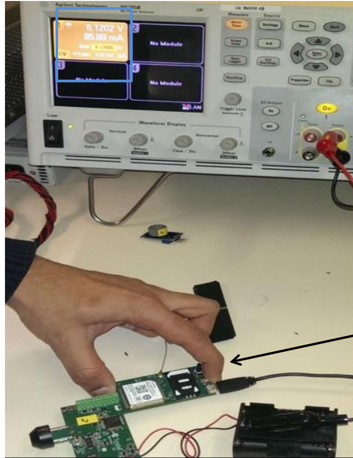
Figure 12. Power Testing Setup.
